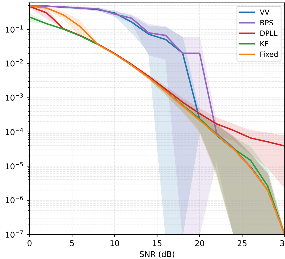
Weak Turbulence
