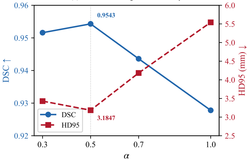
(a) Inter-CBL weight \alpha sensitivity
