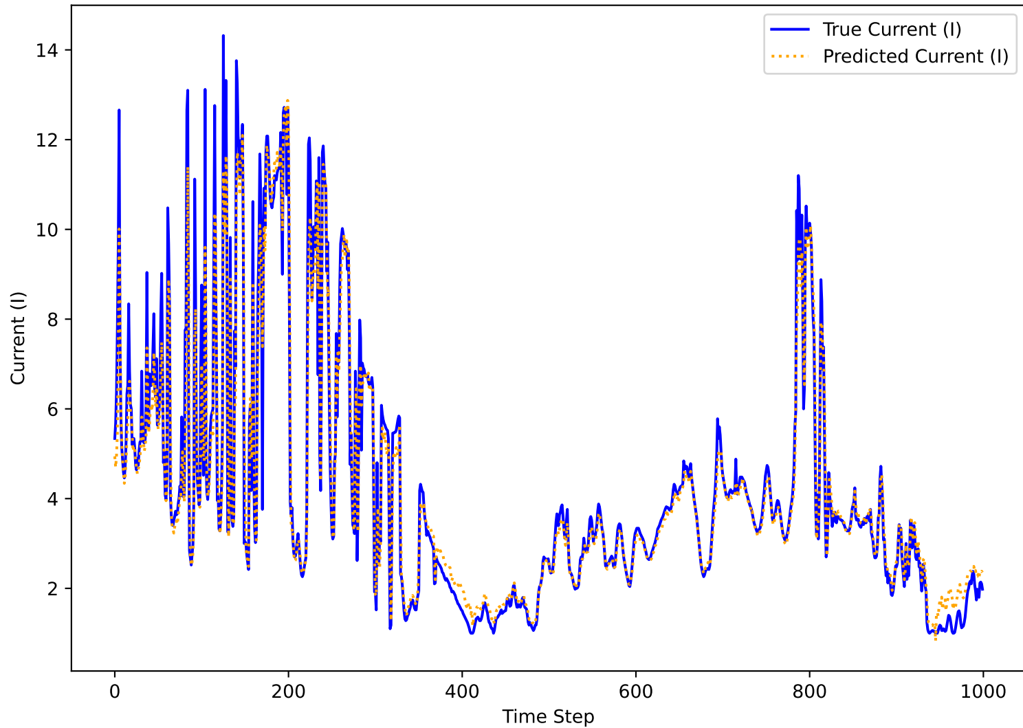
CNN_LSTM - Current (I) Time Series
