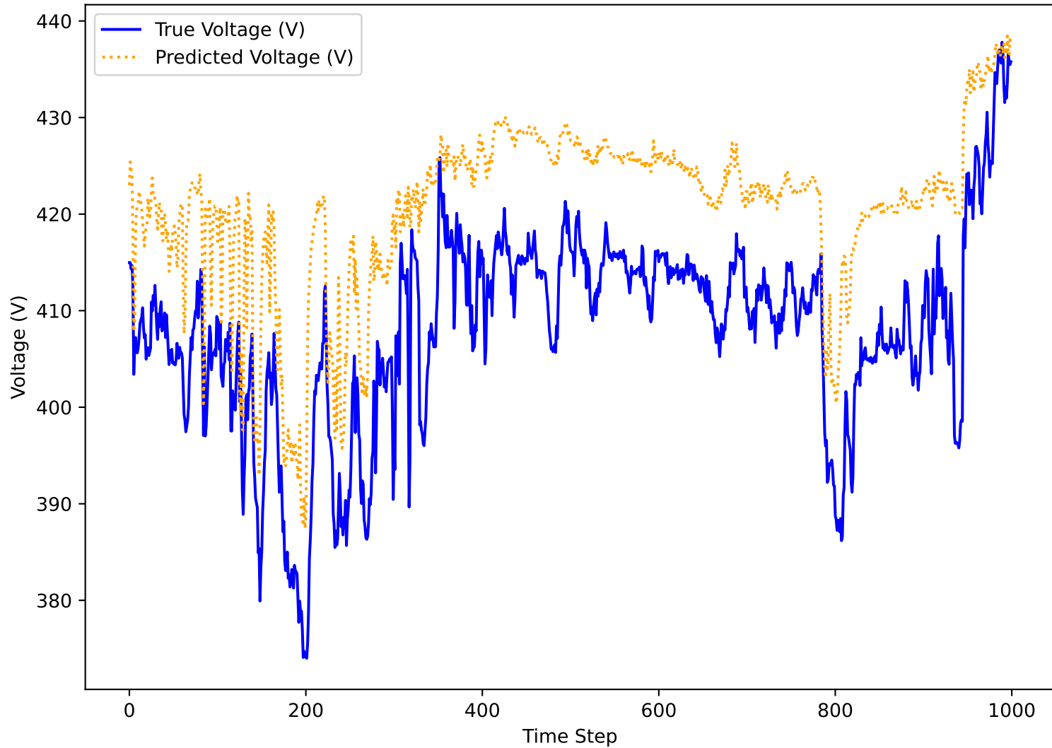
CNN_LSTM - Voltage (V) Time Series
