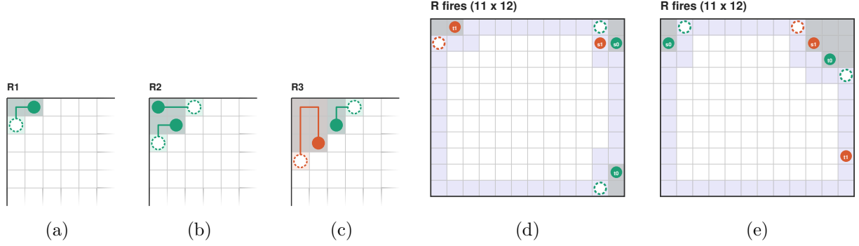
Figure 4: The R entry. (a)–(c) Rules R1–R3 at the top-left corner of the grid, which continues to the right and below. Green is a colour \gamma and orange the other colour \bar{\gamma} . The forced path pieces are drawn, settled cells are grey, and dashed circles are the effective endpoints. (d), (e) Two 11 \times 12 instances on which R fires and no other entry does. Neither has a solution. After the forced routes, the four effective endpoints lie on the border of the remaining region (shaded purple) and alternate in colour along it. This is the T1 condition for that region, so the two paths would have to cross. In (d) rule R1 applies at three corners, and in (e) rule R3 settles eight cells at the top-right corner and R1 settles two at the top-left.
