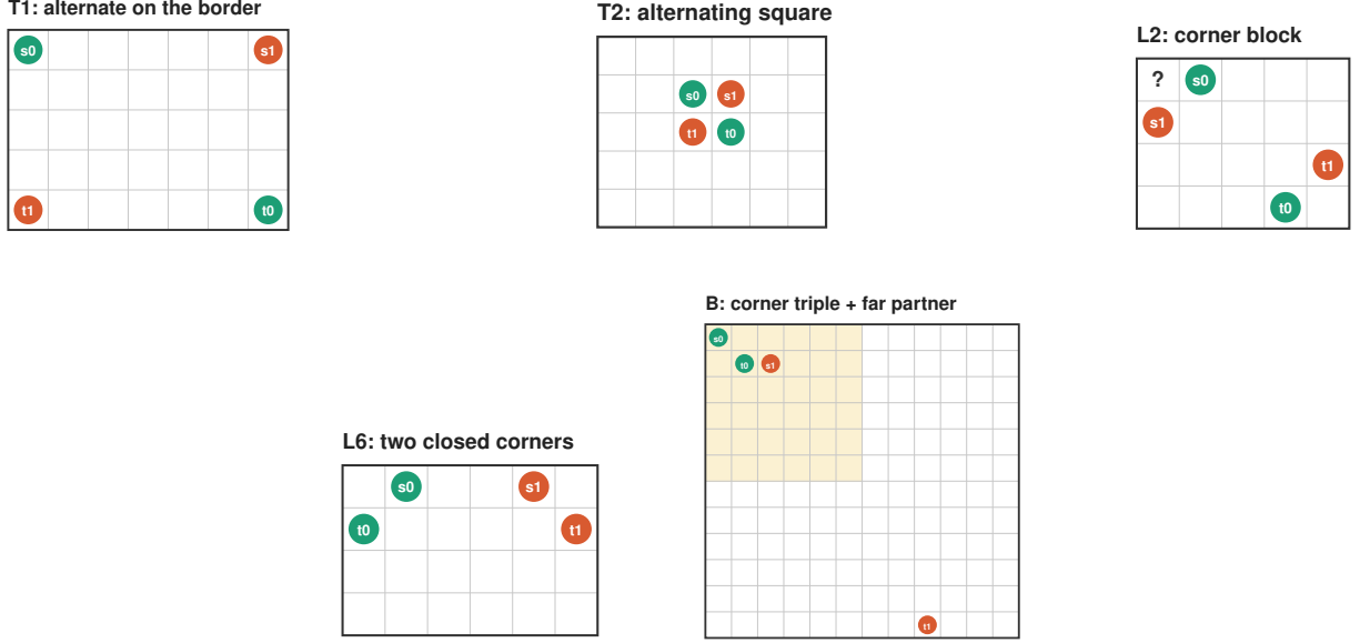
Figure 3: Entries T1, T2, L2, L6 and B. In T2 the endpoints fill a 2 \times 2 square with each colour on a diagonal, so the two paths would have to cross inside the square. In L2 the corner cell (marked ?) can only be reached from two endpoints of different colours. In B the 6 \times 6 corner window is shaded.
