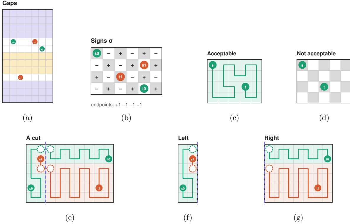
Figure 2: Definitions. (a) A 13 \times 7 instance. Rows 0–3 and 10–12 are free and form edge gaps (purple), and rows 6–8 form an internal gap (yellow). (b) Black cells have sign \sigma = +1 and white cells -1 . The endpoint signs sum to 0, which is 2 \cdot (RC \bmod 2) since RC = 24 is even, as parity requires. (c) A one-path piece. The cells s and t have different shades on a 4 \times 5 rectangle, so the pair is acceptable and a Hamiltonian s – t path exists. (d) Both cells are black on a rectangle with an even number of cells, so the pair is not acceptable. (e) A solution and a cut (dashed). Each colour crosses the cut once, and the two crossing pairs are circled. (f), (g) The pieces left and right of the cut, with the cut drawn on the side where they meet. Each crossing cell becomes a virtual endpoint (dashed) of its piece, and the pieces’ solutions glue back into (e).
