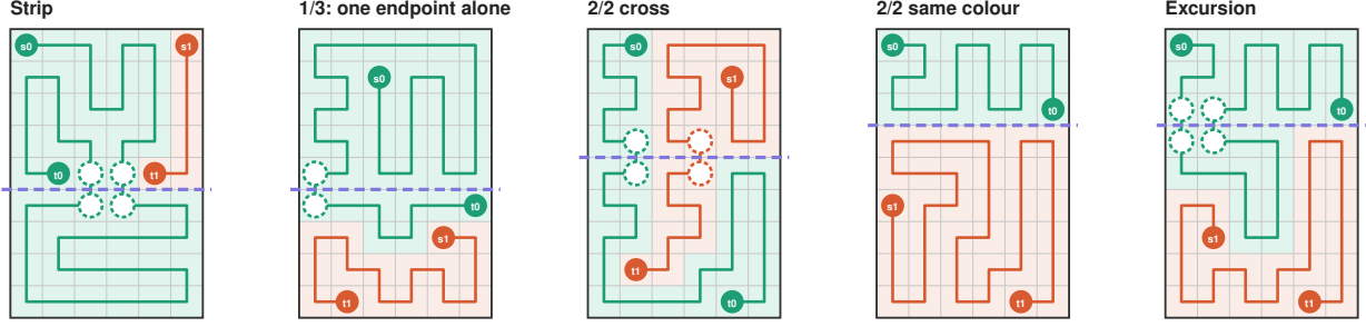
Figure 6: The five move types. Each cuts the rectangle along the dashed line, and the dashed circles mark crossing pairs, whose cells become virtual endpoints of the pieces. In a strip all four endpoints lie on one side, and the other side is an empty block of even area, spliced into a path that runs along the cut. In a 1/3 move one endpoint is alone on its side. Its path crosses the cut once, so that side is a one-path piece from the endpoint to its crossing cell, and the other side is a two-path piece. In a 2/2 cross each side holds one endpoint of each colour. Each path crosses once, and both sides are two-path pieces. In a 2/2 same colour move each side holds both endpoints of one colour. No path crosses, and both sides are one-path pieces. In an excursion each side holds one whole pair as in 2/2 same , but one path (here colour 0) leaves its side and returns, crossing twice.
