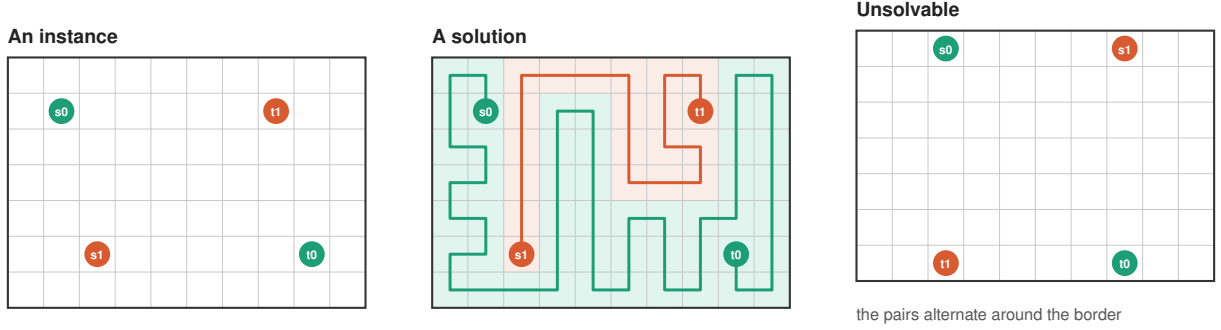
Figure 1: Two-colour Zig-Zag Numberlink on a 7 \times 10 rectangle. Left, an instance with endpoints s_0, t_0 of colour 0 (green) and s_1, t_1 of colour 1 (orange). Middle, a solution. The two vertex-disjoint paths s_0 \rightarrow t_0 and s_1 \rightarrow t_1 together visit every cell, and the colour-0 path winds around the colour-1 path. Right, an unsolvable instance. The endpoints alternate in colour around the border, so the two paths would have to cross (catalogue entry T1, Section 5).
