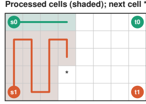
Figure 8: Processed cells (shaded) and the next cell (*).
