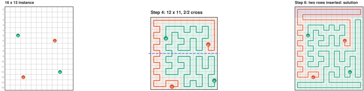
Figure 7: A 16 \times 13 instance, the 12 \times 11 core with its 2/2-cross move, and the solution.
