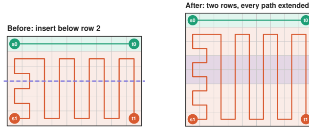
Figure 5: Band extension. Two rows are inserted below row 2.
