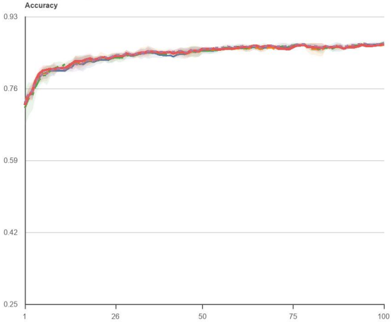
Fashion-MNIST ( \alpha=1.0 )
