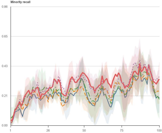
Fashion-MNIST ( \alpha=0.3 )
