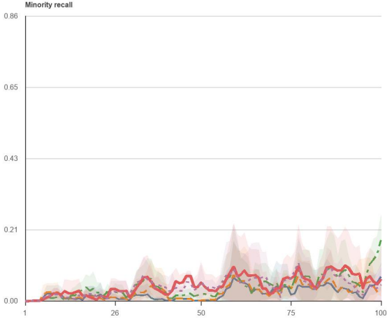
Fashion-MNIST ( \alpha=0.1 )
