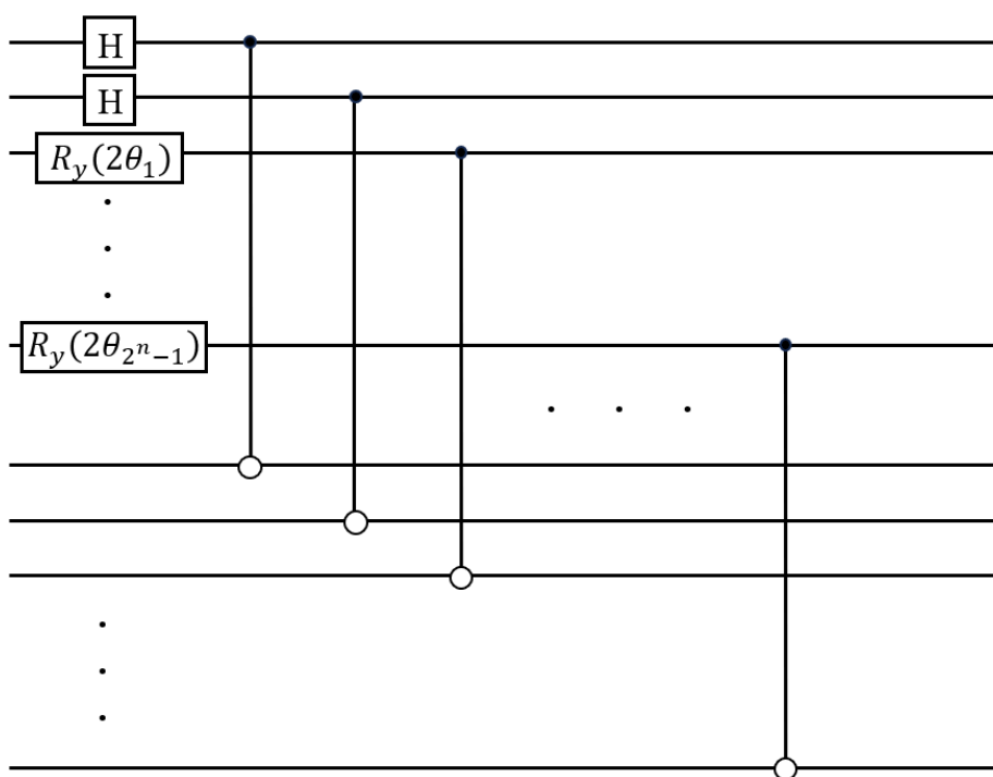
Figure 2: 多量子纠缠量子门电路示意
