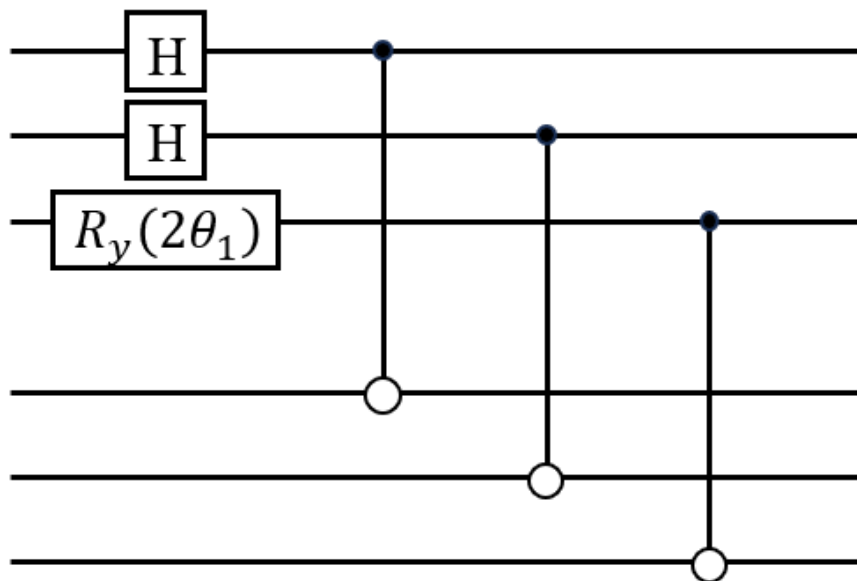
Figure 1: 三量子纠缠量子门电路示意
