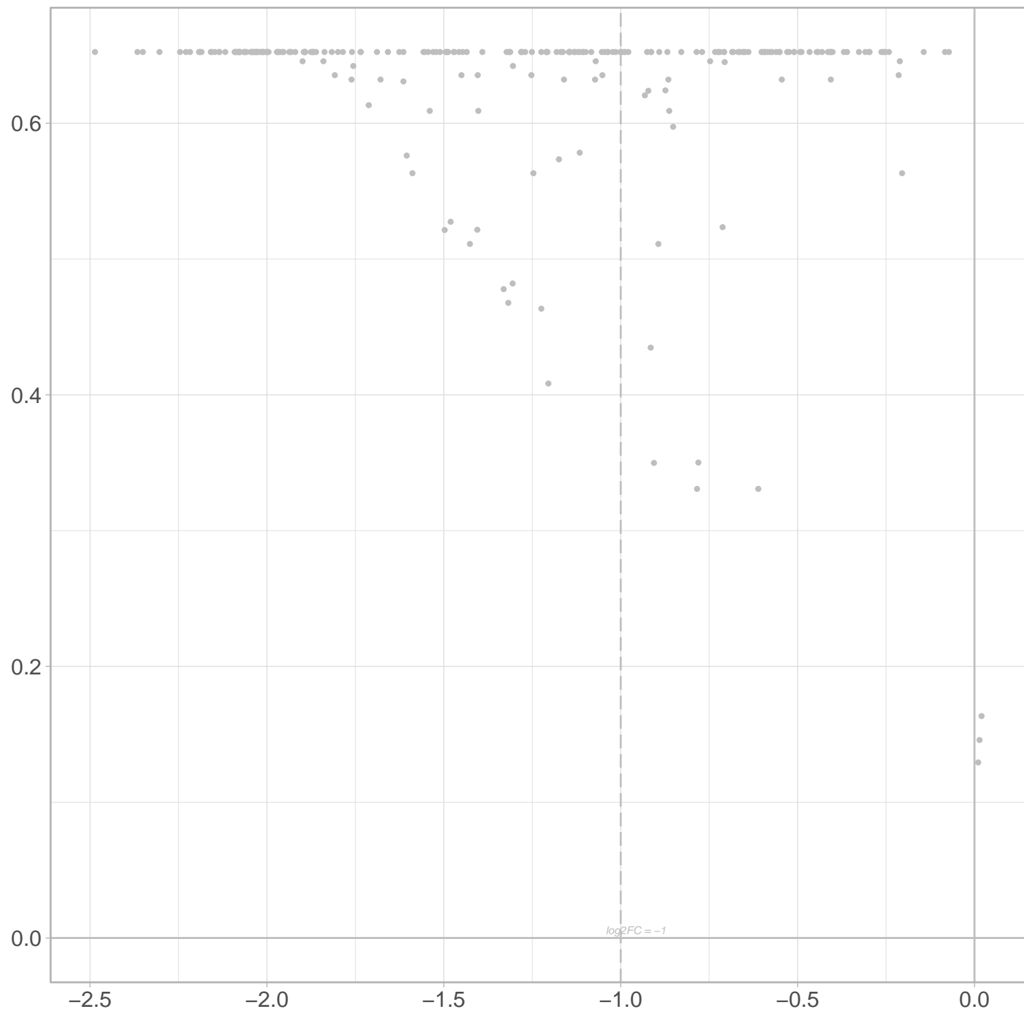
Lab2 vs Lab1 Differential Expression
