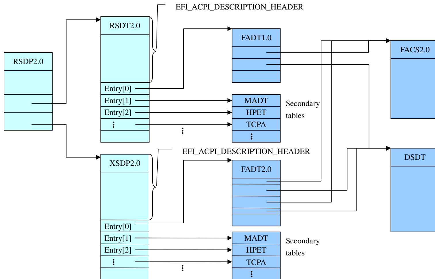
Figure1 Xen hvmloder ACPI tables structure
