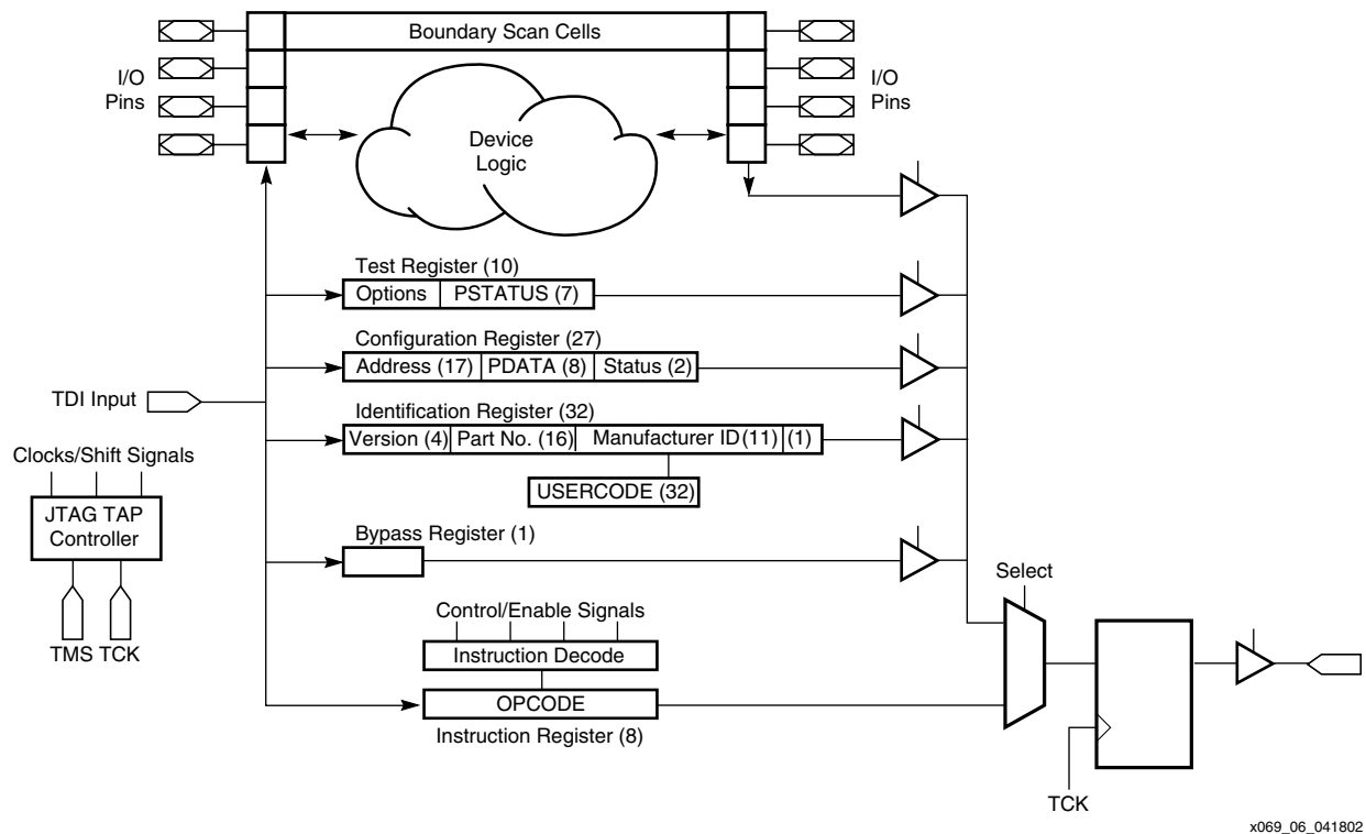
Figure 6: JTAG Architecture
