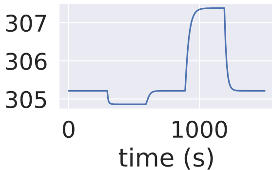
sCO 2 out (K)
