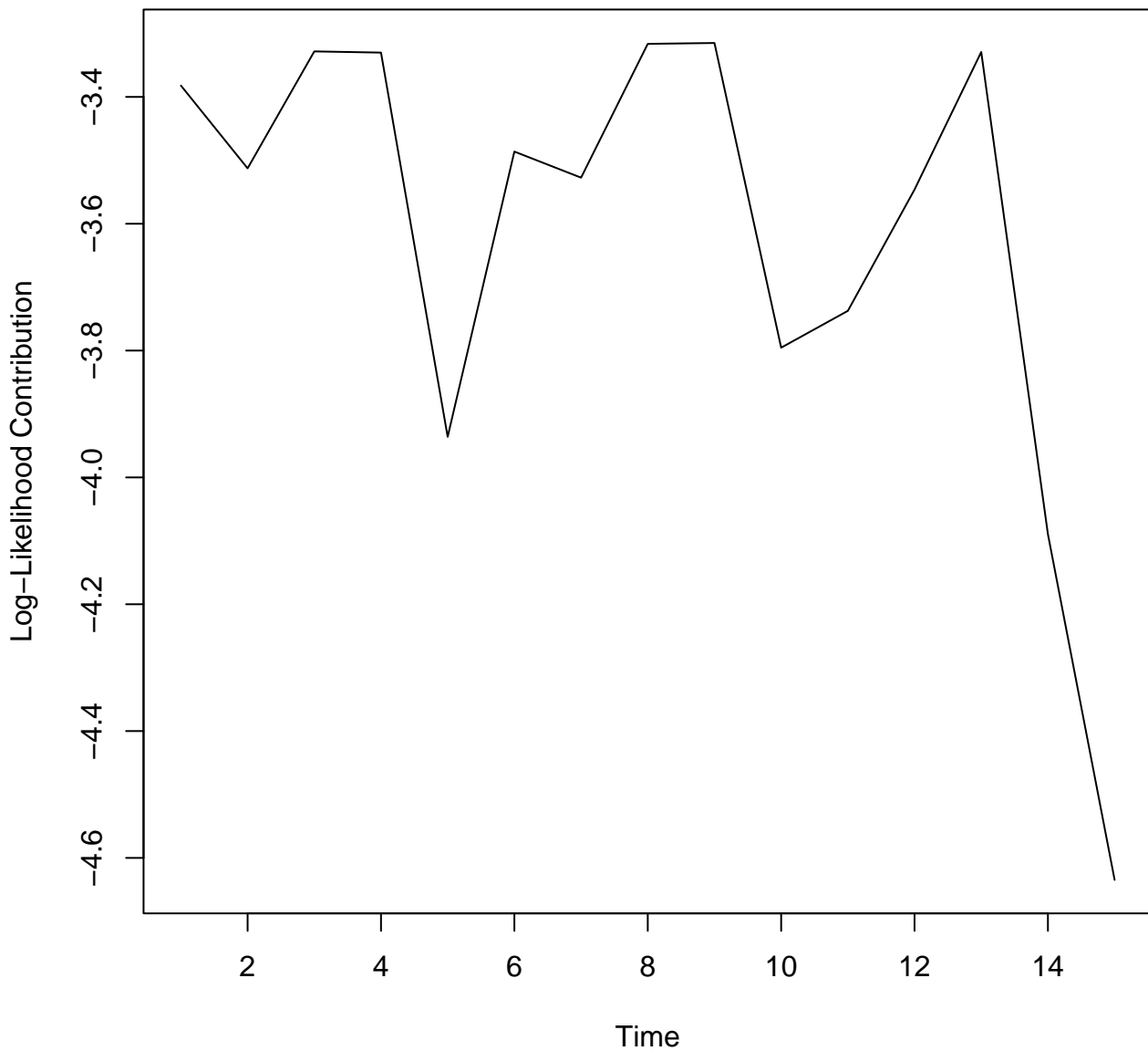
Log-Likelihood Contributions Over Time
