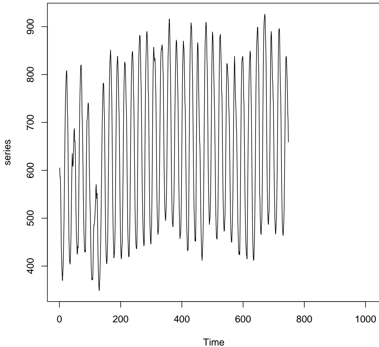
M4 hourly series: H1
