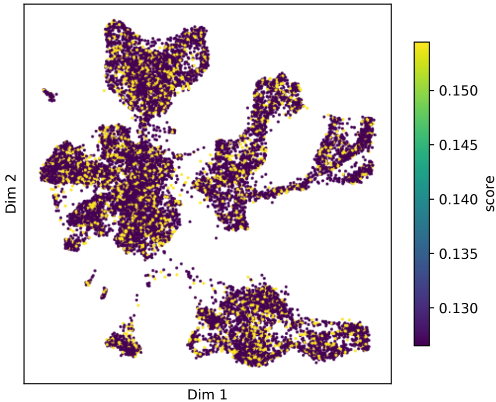
GOZGIT_ESR1_TARGETS_DN
