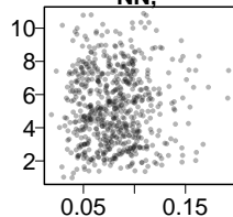
F-MDS, 0.6
