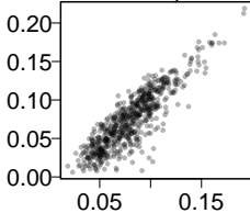
superMDS, 0.4
