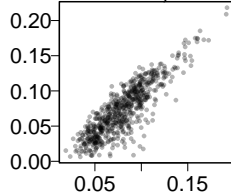
superMDS, 0.6
