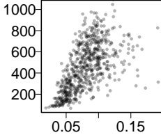
Isomap, 10
