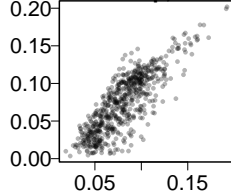
Isomap, 10
