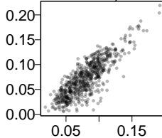
superMDS, 0.8
