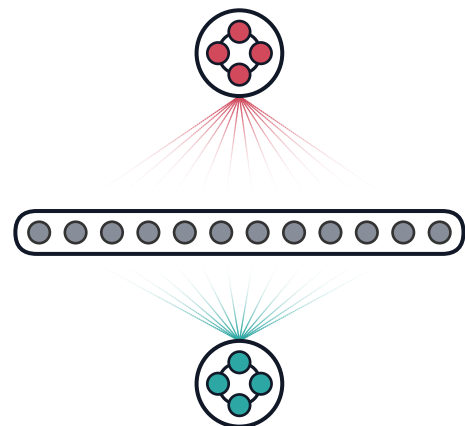
RRR (Non-spatial)
