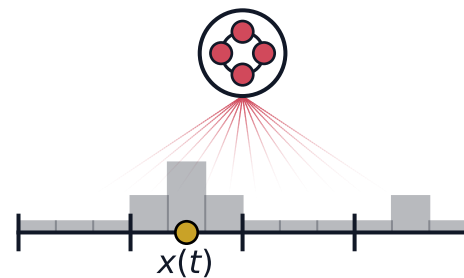
High-D PF
