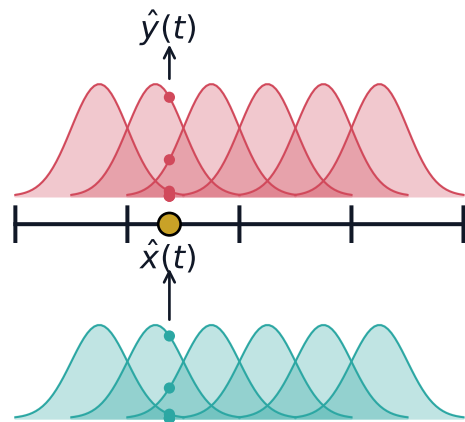
RRR (Non-spatial)
