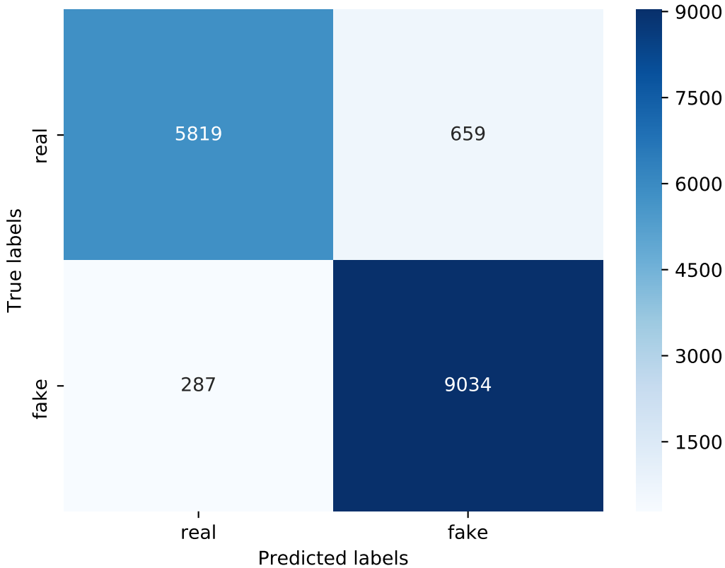
Confusion Matrix
