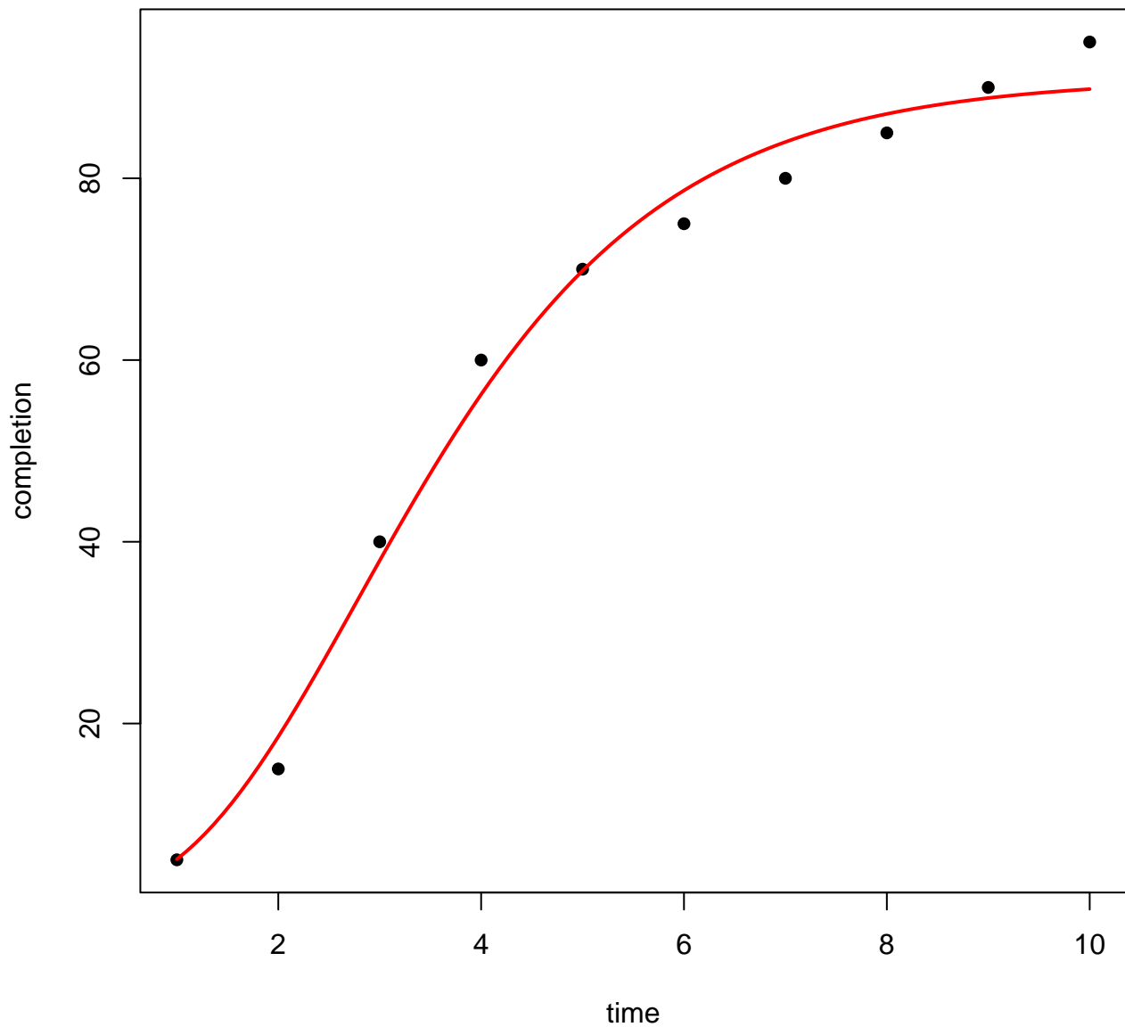
Fitted Gompertz Model
