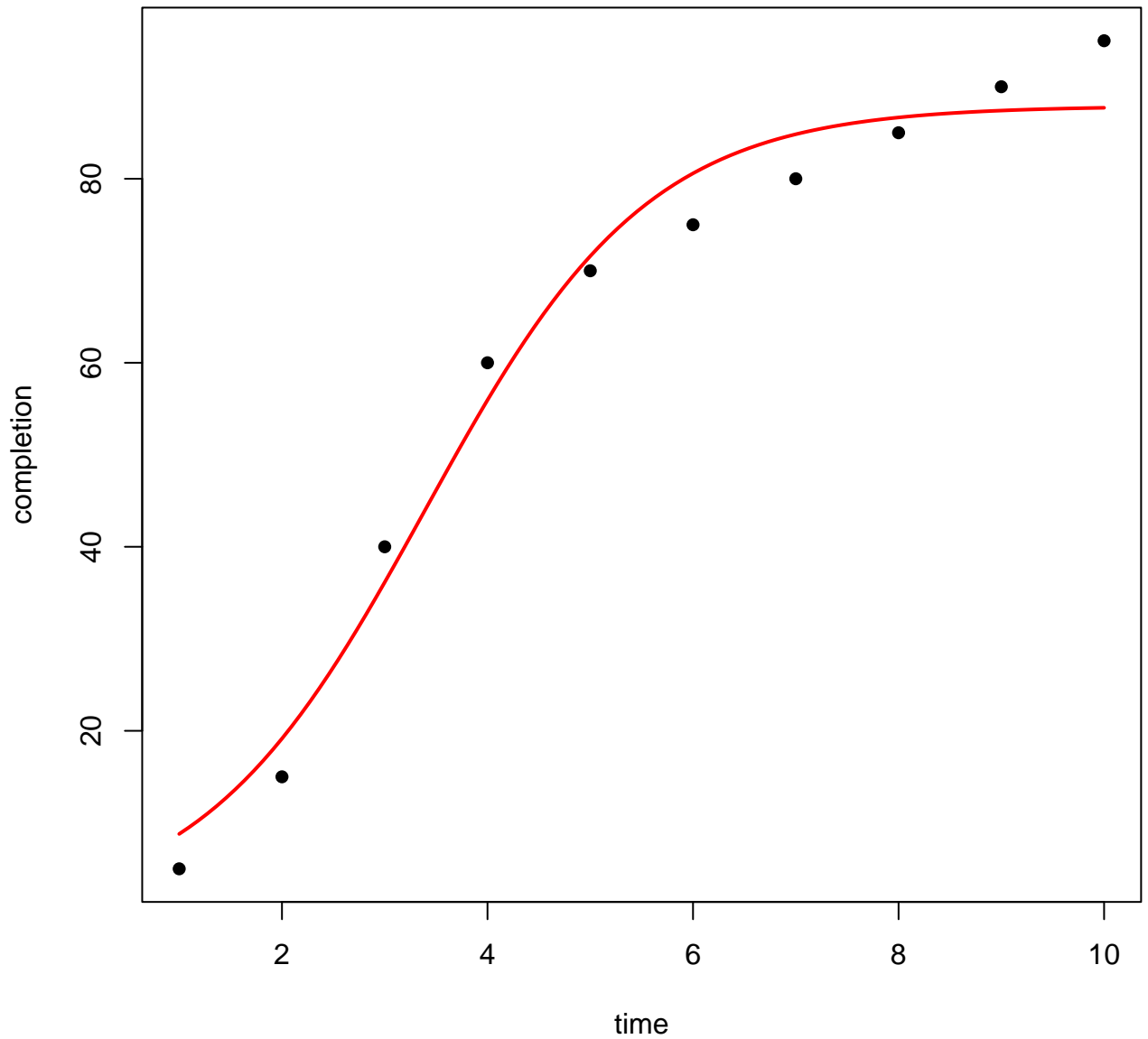
Fitted Pearl Model
