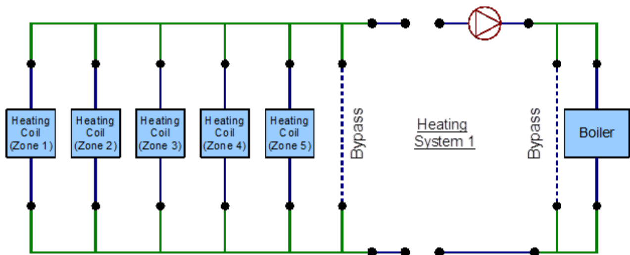
Figure 44 - EnergyPlus line diagram for heating loop
