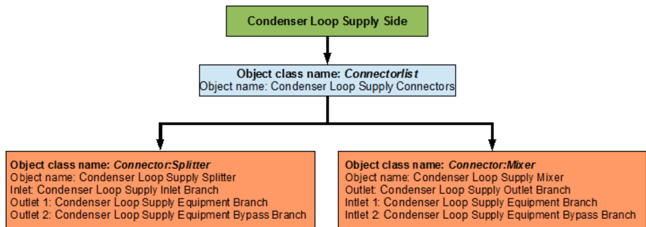
Figure 66 – Flowchart for condenser loop supply side connectors
