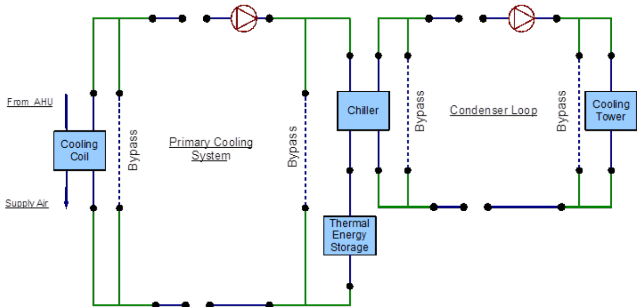
Figure 43 - EnergyPlus line diagram for cooling system
