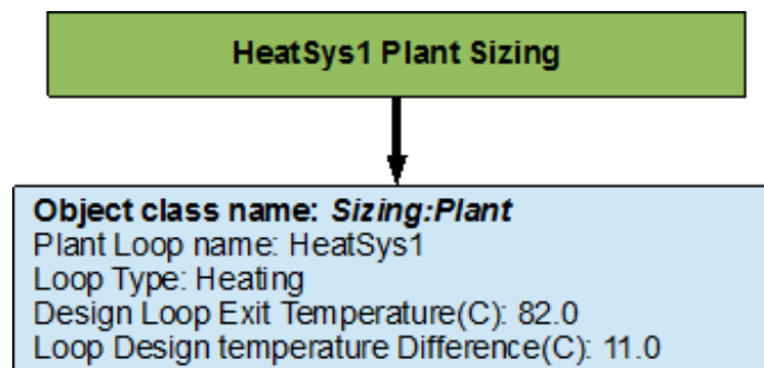
Figure 86 - Flowchart for heating loop sizing
