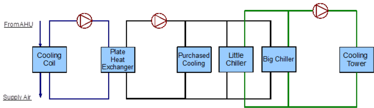
Figure 88 - Simple line diagram for the cooling system
