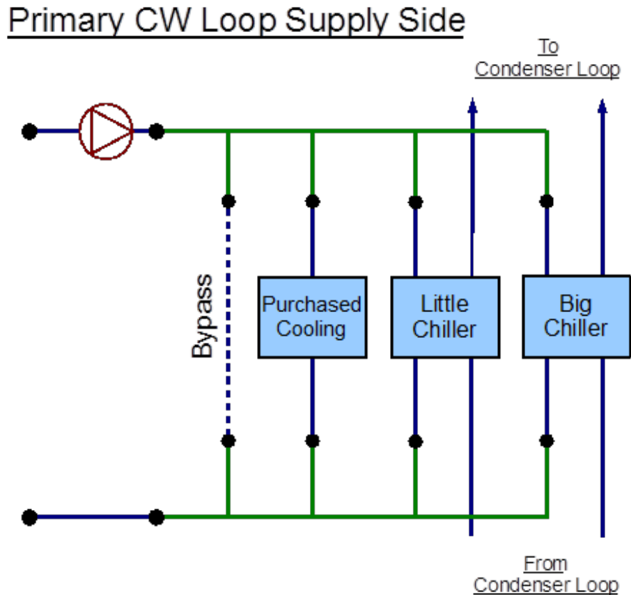
Figure 93 - EnergyPlus line diagram for the supply side of the primary chilled water loop
