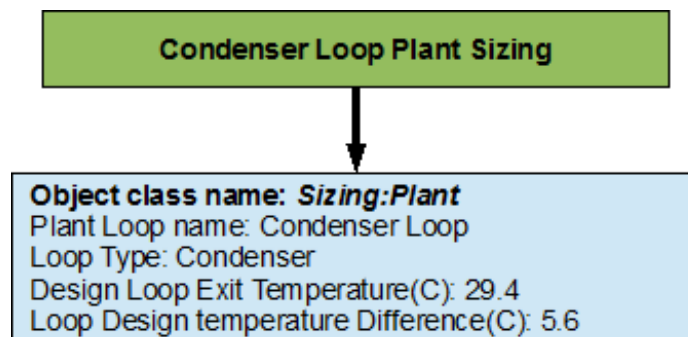
Figure 73 – Flowchart for condenser loop sizing
