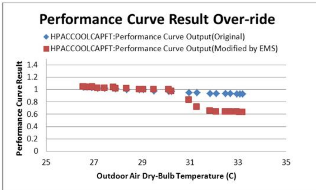
Figure 4. Results of Performance Curve Override
