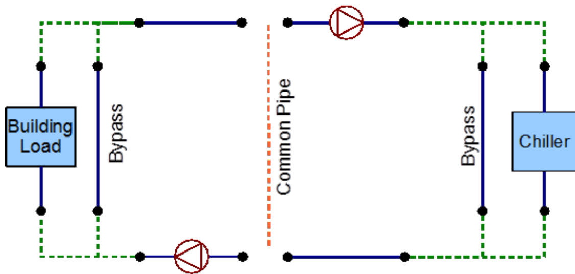
Figure 8 - Branch definition
