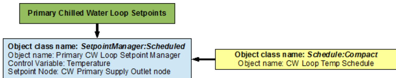
Figure 102 – Flowchart for Primary Cooling Loop setpoints
