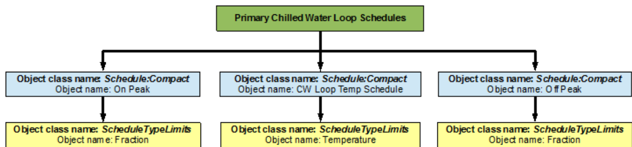
Figure 99 – Flowchart for primary chilled water loop schedules
