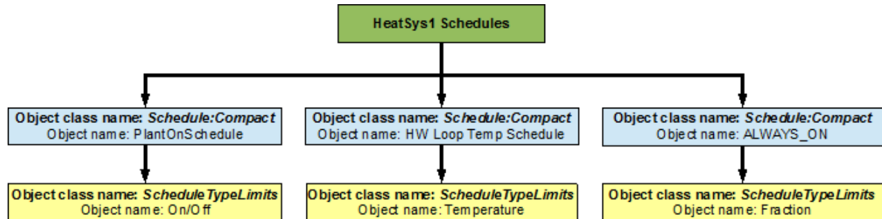
Figure 83 – Flowchart for heating loop schedules
