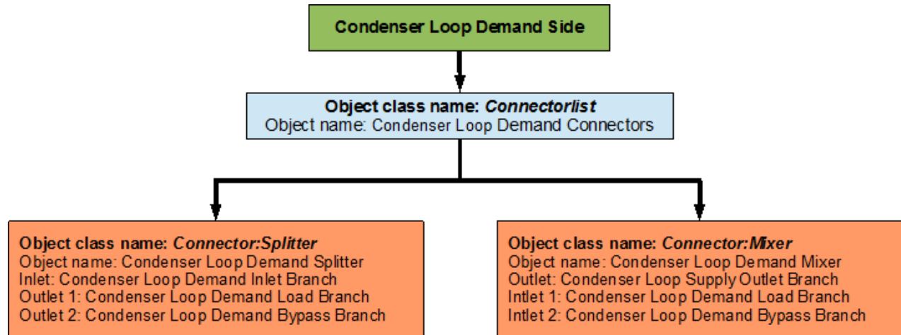
Figure 69 – Flowchart for condenser loop demand side connectors
