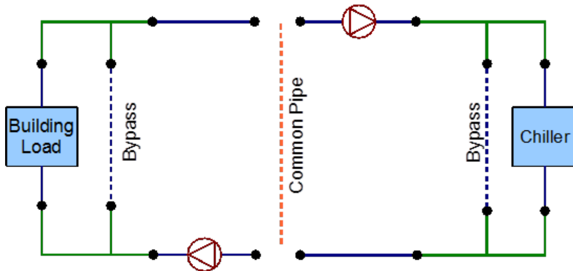
Figure 87 – Example of a common pipe setup
