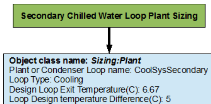
Figure 115 – Flowchart for secondary chilled water loop sizing
