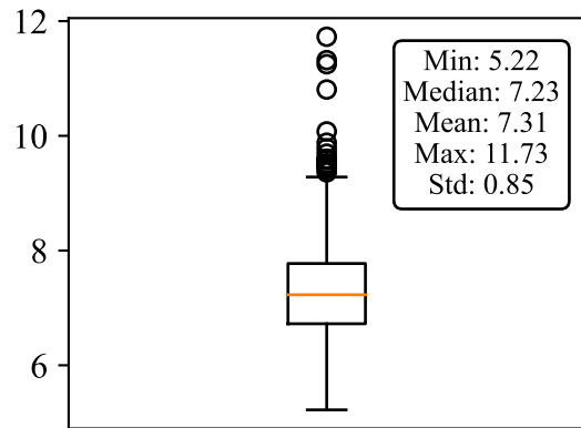
(f) Overall
