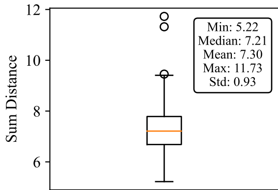
(a) Davinci-002
