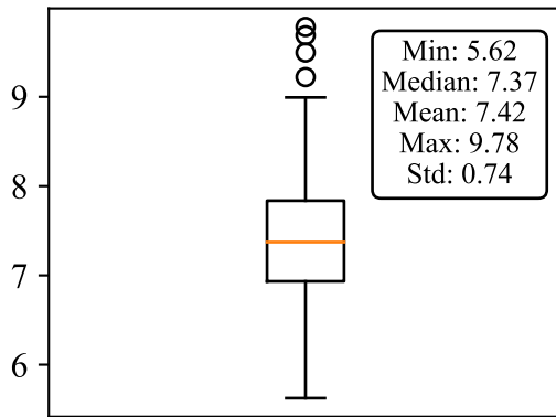
(b) ChatSonic
