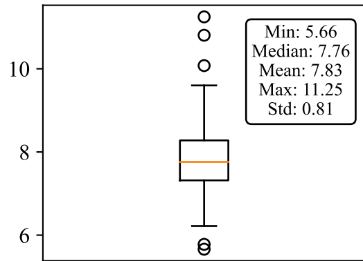
(c) Claude
