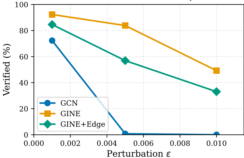
GNN Verification vs. Perturbation (IEEE 24-Bus)
