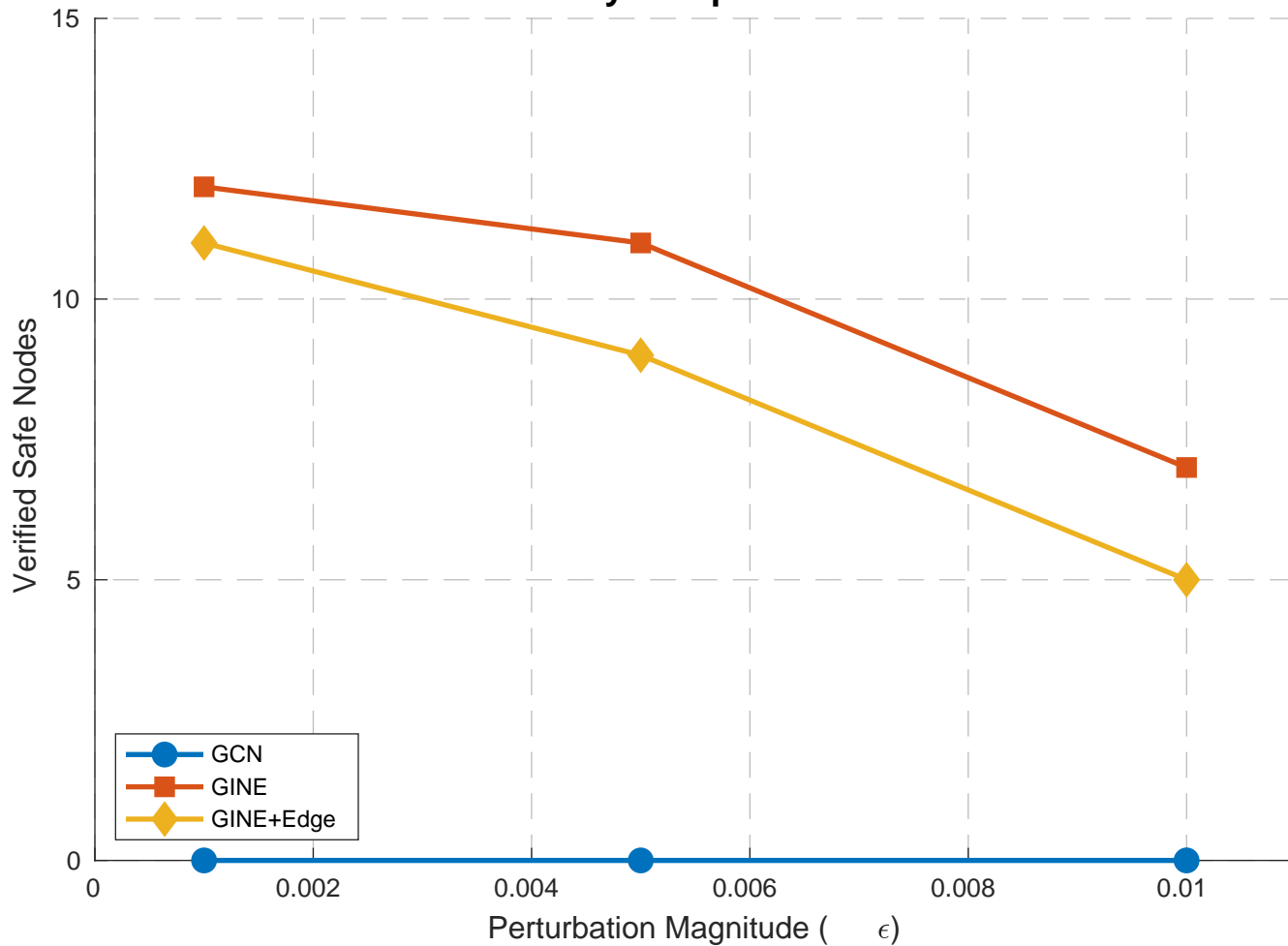
Verification Sensitivity to Input Perturbation
