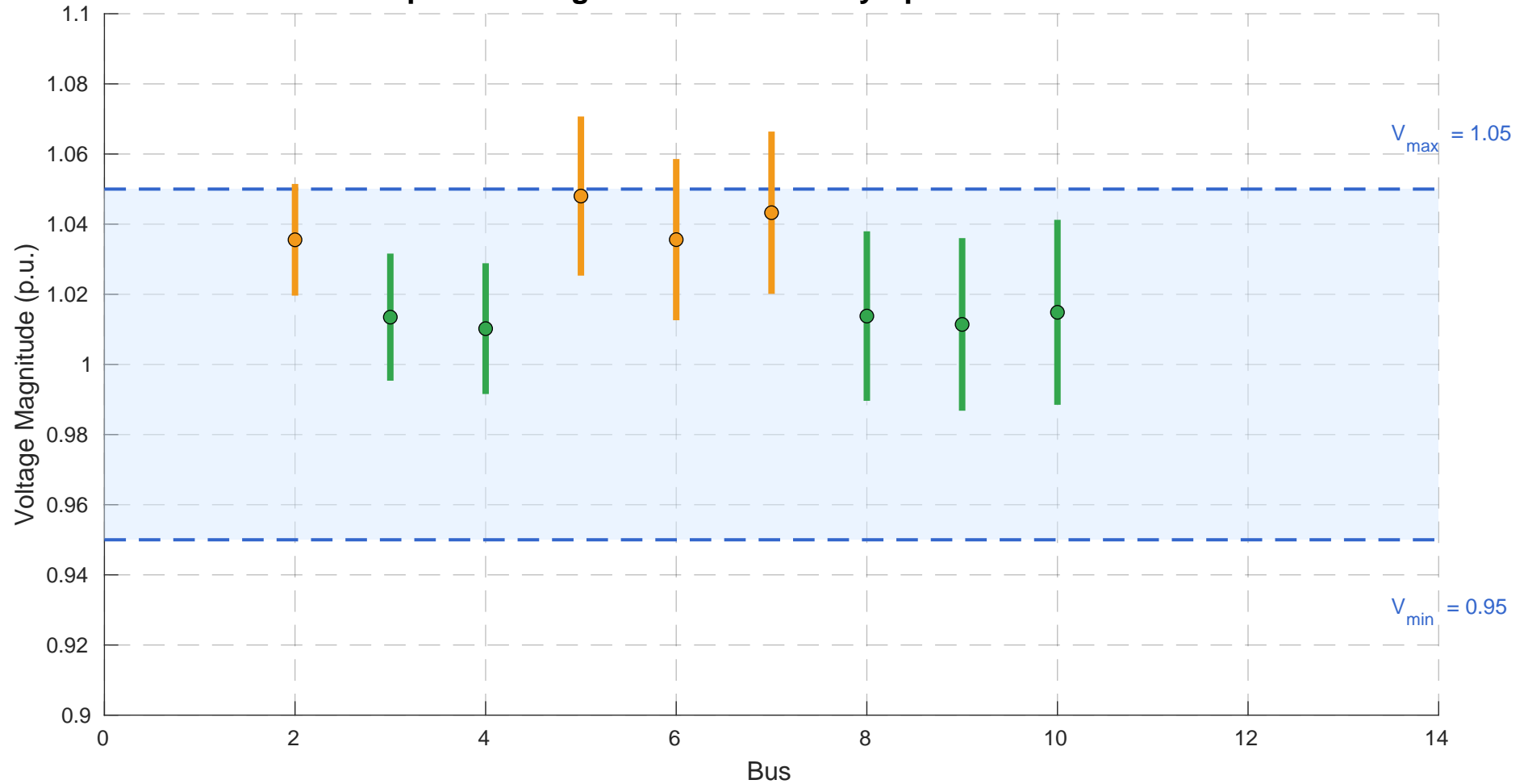
Computed Voltage Bounds vs. Safety Specification
