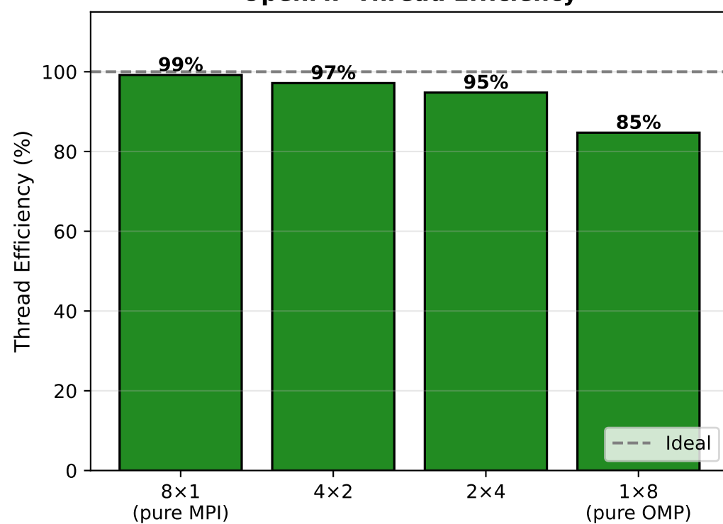
OpenMP Thread Efficiency
