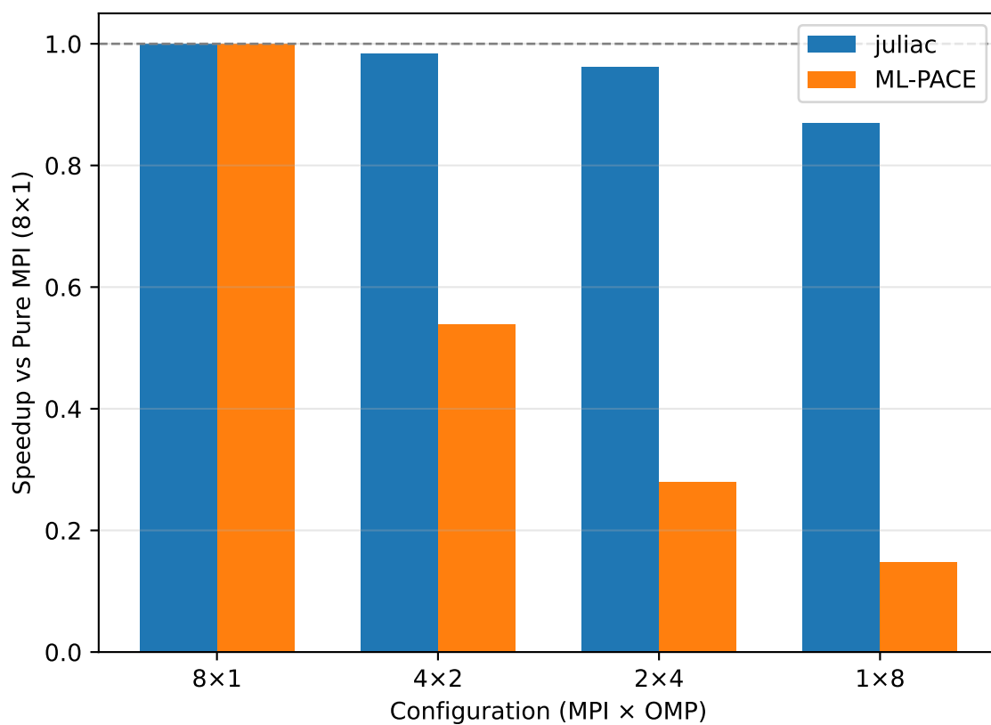
Relative Performance vs Pure MPI Baseline
