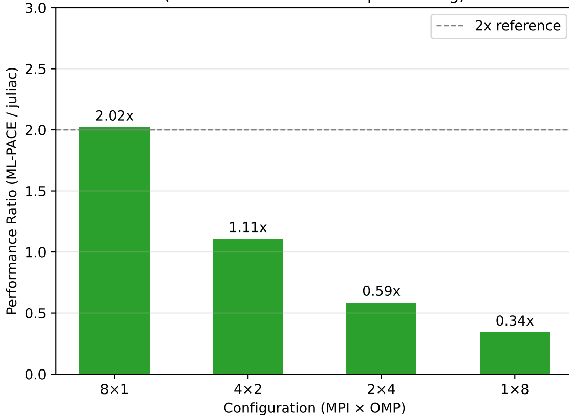
Performance Ratio vs Hybrid Configuration (constant \approx 2x means equal scaling)
