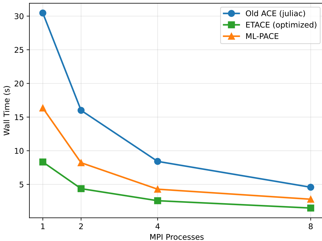
Parallel Speedup
