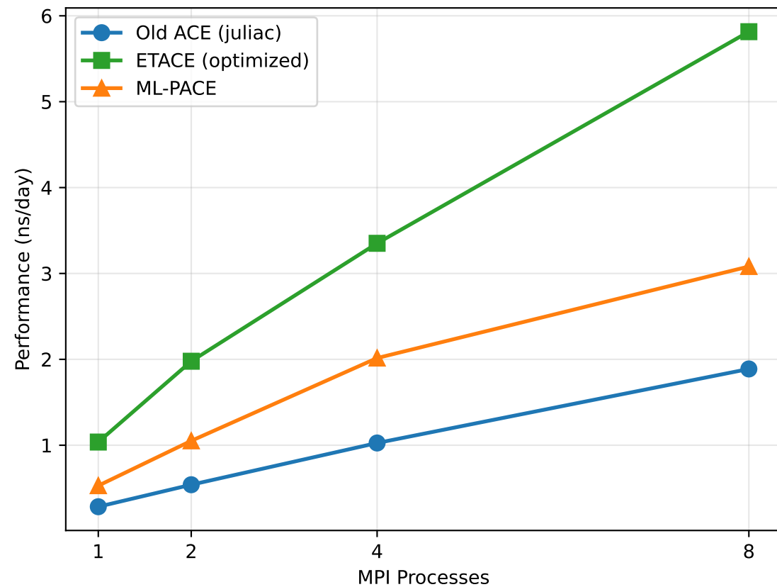
Parallel Efficiency
