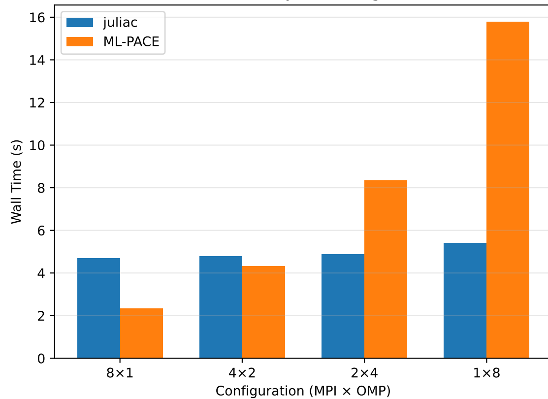
Wall Time vs Hybrid Configuration
