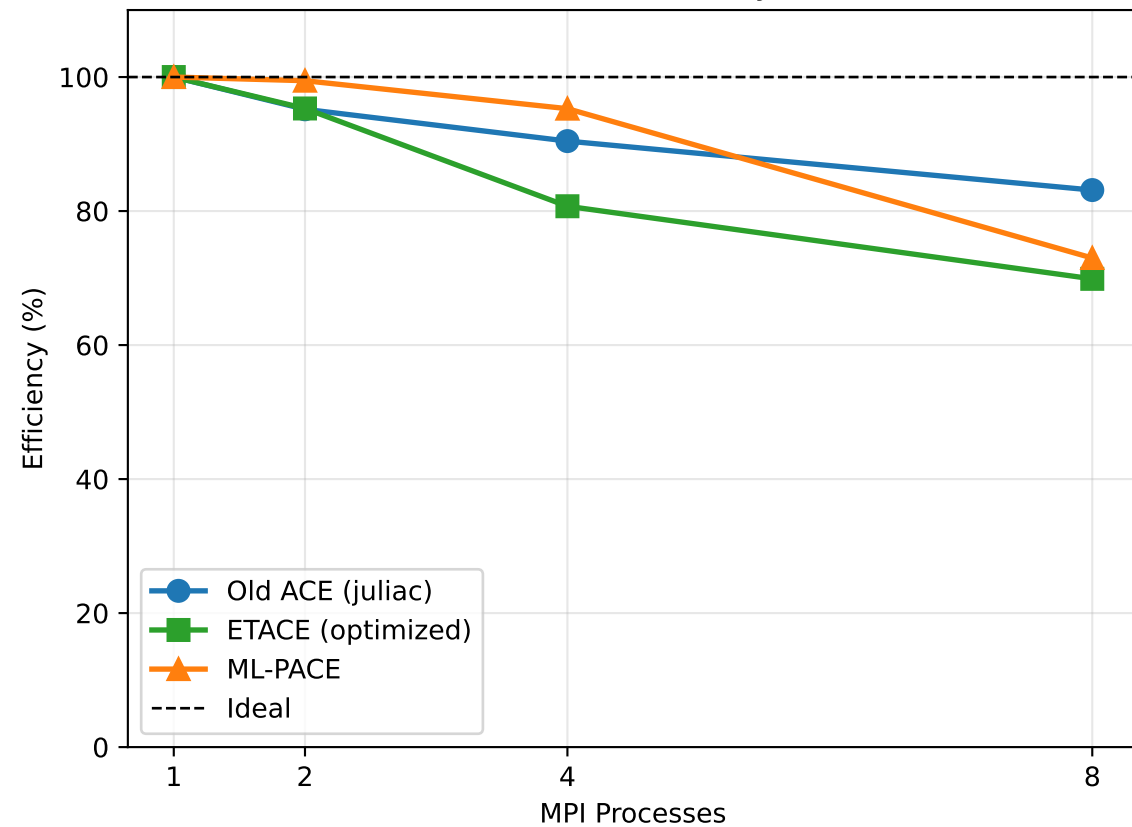
Parallel Efficiency
