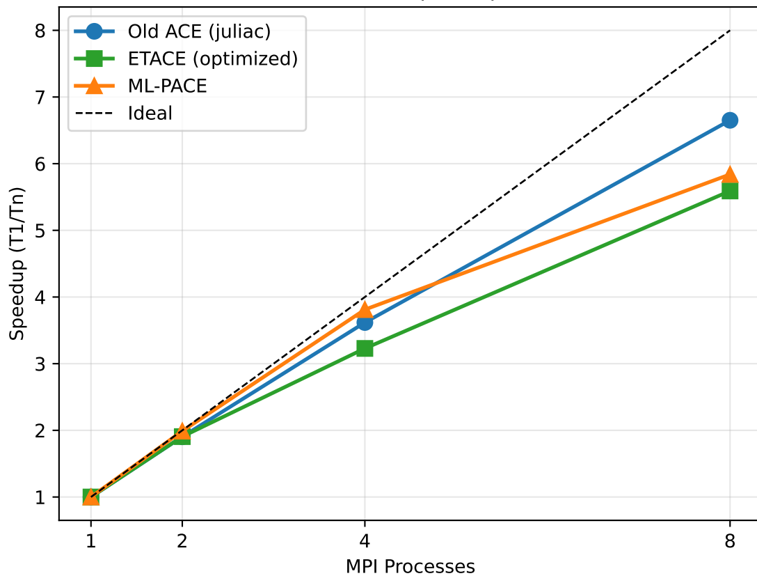
Parallel Speedup
