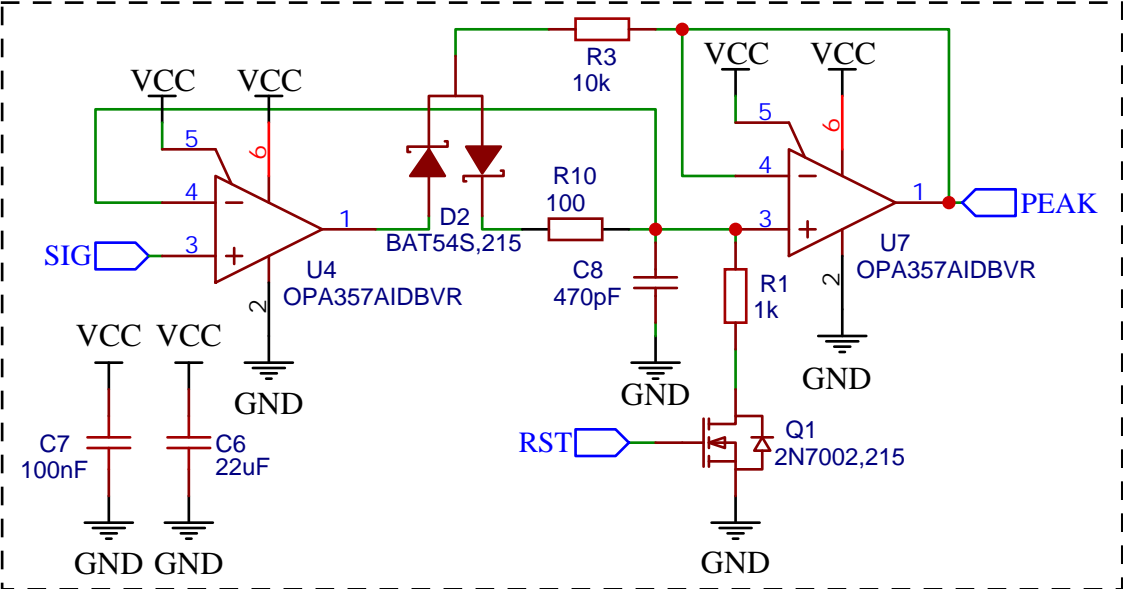
Sample and Hold / Peak Detector
