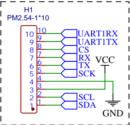
IO Connections
