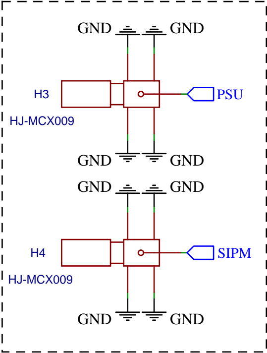
SiPM Connection MCX
