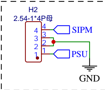
SiPM Connection Pins
