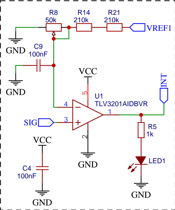
Pulse Discriminator (~0 - 320 mV)
