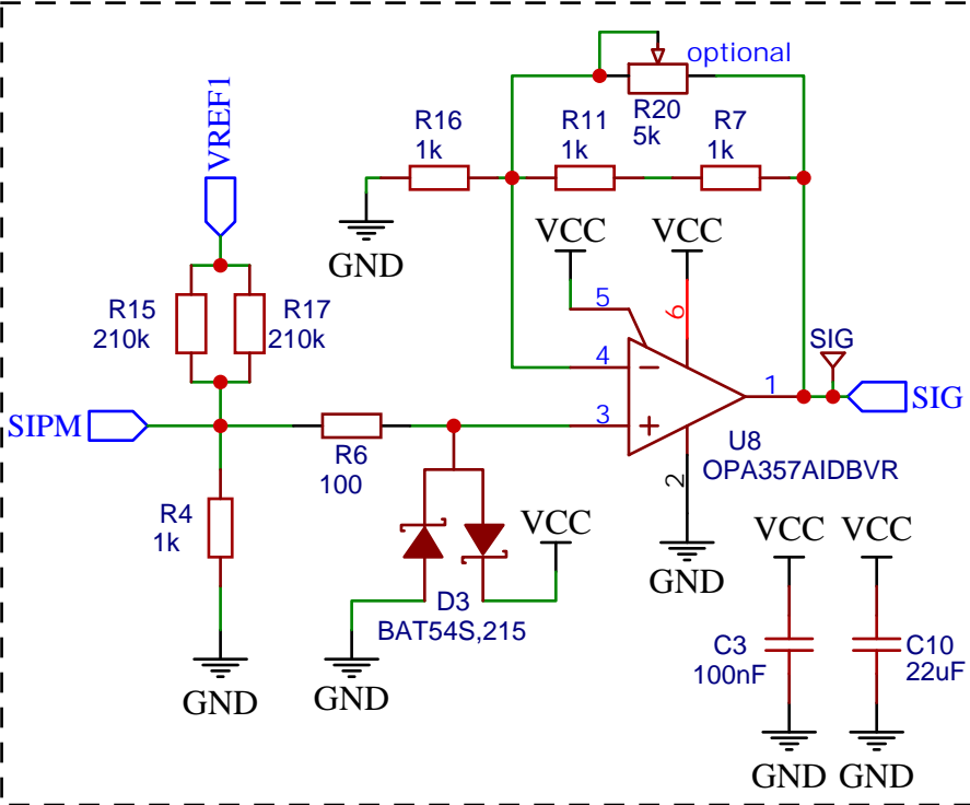
SiPM Output and Preamplifier
