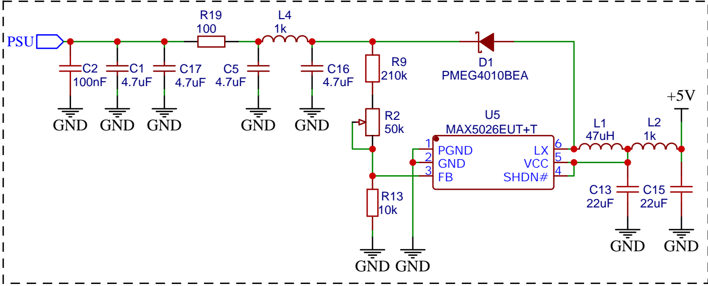
SiPM Bias 27.5 - 33.75 V (not temp corrected)
