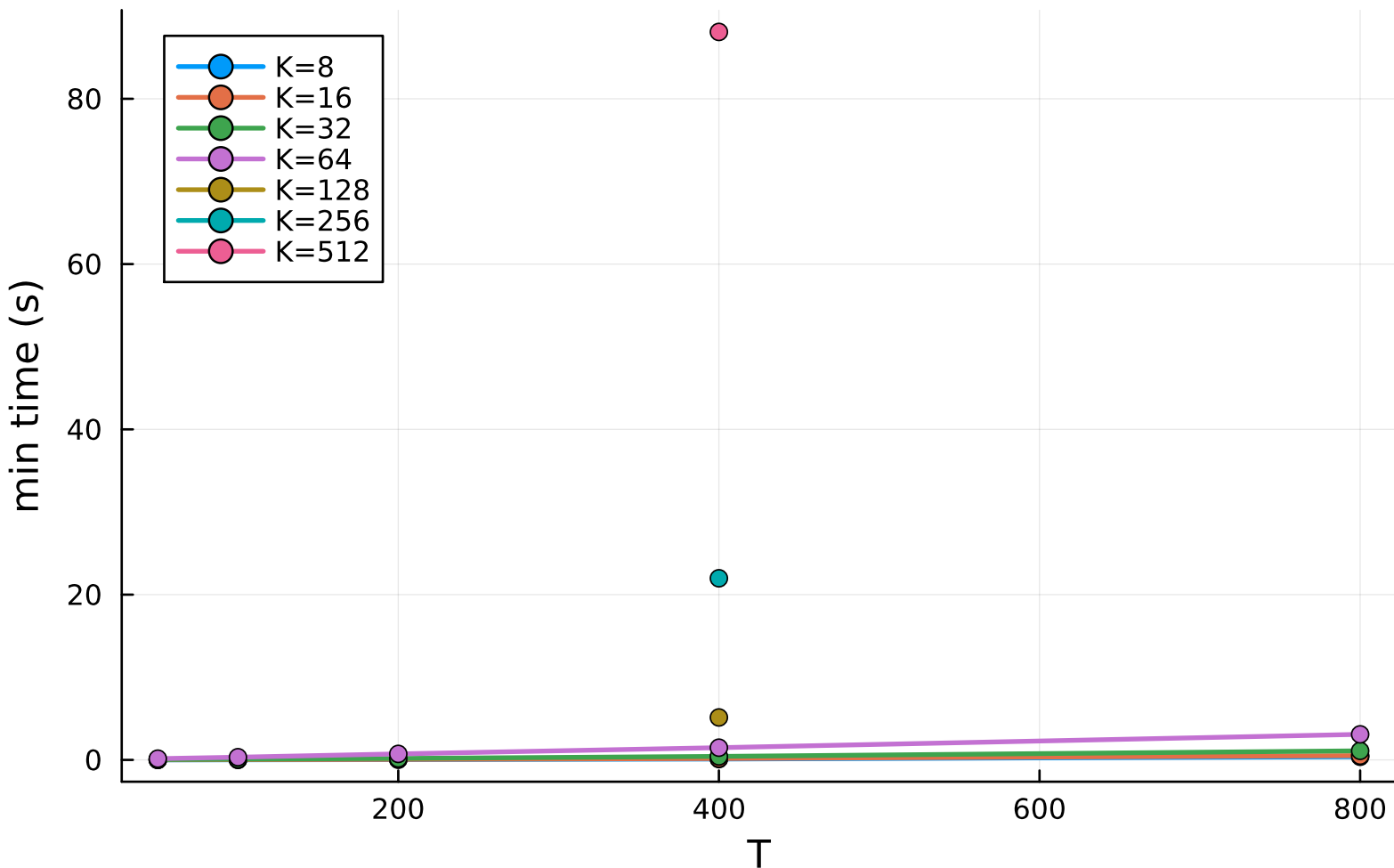
HMM scaling: time vs T (interleaved)
