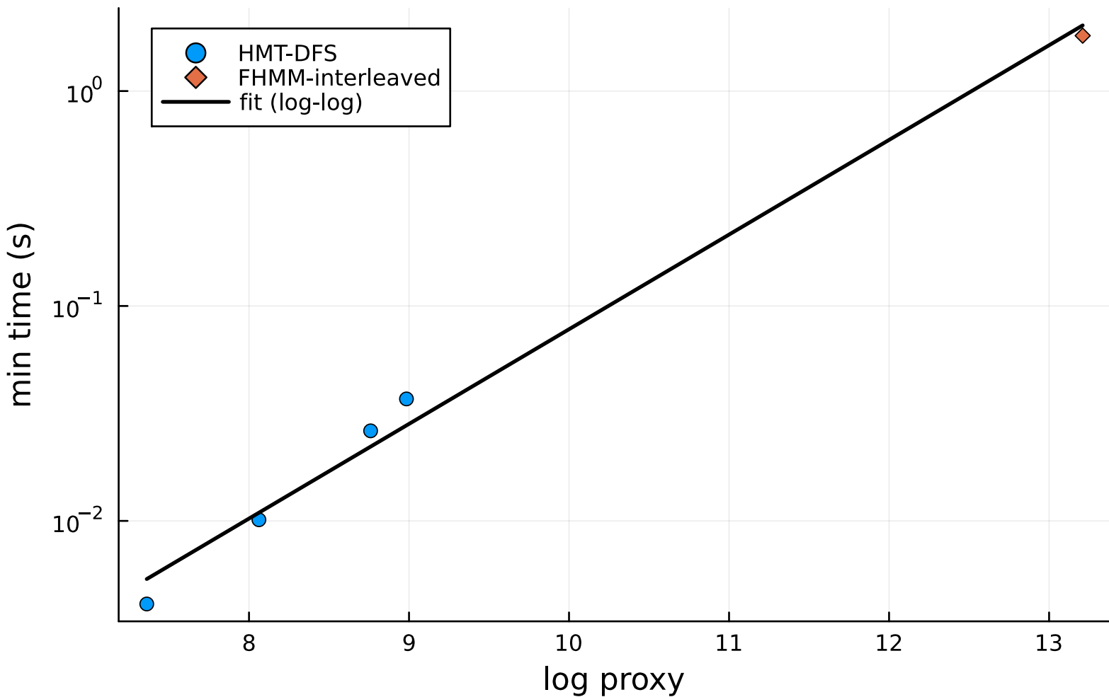
Runtime vs proxy ( \log R^2=0.991 )
