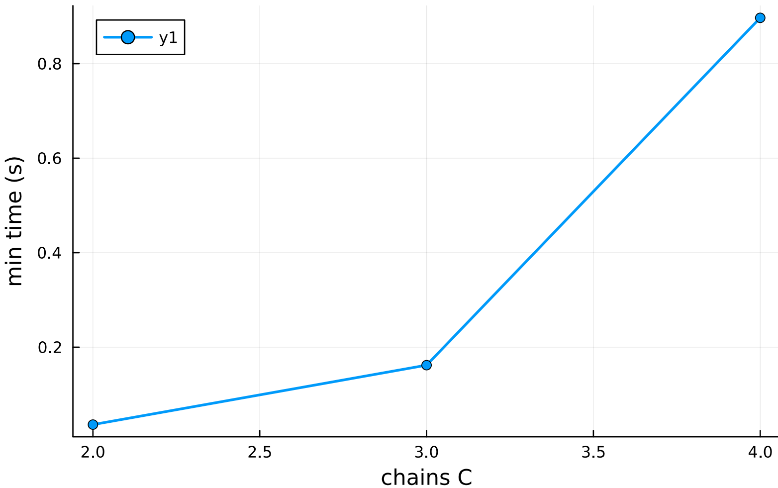
FHMM interleaved: time vs C (K=4, T=100)
