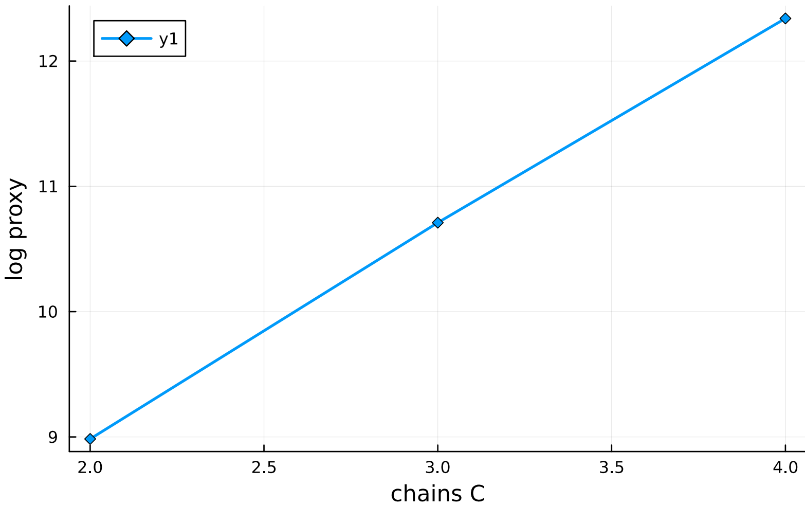
FHMM interleaved: \log \Sigma K^{\text{width}} vs C
