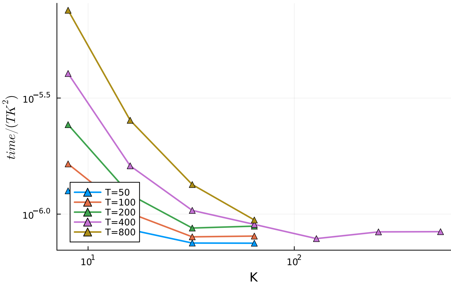
HMM normalized vs K
