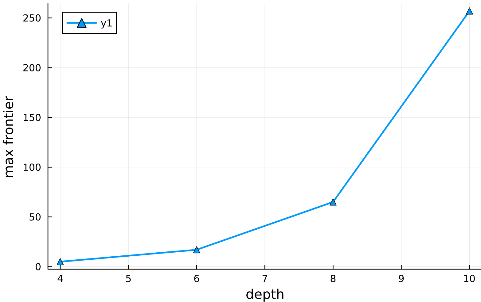
HMT BFS: max frontier vs depth
