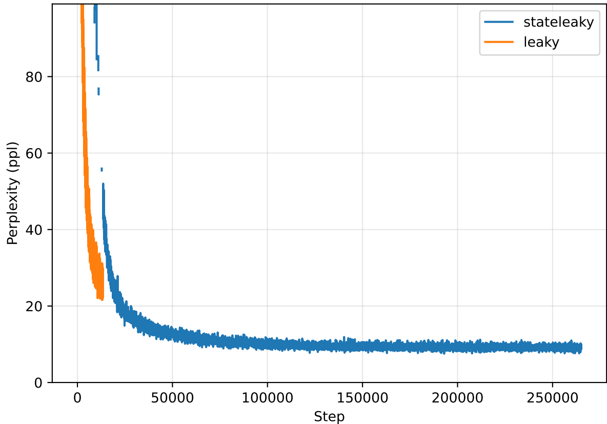
Perplexity vs Batches Processed
