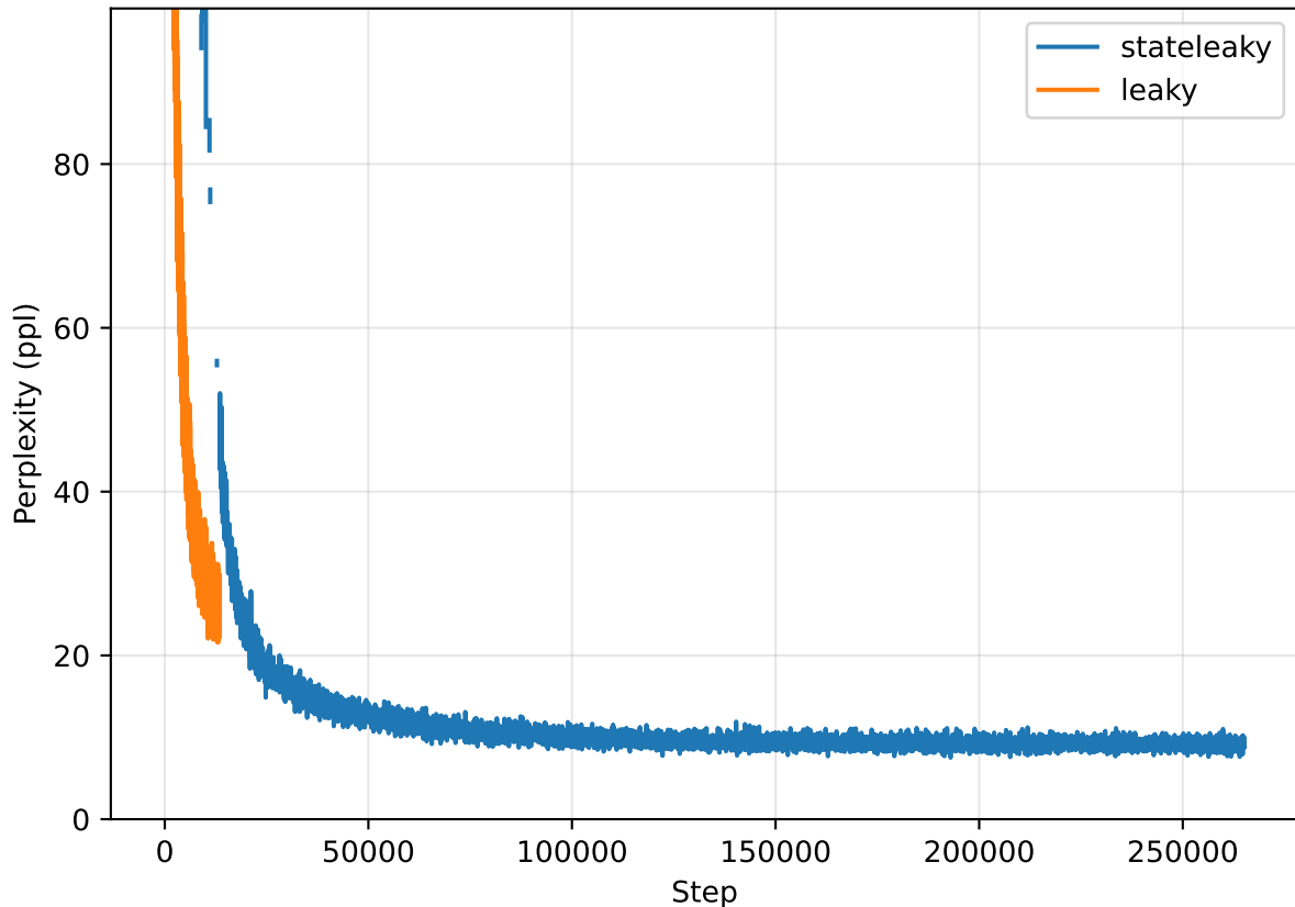
Perplexity vs Batch/Step (y truncated at 99)
