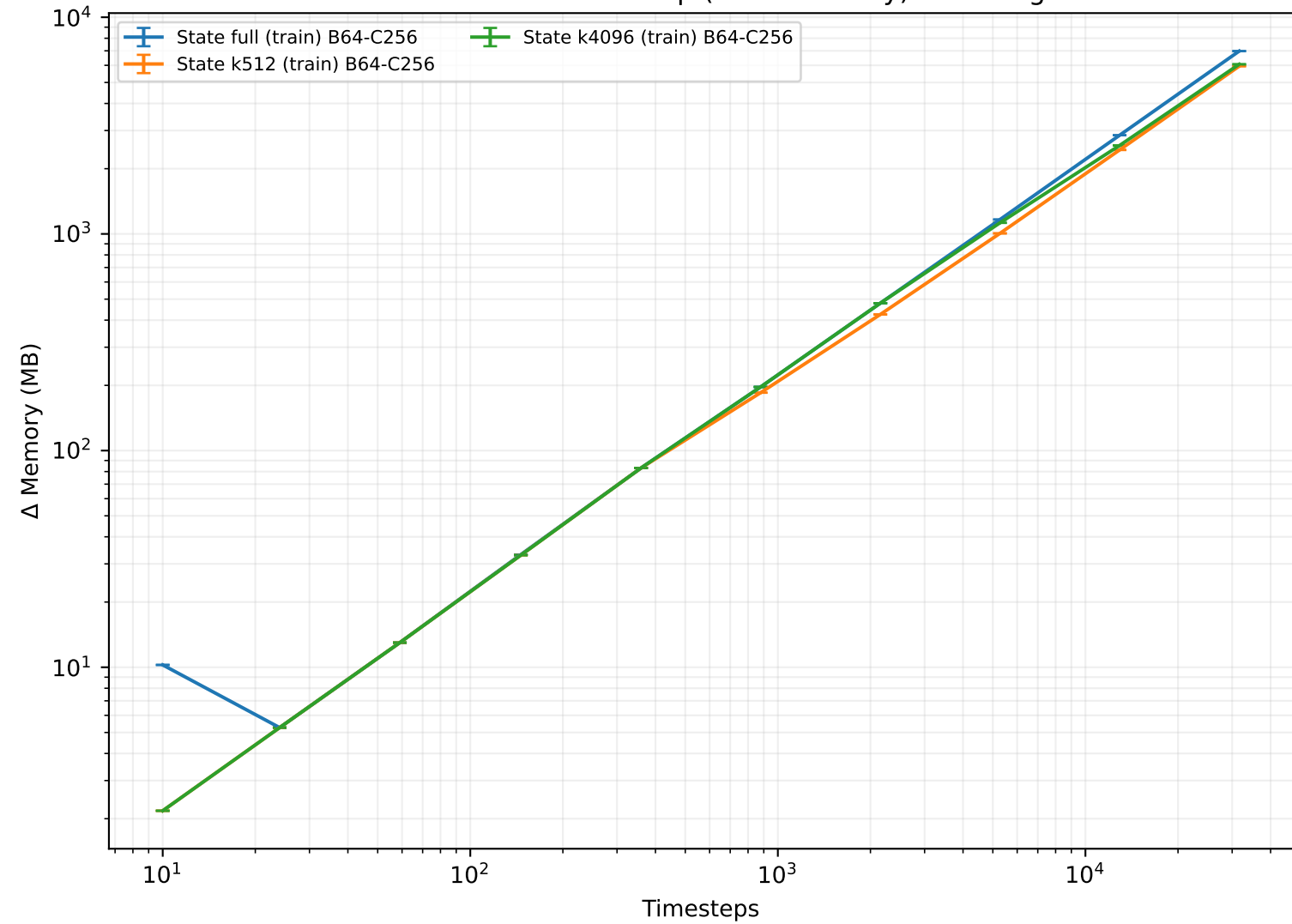
Kernel Truncation Sweep (Peak Memory) - Training
