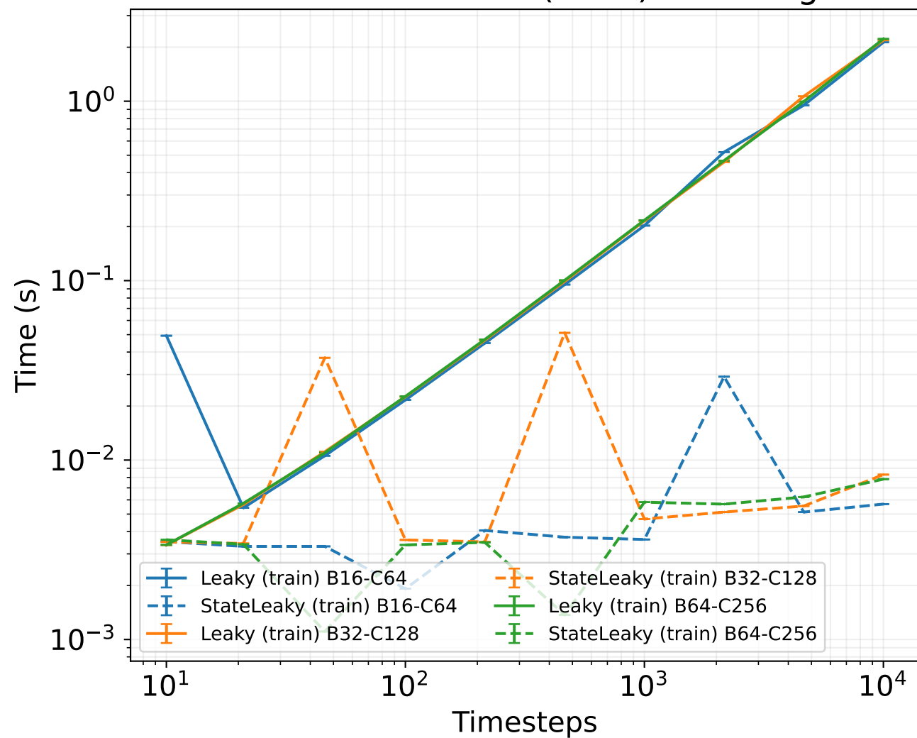
SNN Performance (Time) - Training
