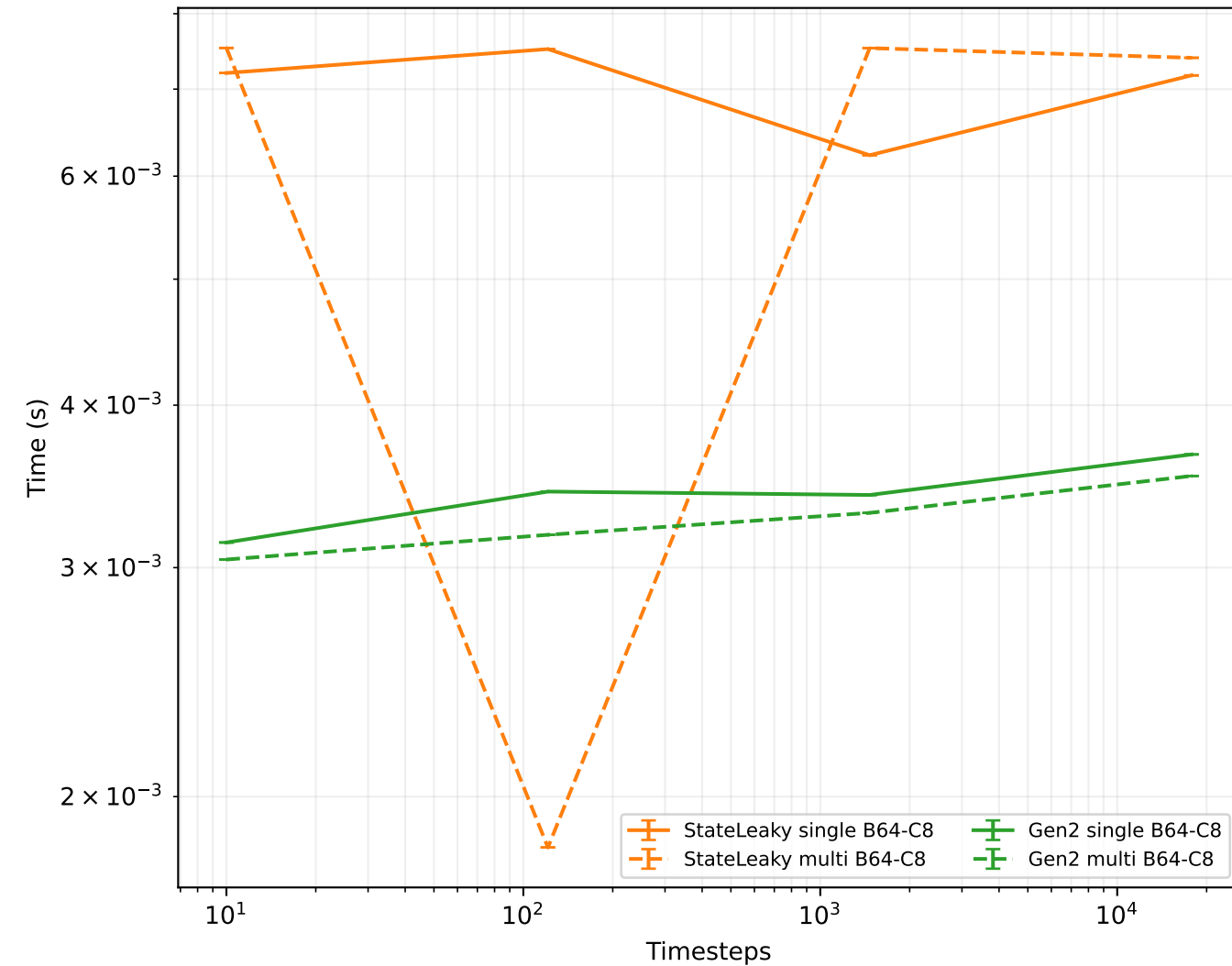
SNN Performance (Time) - Inference
