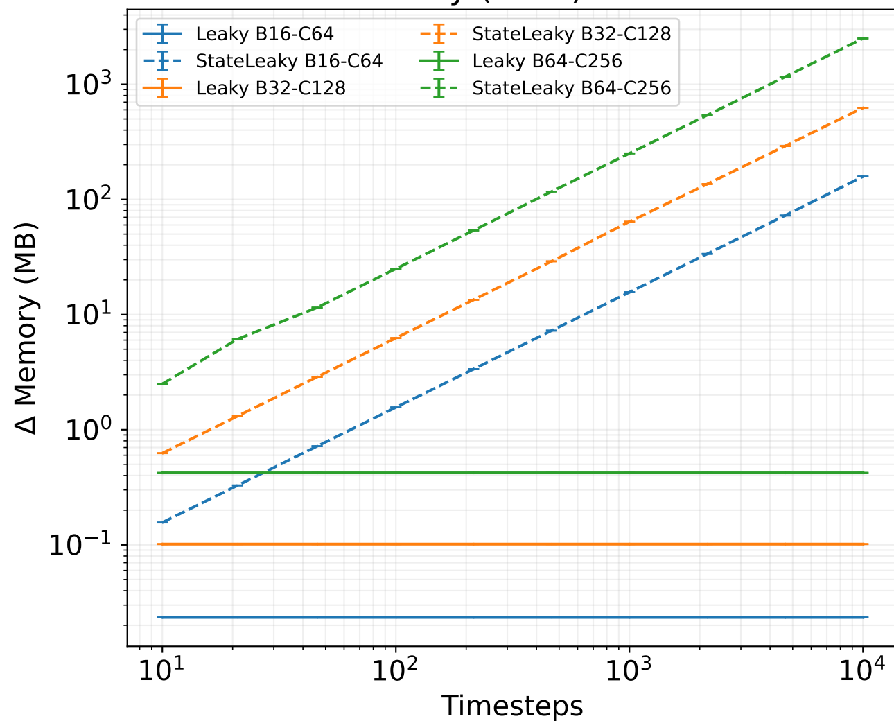
SNN Memory (Peak) - Inference
