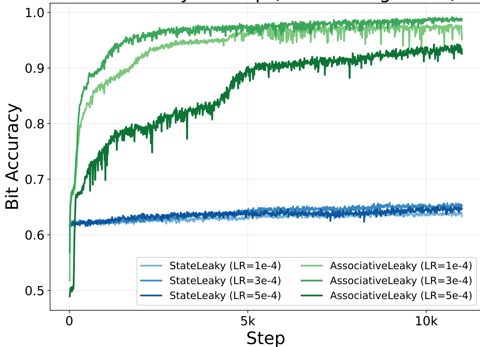
Bit Accuracy vs Step (All Learning Rates)
