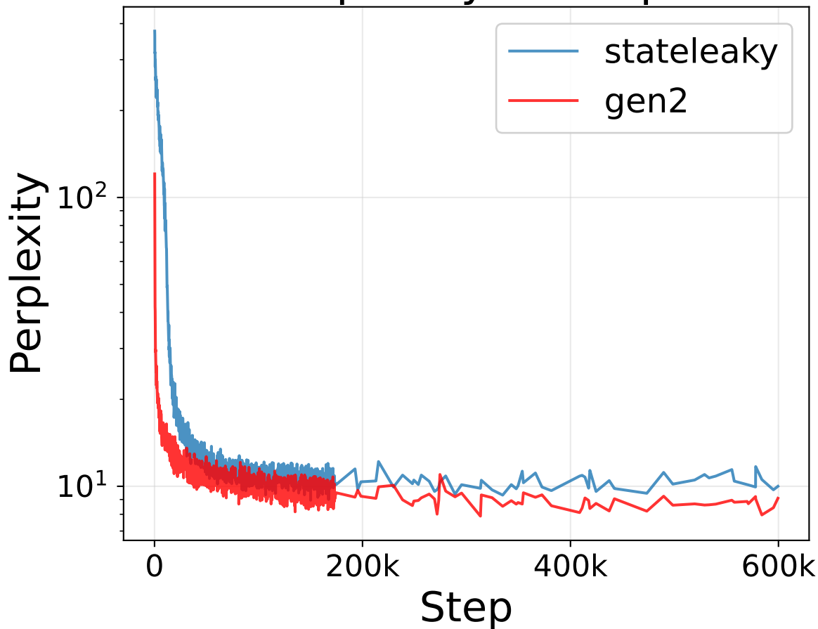
Perplexity vs Step
