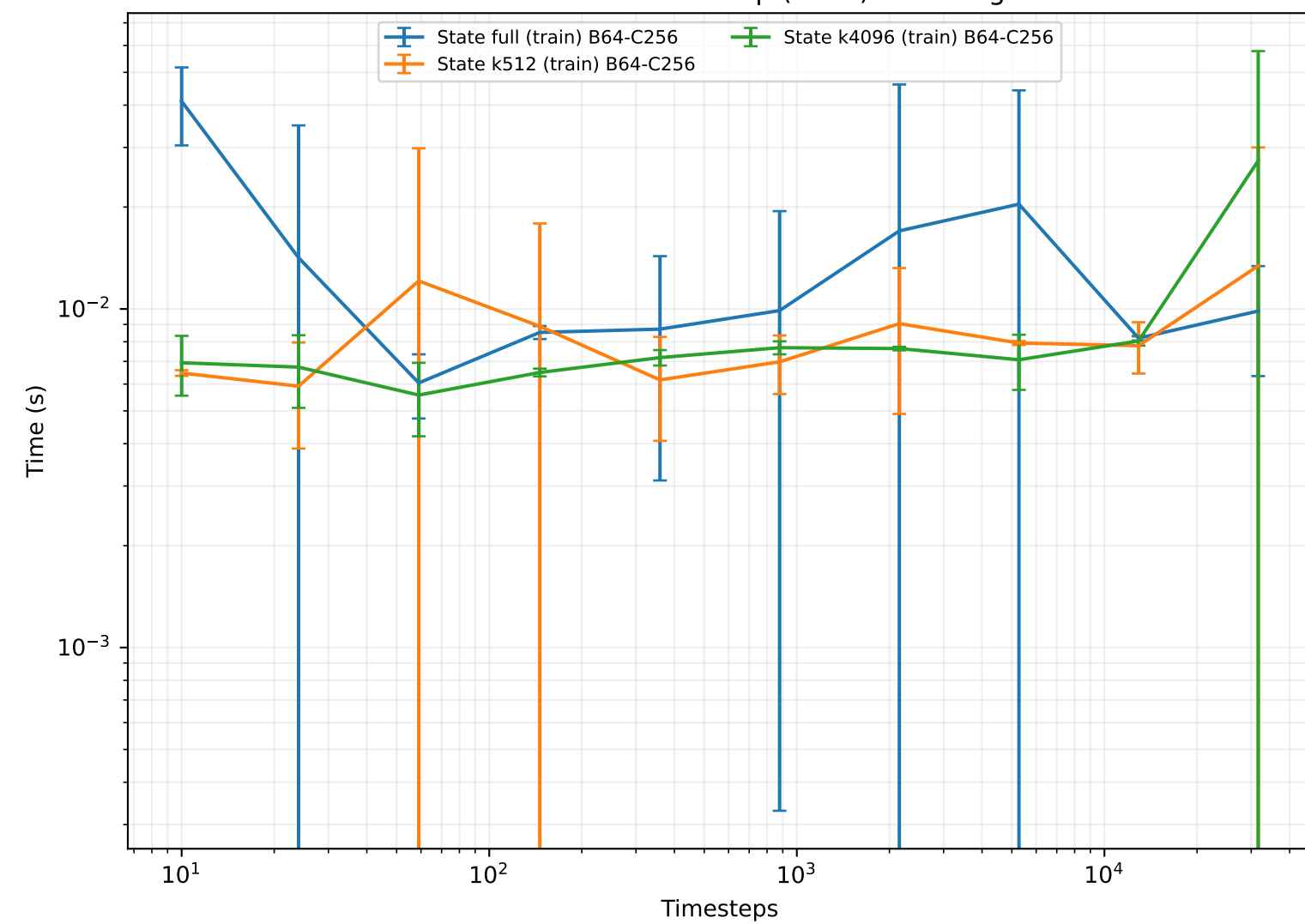
Kernel Truncation Sweep (Time) - Training
