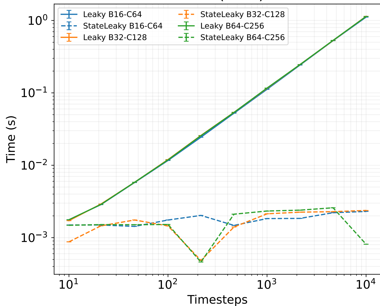
SNN Performance (Time) - Inference
