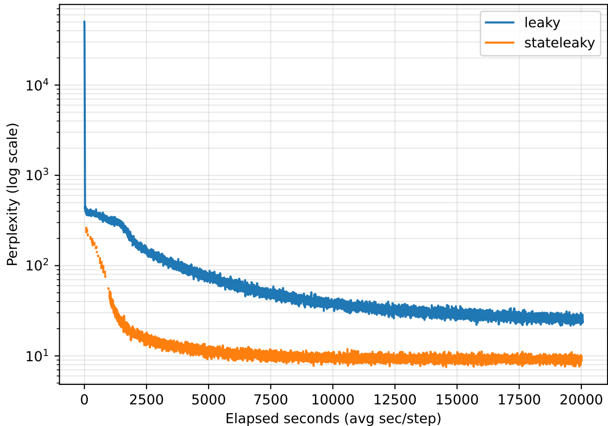
Perplexity vs Wall-Clock Time
