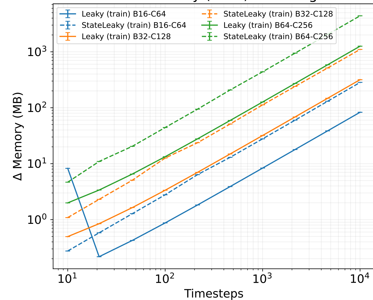
SNN Memory (Peak) - Training
