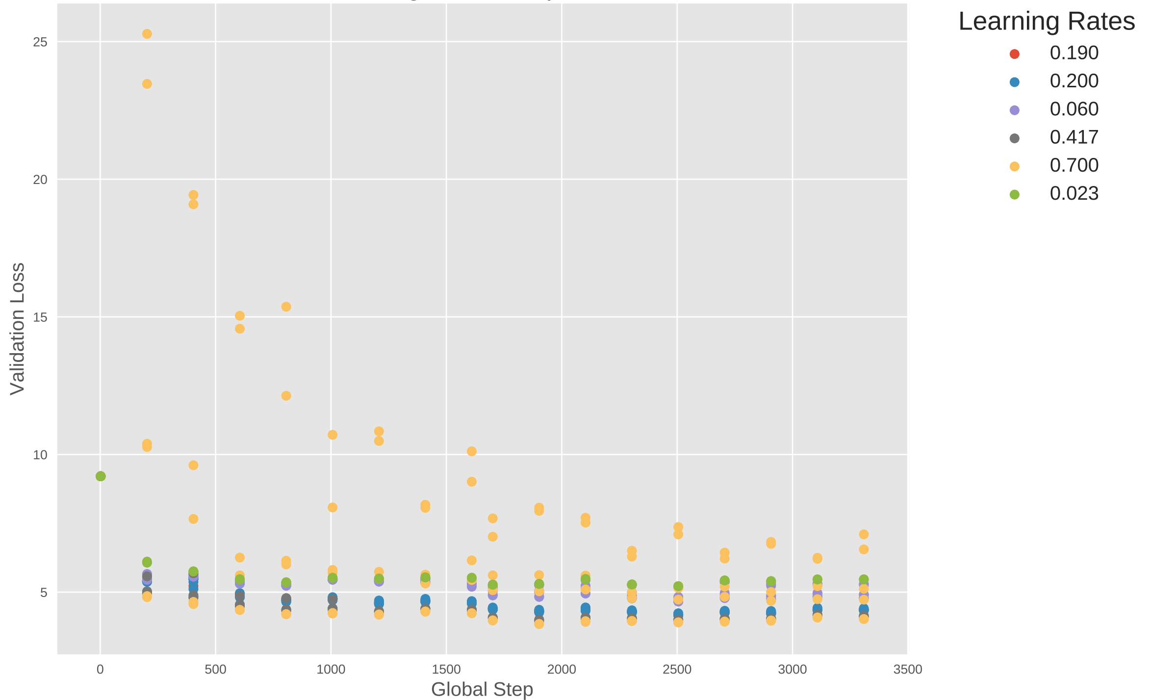
Learning Rate Comparisons
