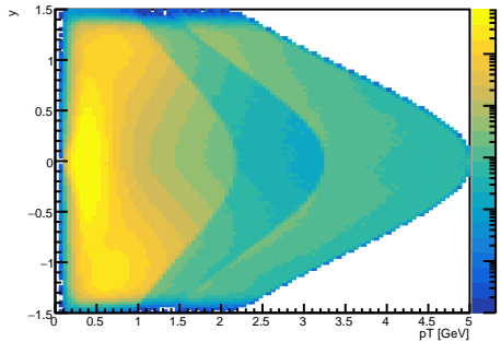
p^+ + p^- vs. p_T vs. rapidity
