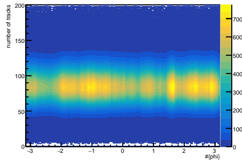
p^+ + p^- vs. \phi vs. nTracks
