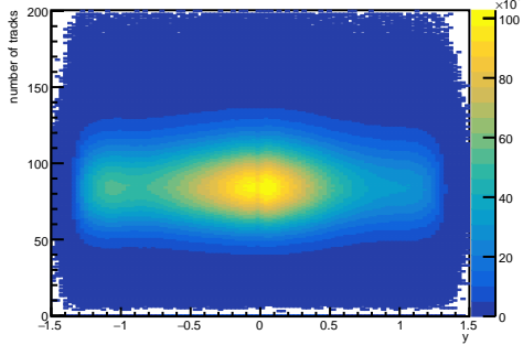
p^+ vs. rapidity vs. nTracks
