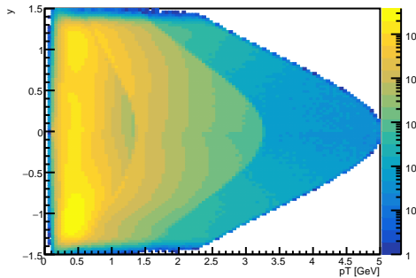
K + vs. pT vs. rapidity
