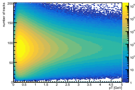
negatively-charged track vs. pT vs. nTracks
