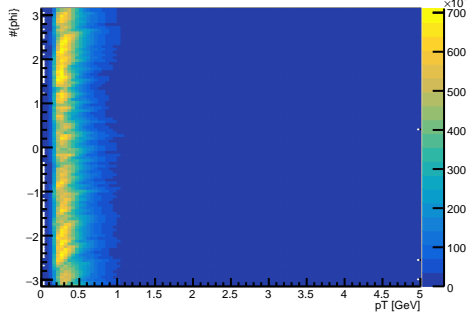
\pi^- vs. p_T vs. \phi
