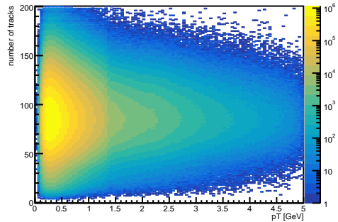
\pi^- vs. p_T vs. nTracks
