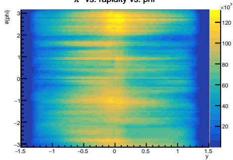
\pi^+ vs. rapidity vs. \phi
