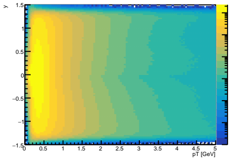
positively-charged track vs. pT vs. rapidity
