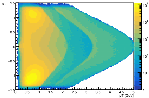
p^- vs. p_T vs. rapidity
