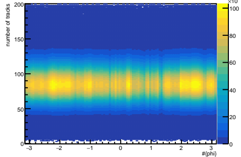
\pi^- vs. \phi vs. nTracks
