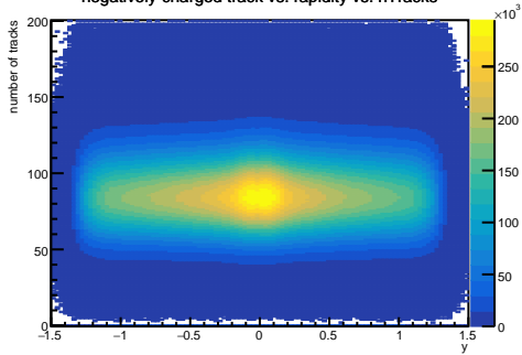
negatively-charged track vs. rapidity vs. nTracks
