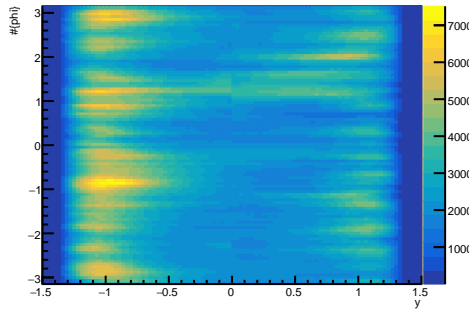
K^+ + K^- vs. rapidity vs. phi
