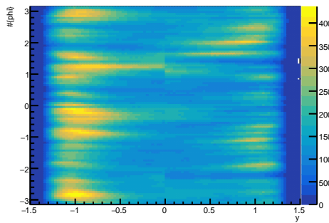
K + vs. rapidity vs. phi
