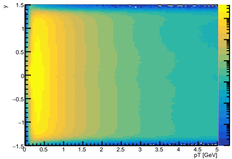
all tracks vs. pT vs. rapidity
