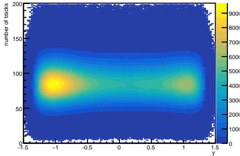
K^+ + K^- vs. rapidity vs. nTracks
