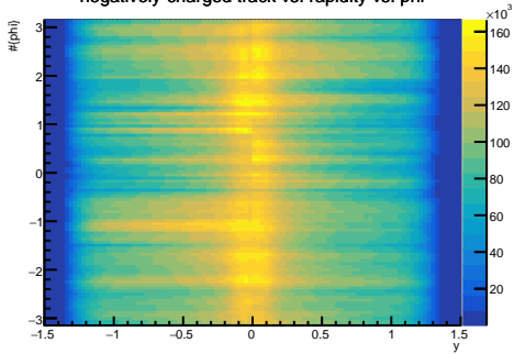
negatively-charged track vs. rapidity vs. phi
