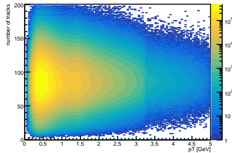
K^+ + K^- vs. pT vs. nTracks
