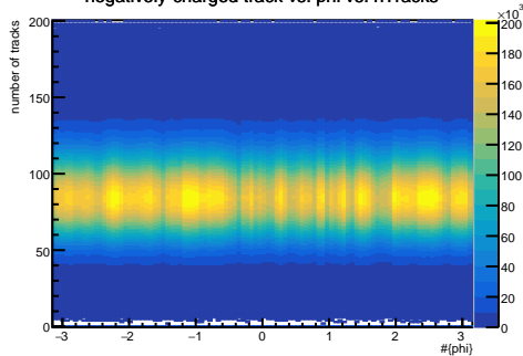
negatively-charged track vs. phi vs. nTracks
