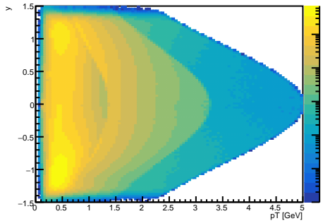
K^+ + K^- vs. pT vs. rapidity
