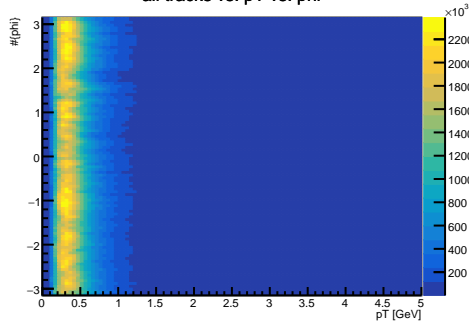
all tracks vs. pT vs. phi
