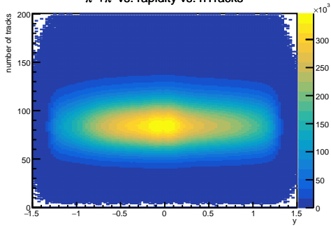
\pi^+\pi^- vs. rapidity vs. nTracks
