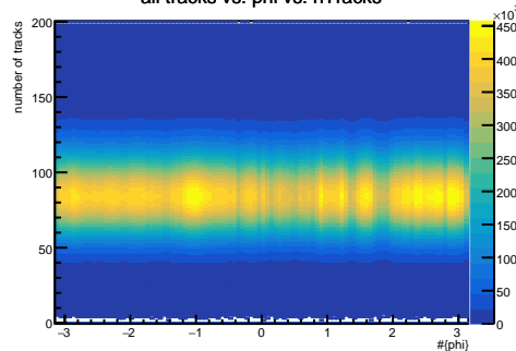
all tracks vs. phi vs. nTracks
