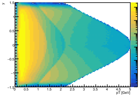
\pi^+\pi^- vs. p_T vs. rapidity
