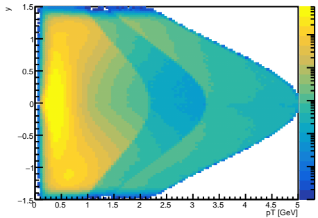
p^+ vs. p_T vs. rapidity
