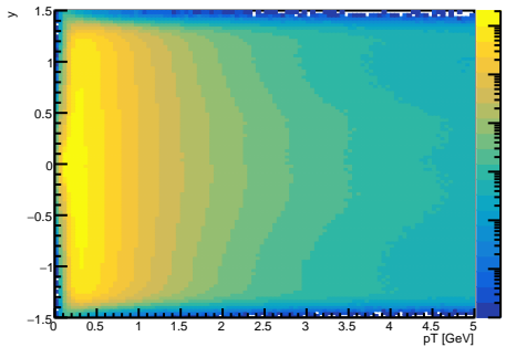
negatively-charged track vs. pT vs. rapidity
