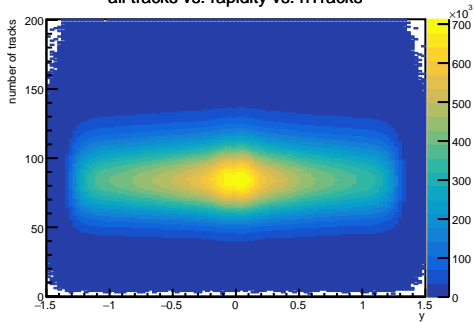
all tracks vs. rapidity vs. nTracks
