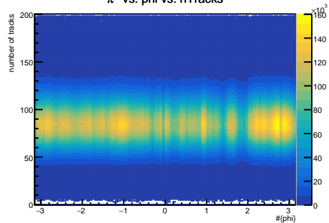
\pi^+ vs. \phi vs. nTracks
