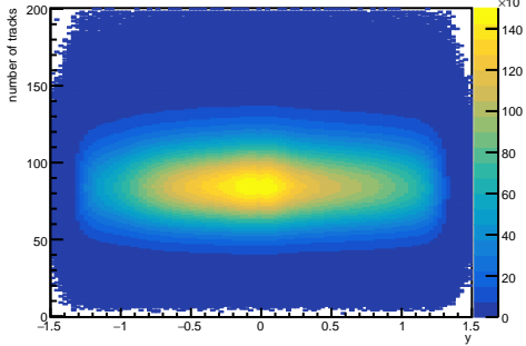
\pi^- vs. rapidity vs. nTracks
