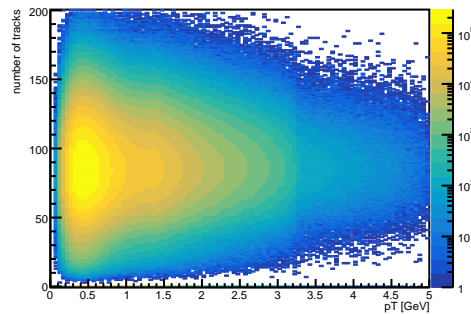
K + vs. pT vs. nTracks
