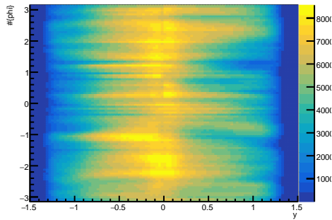
\pi^- vs. rapidity vs. \phi
