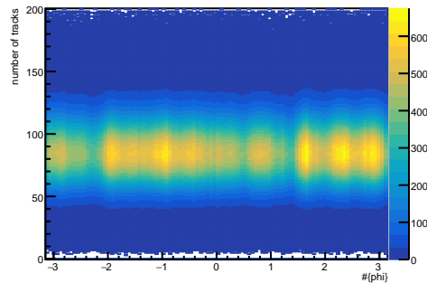
p^+ vs. \phi vs. nTracks
