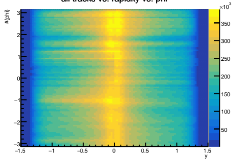
all tracks vs. rapidity vs. phi
