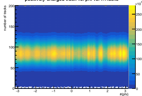
positively-charged track vs. phi vs. nTracks
