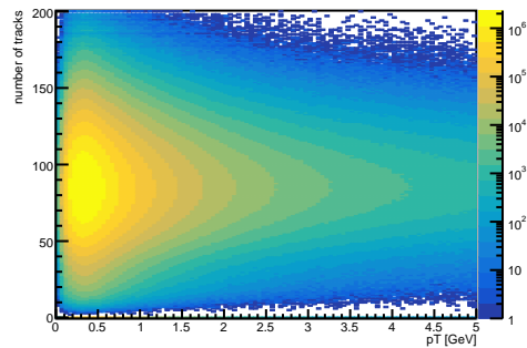
positively-charged track vs. pT vs. nTracks
