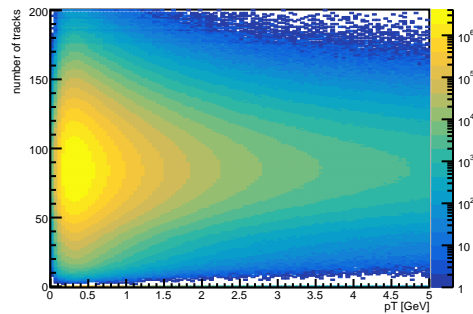
all tracks vs. pT vs. nTracks
