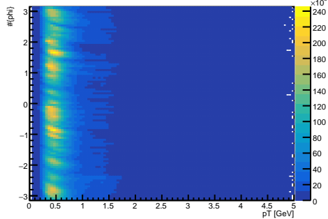
K + vs. pT vs. phi
