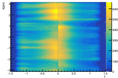
p^+ vs. rapidity vs. \phi
