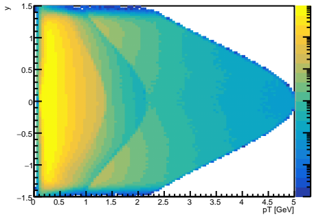
\pi^- vs. p_T vs. rapidity
