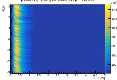
positively-charged track vs. pT vs. phi
