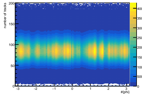
K + vs. phi vs. nTracks
