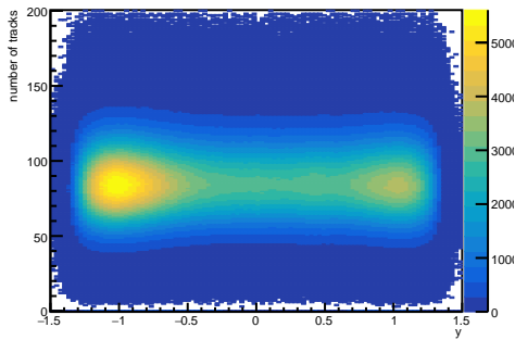
K + vs. rapidity vs. nTracks
