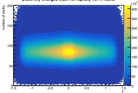
positively-charged track vs. rapidity vs. nTracks
