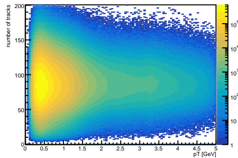
p^+ vs. p_T vs. nTracks
