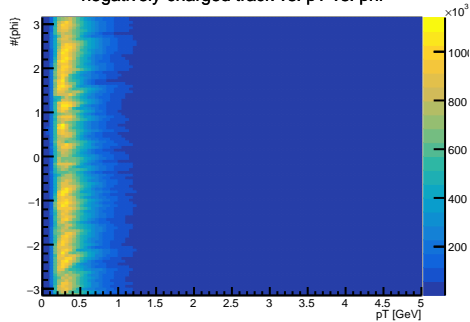
negatively-charged track vs. pT vs. phi
