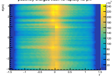
positively-charged track vs. rapidity vs. phi
