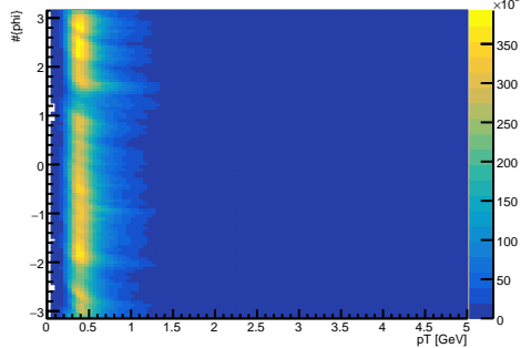
p^+ vs. p_T vs. \phi
