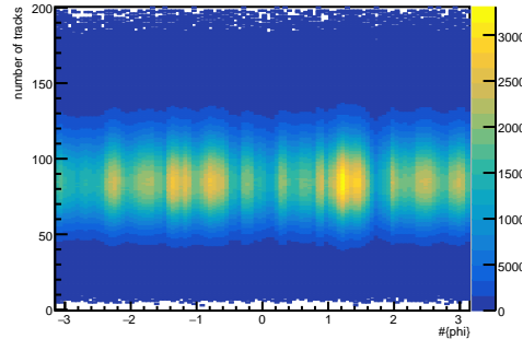
K^- vs. phi vs. nTracks
