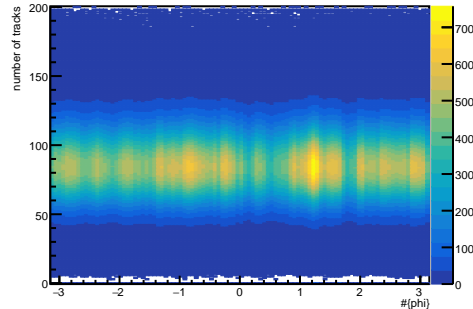
K^+ + K^- vs. phi vs. nTracks
