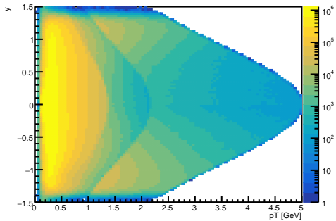
\pi^+ vs. p_T vs. rapidity
