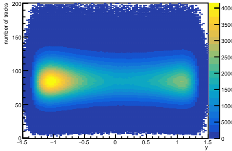
K^- vs. rapidity vs. nTracks
