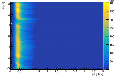
p^+ + p^- vs. p_T vs. \phi
