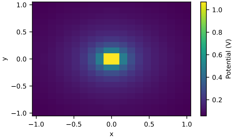
Electric Potential from Point Current in a Wholespace
