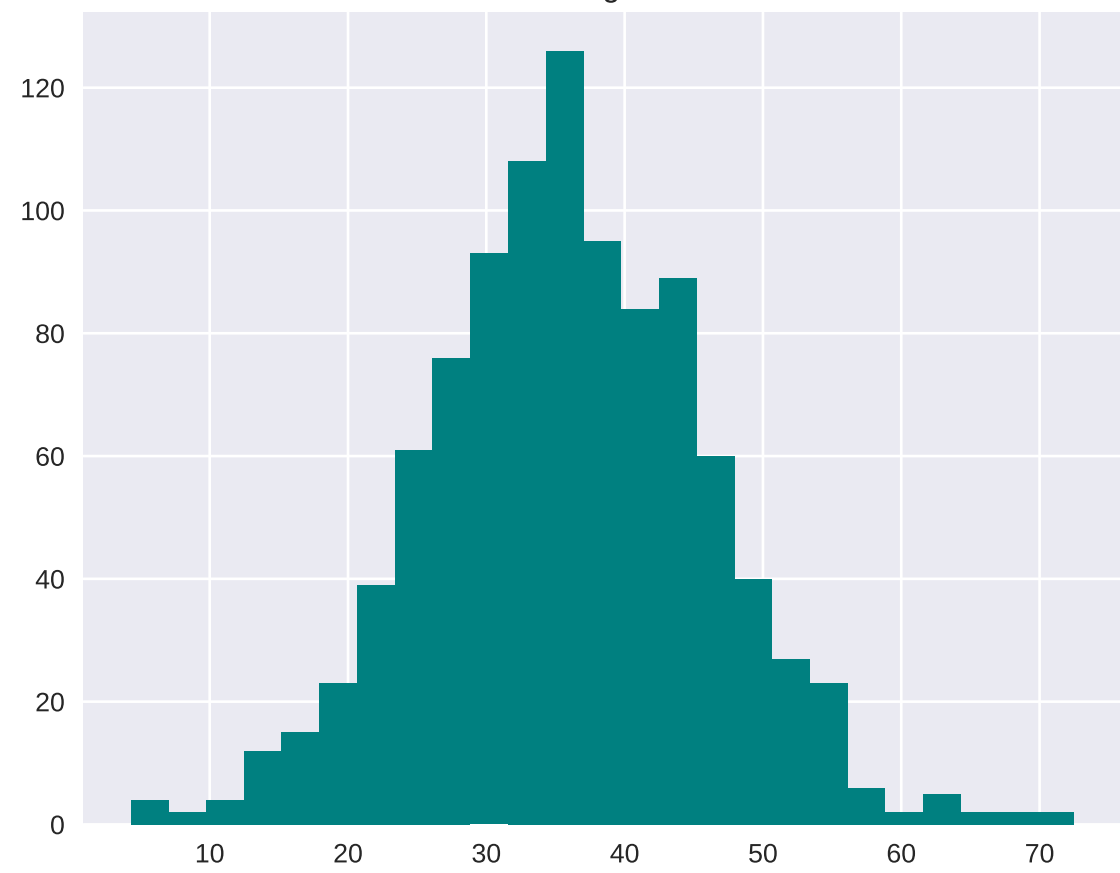
Histogram
