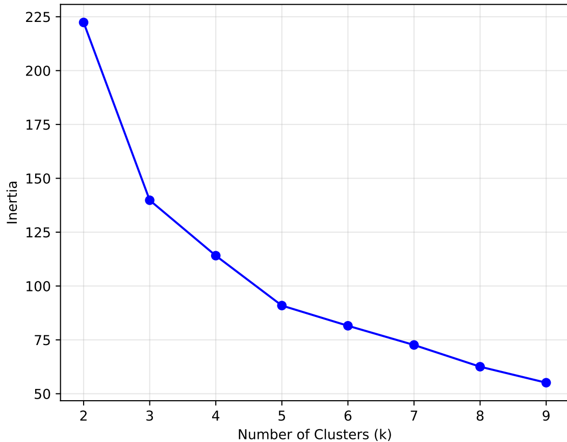
Elbow Method
