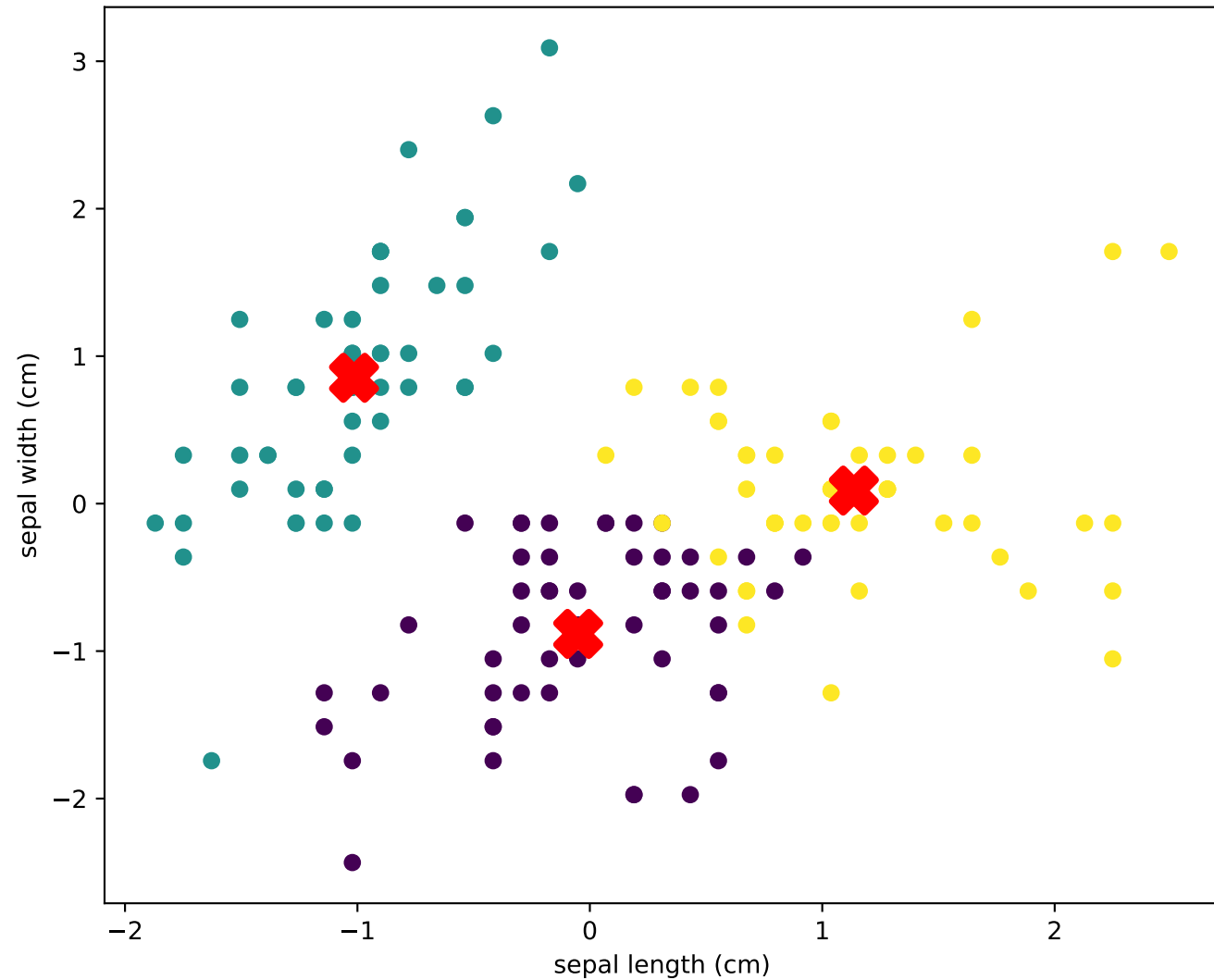
K-Means Predicted Clusters
