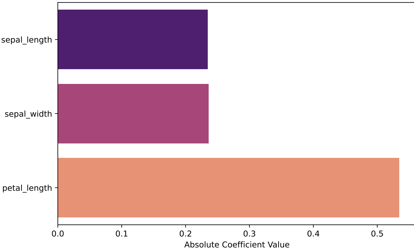
Feature Importance in Multiple Regression
