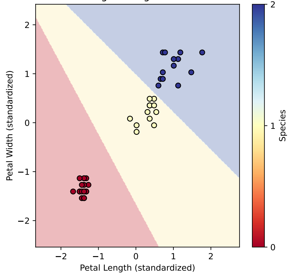
Logistic Regression
