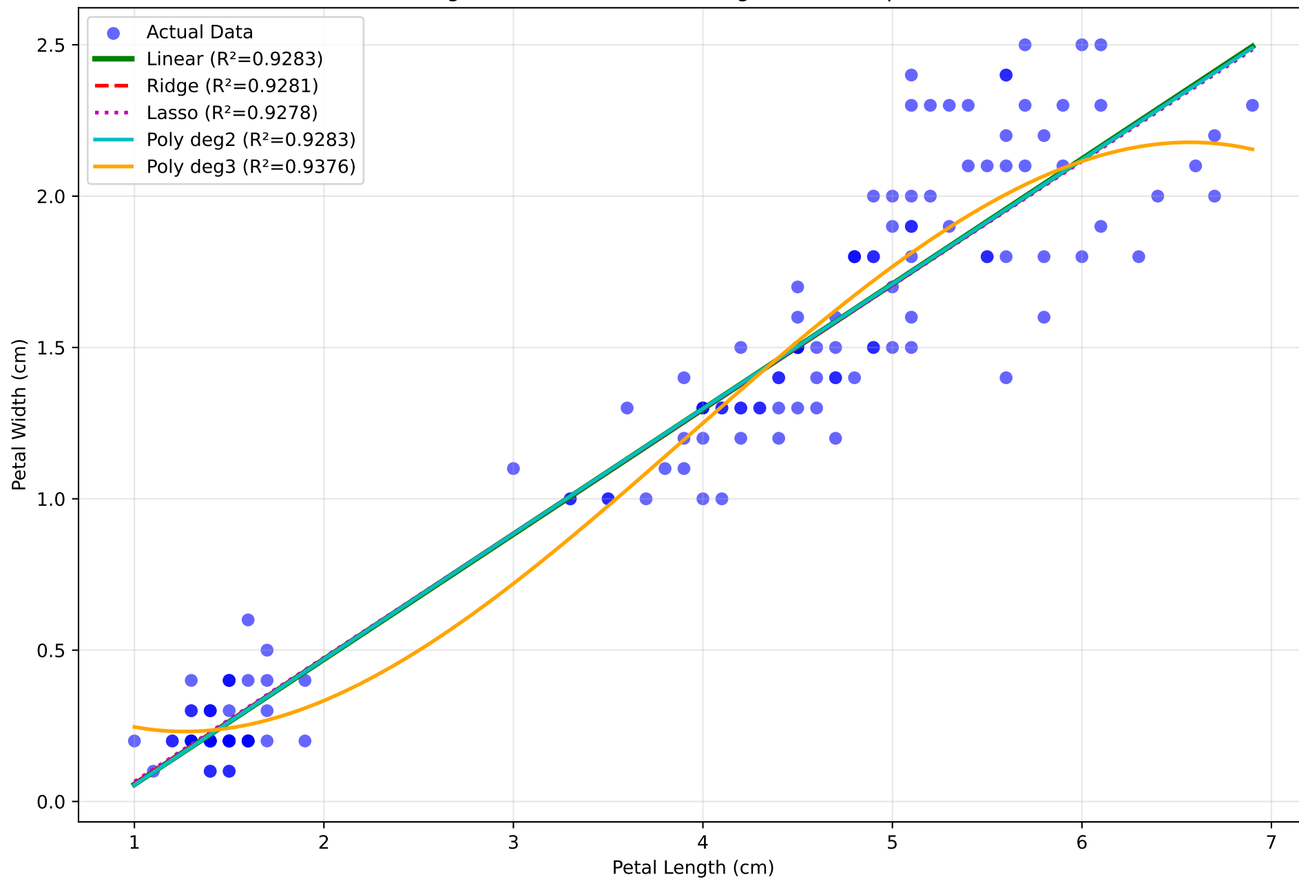
Regularized + Non-Linear Regression Comparison
