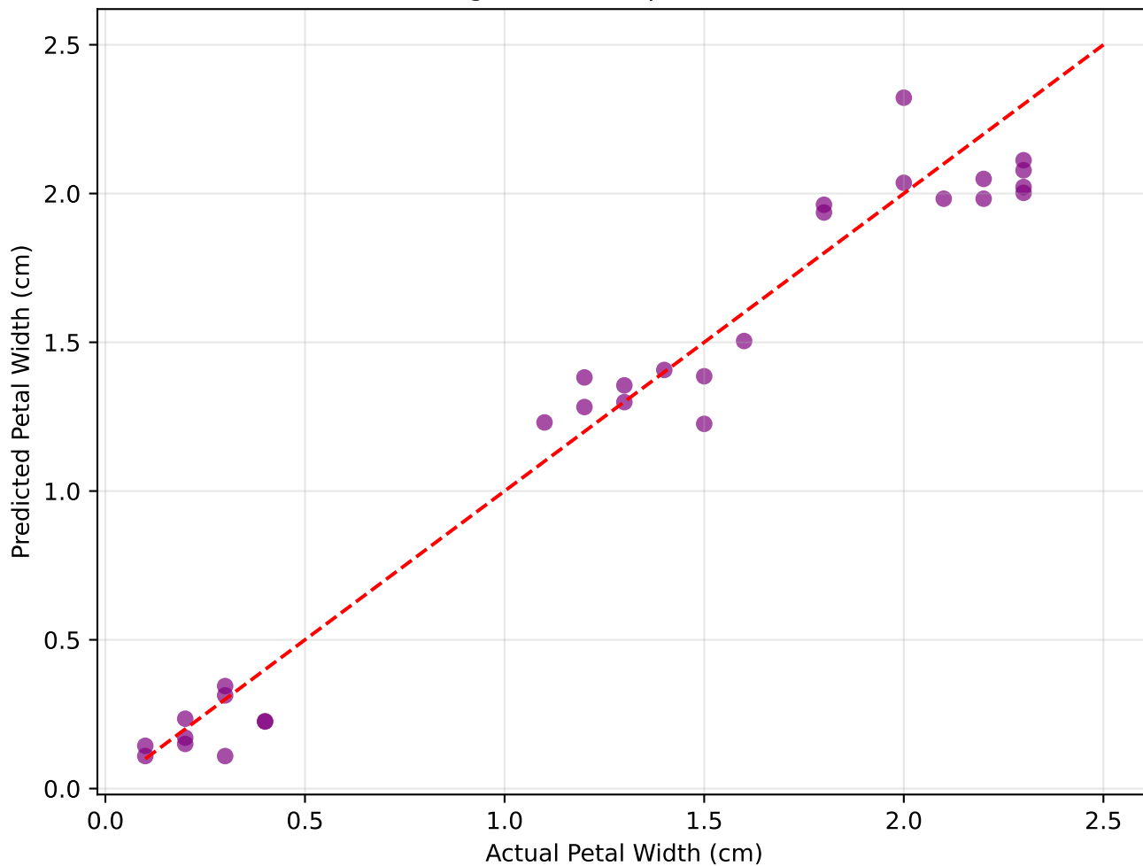
Linear Regression on Iris (Missing Values + Species Included)
