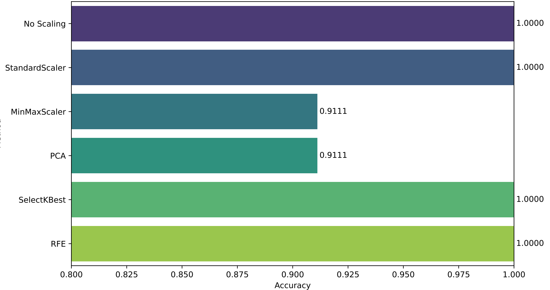
Feature Scaling & Selection Comparison on Iris
