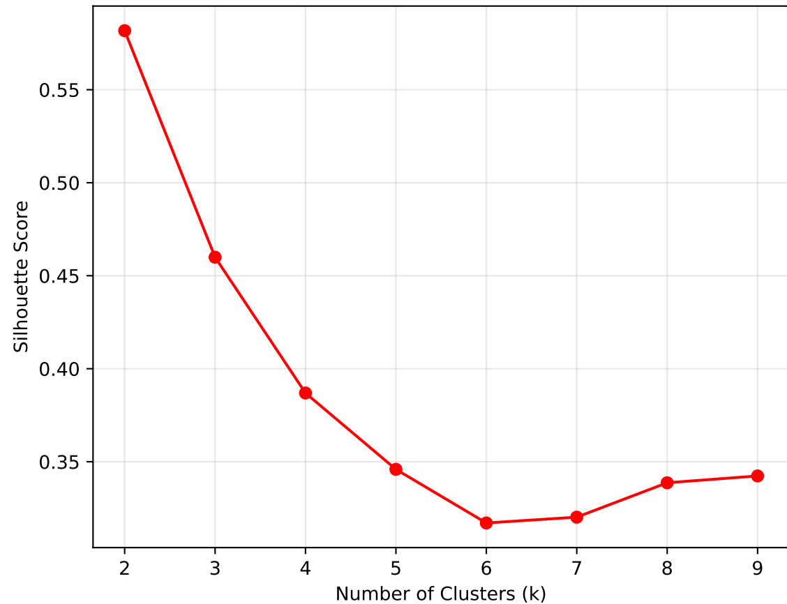
Silhouette Score
