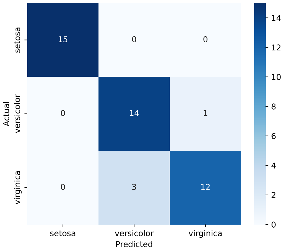
Confusion Matrix - Naive Bayes
