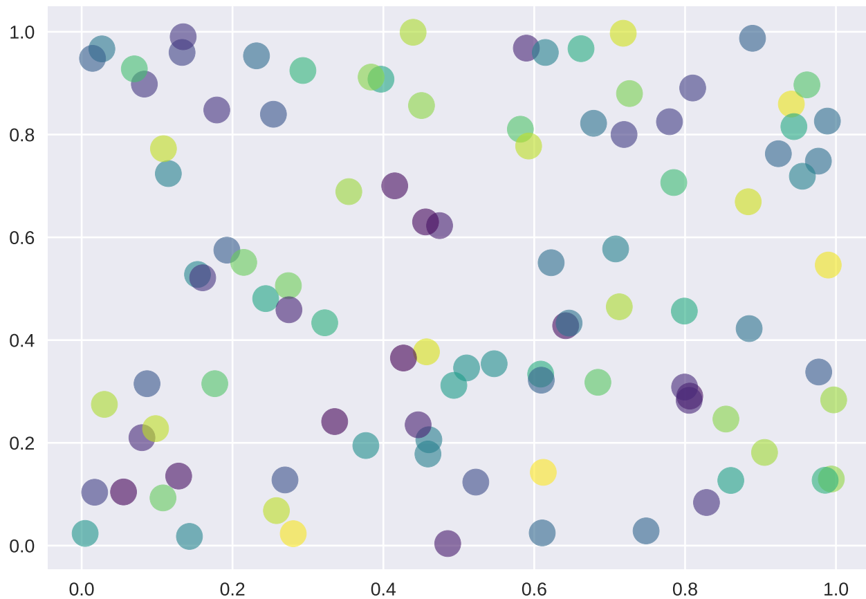
Scatter Plot
