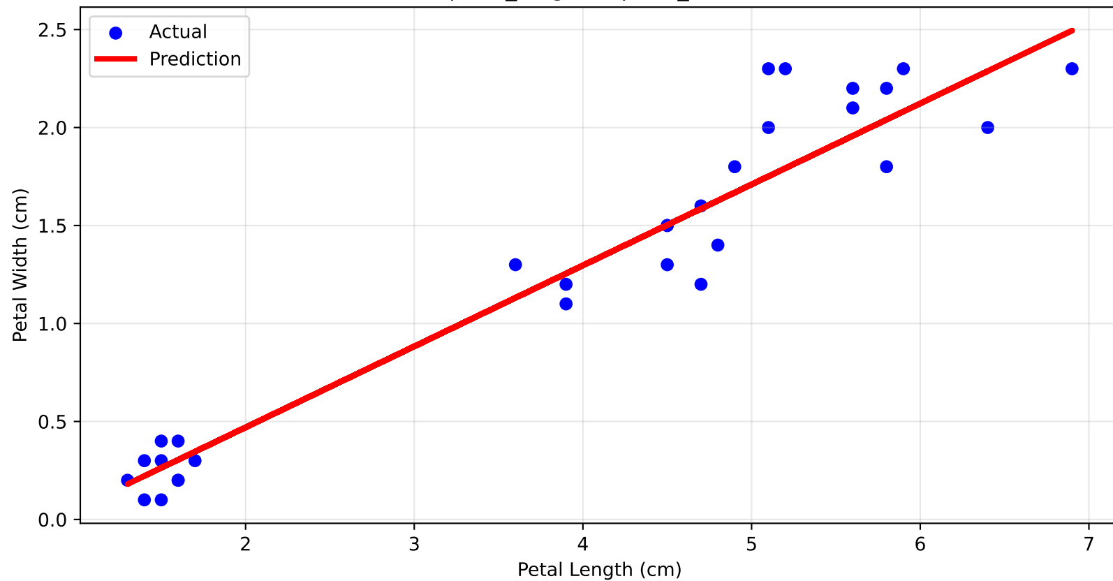
Simple Linear Regression (petal_length \rightarrow petal_width)
