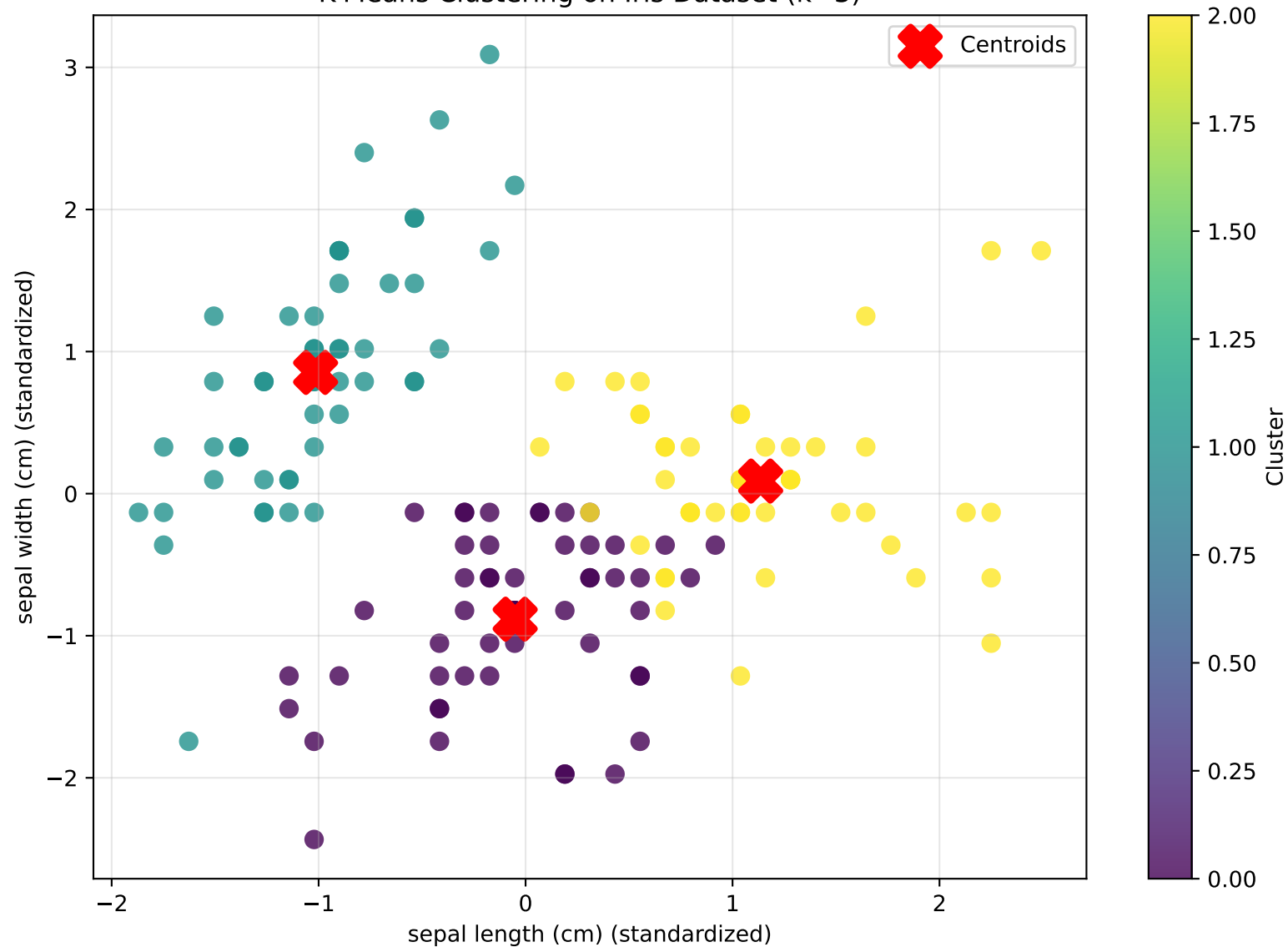
K-Means Clustering on Iris Dataset (k=3)
