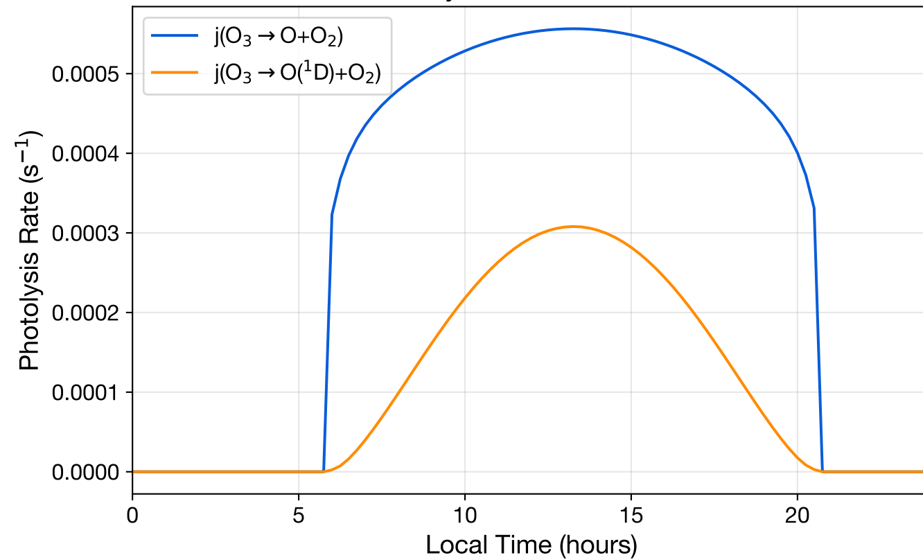
Photolysis Rates at 30 km
