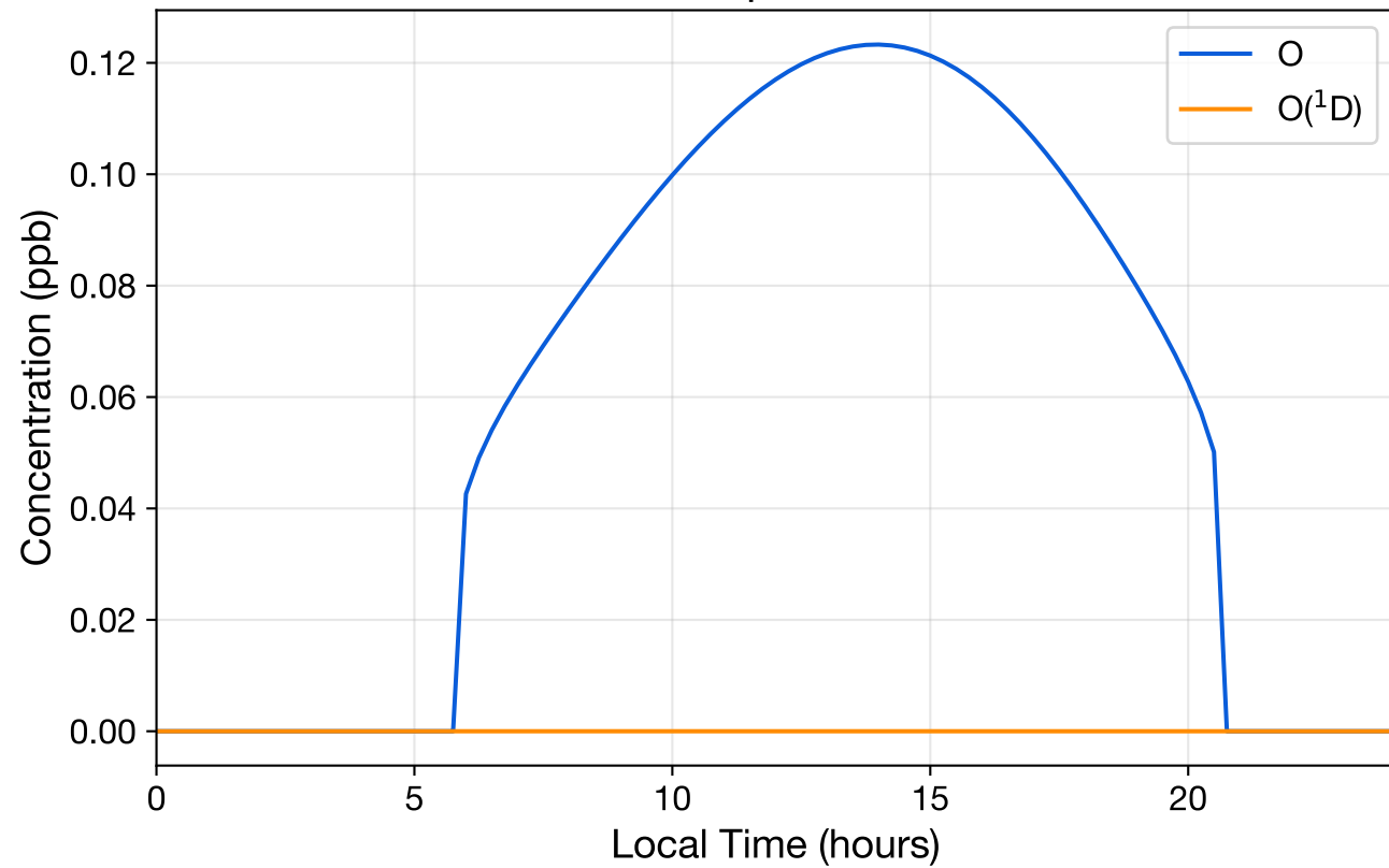
Short-lived Species at 30 km
