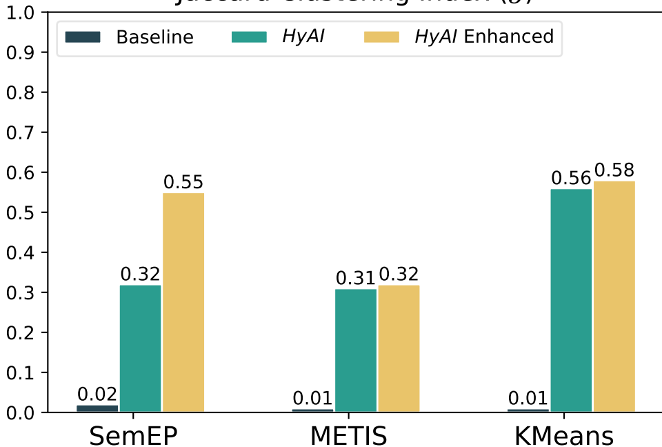
Jaccard Clustering Index ( \mathcal{J} )
