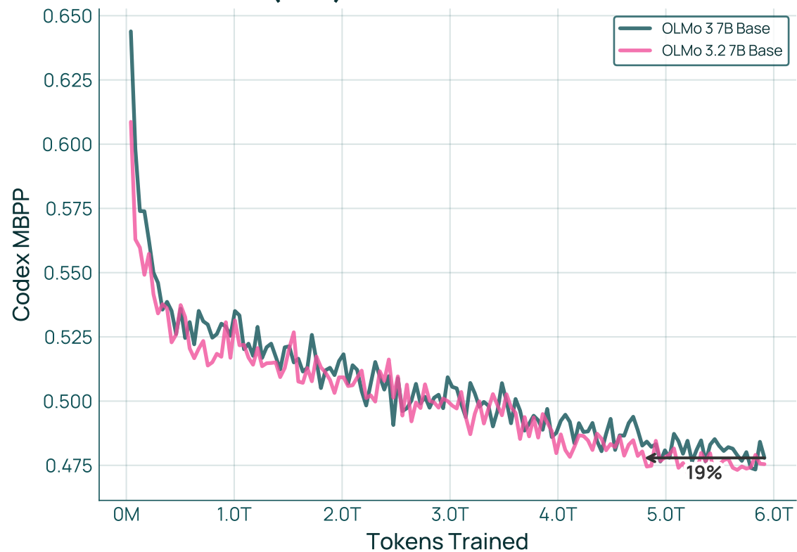
Codex MBPP (BPB)
