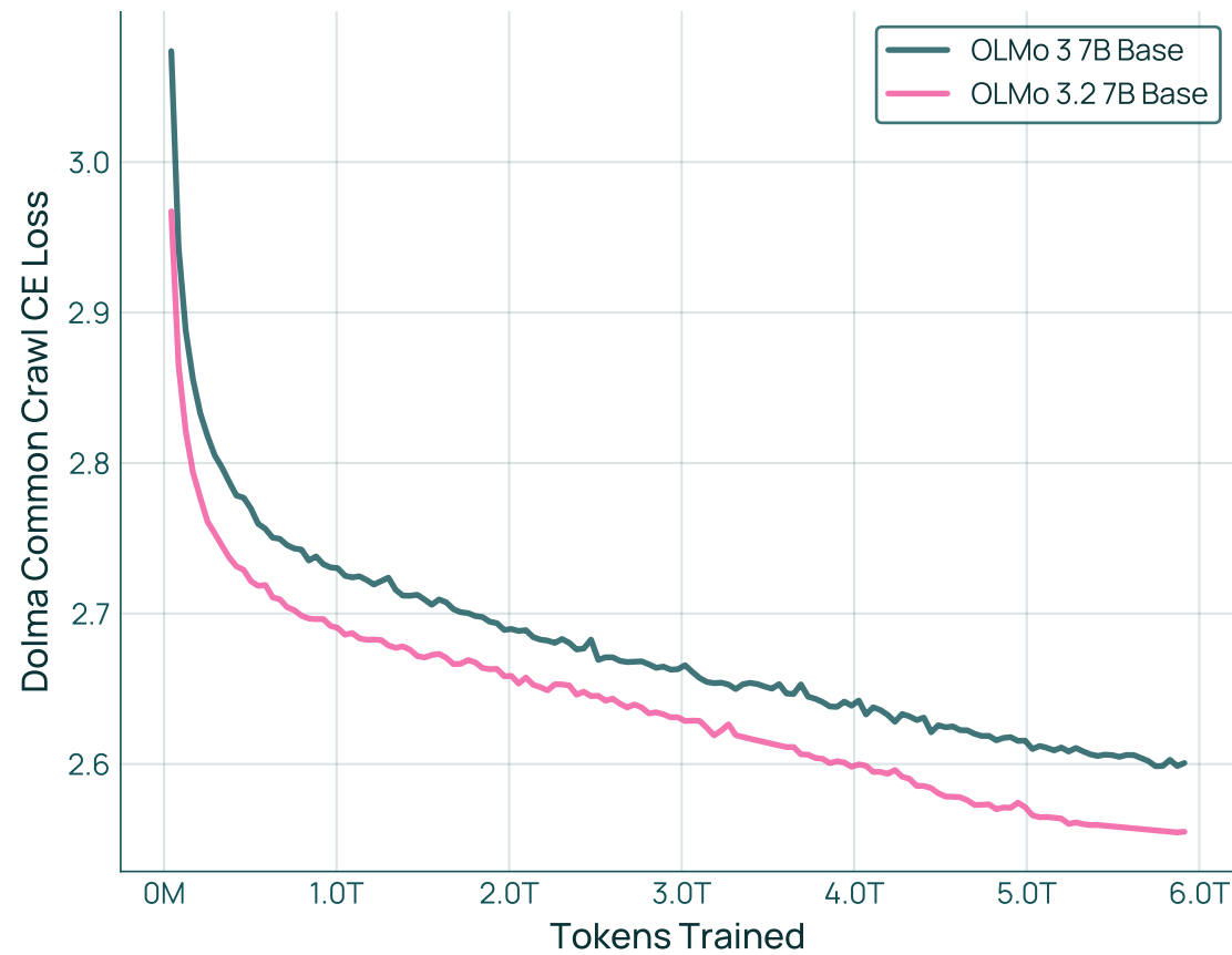
Dolma Common Crawl CE Loss
