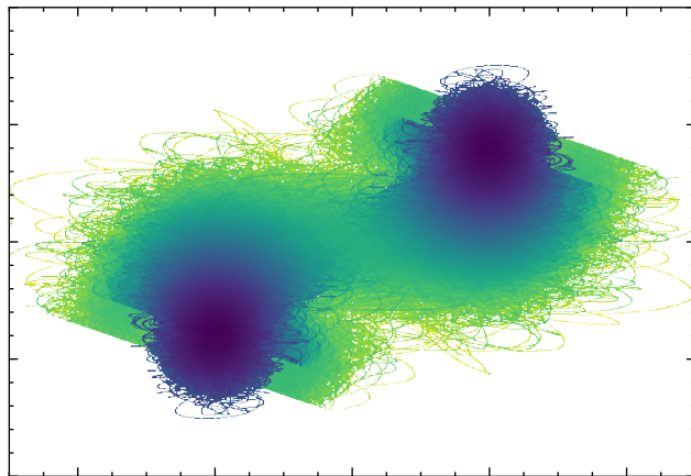
Committor Surface
