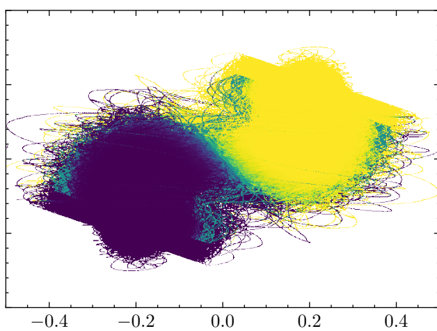
Committor Surface
