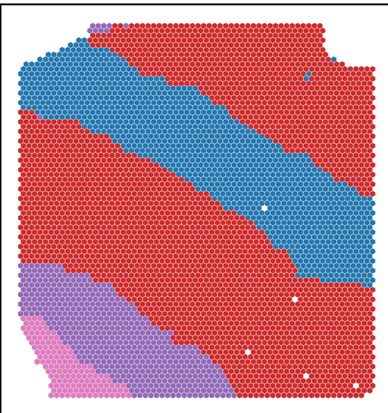
K = 4
