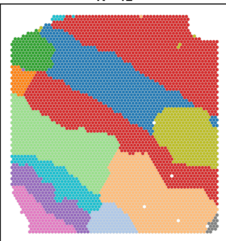
K = 12
