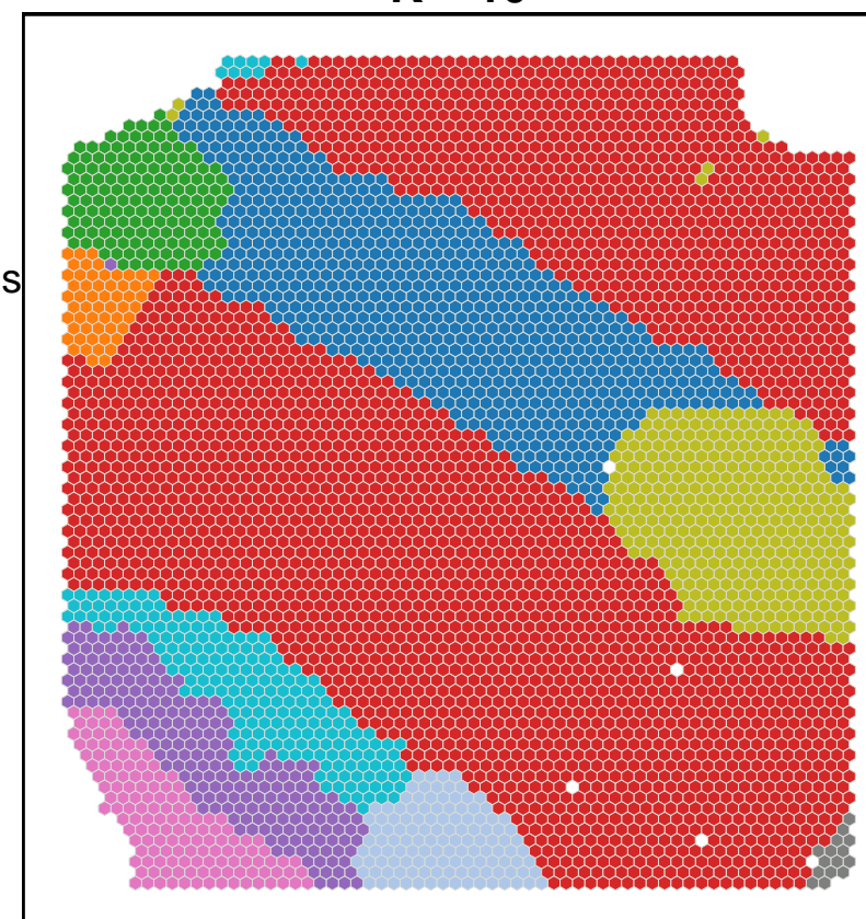
K = 10
