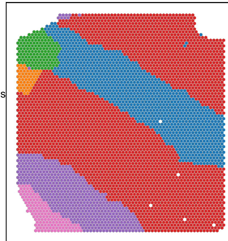
K = 6
