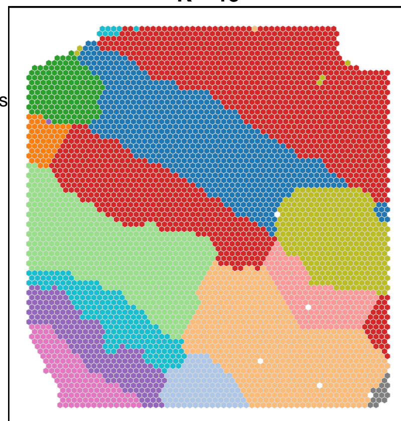
K = 13
