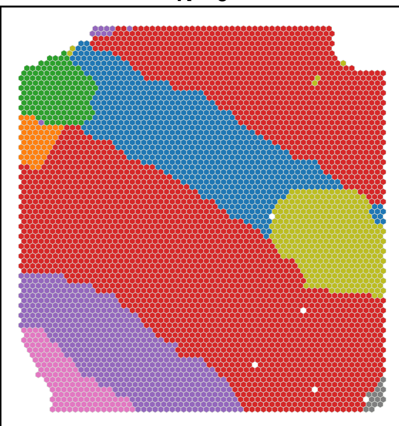
K = 8
