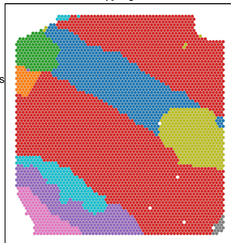
K = 9
