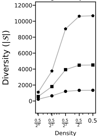
5 base binary relations and a target ternary relation
