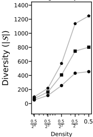
5 base binary relations and a target binary relation
