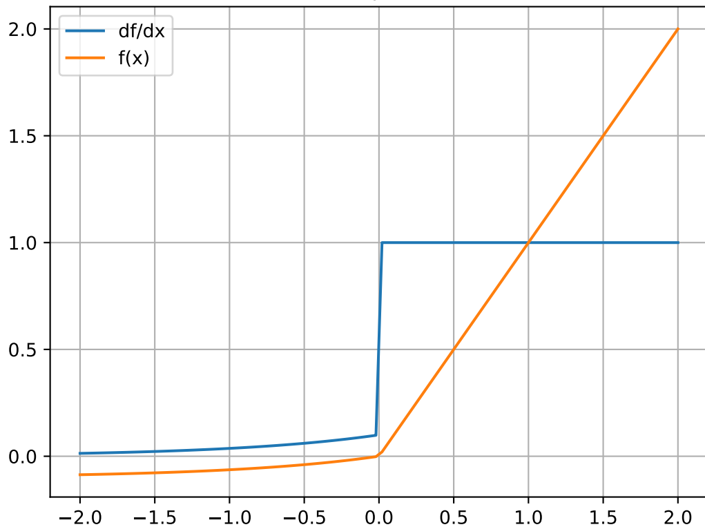
elu(x, alpha=0.1)
