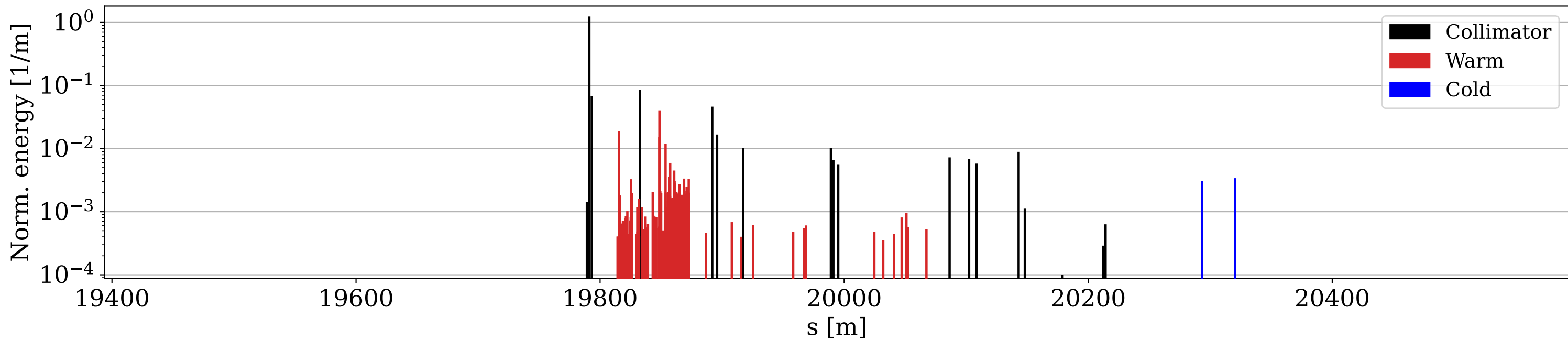
Zoom on betatron insertion
