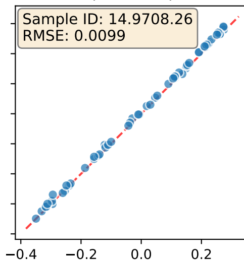
Prediction vs. True (Masked)
