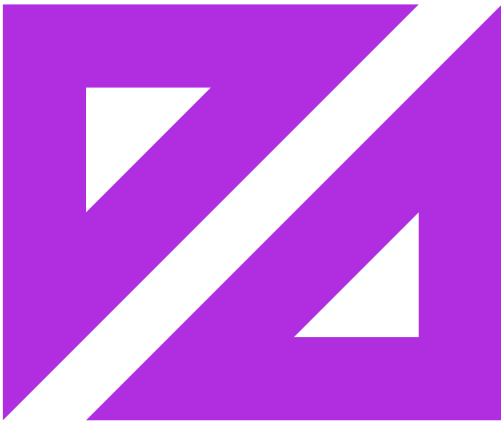
GeometryCollection
