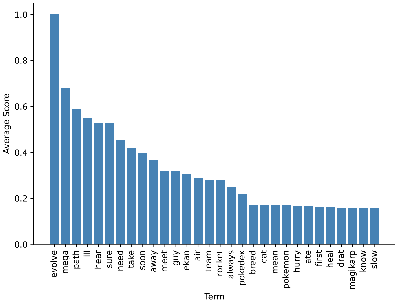
Bar plot of average TF-IDF score for top 30 terms
