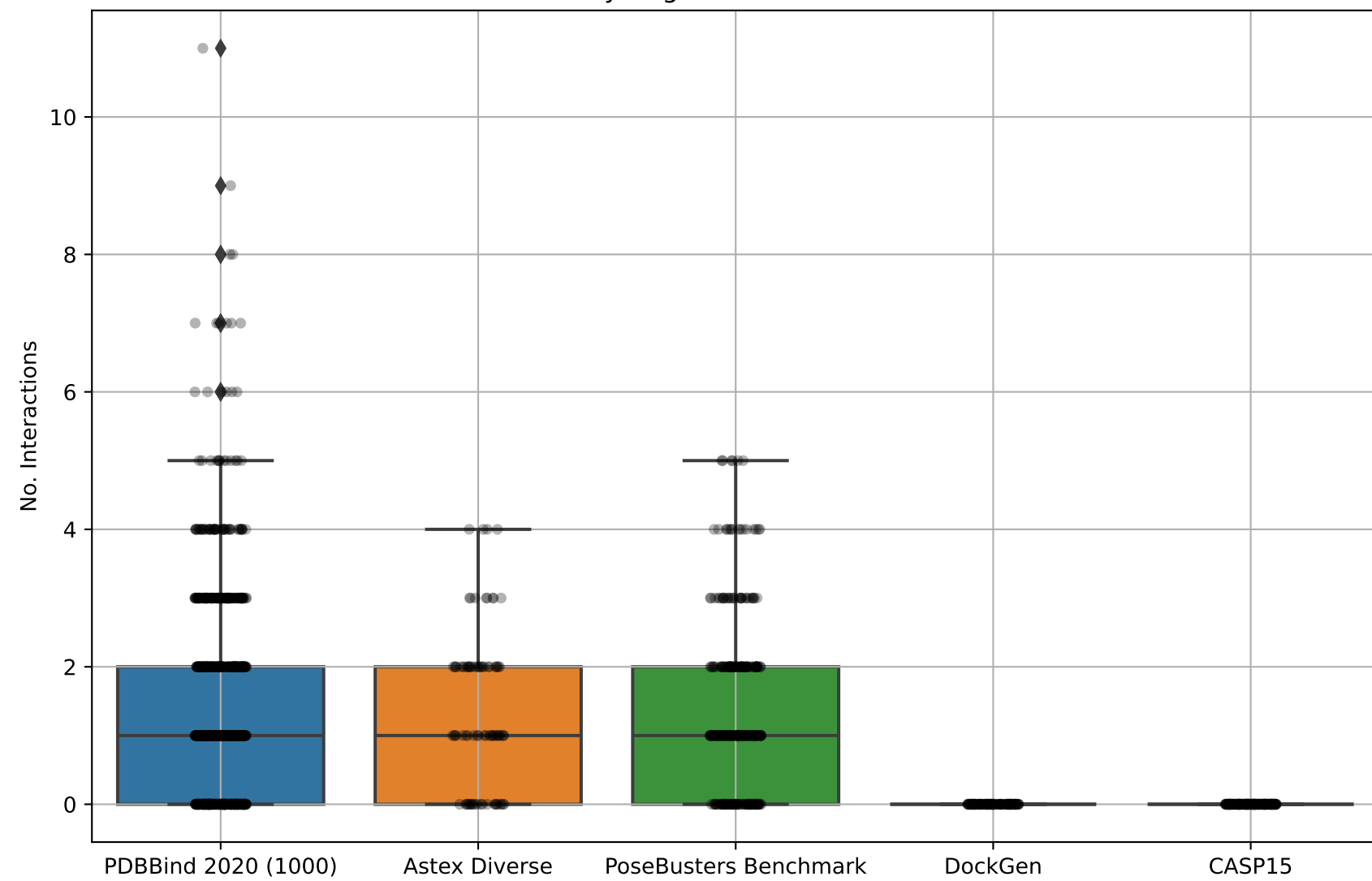
Hydrophobic Interactions
