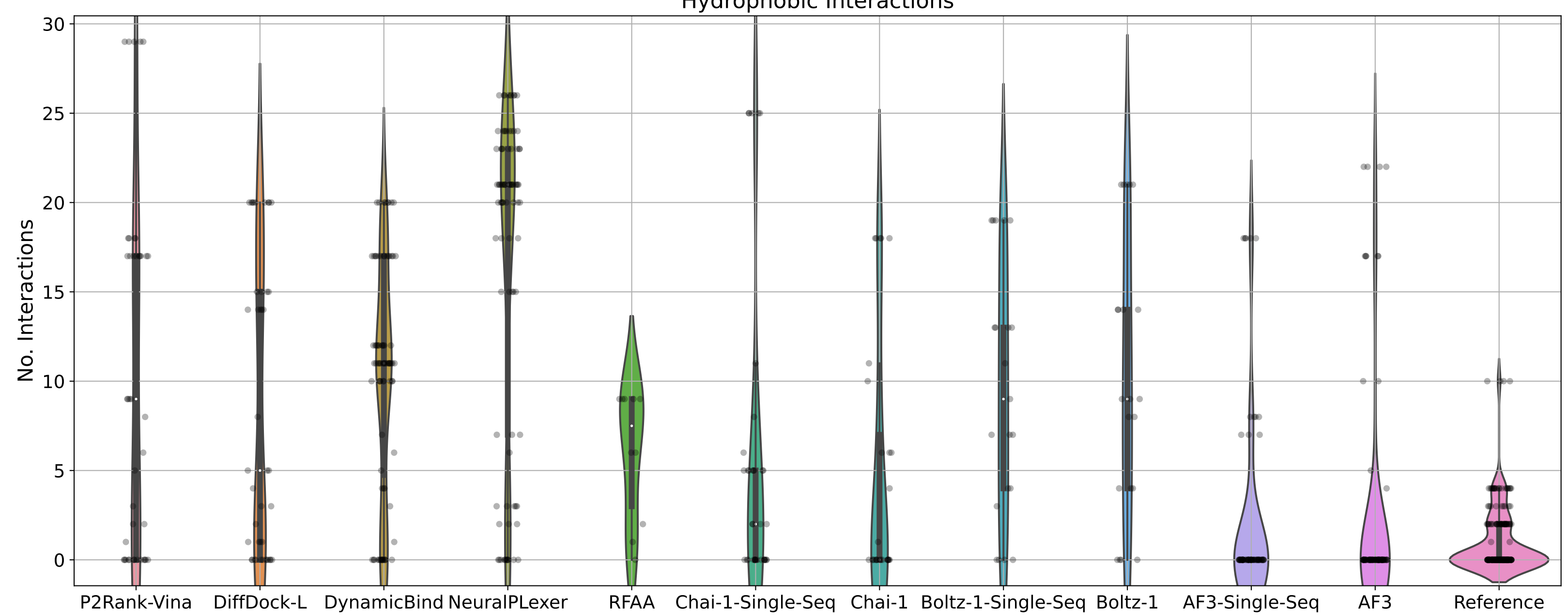
Hydrophobic Interactions
