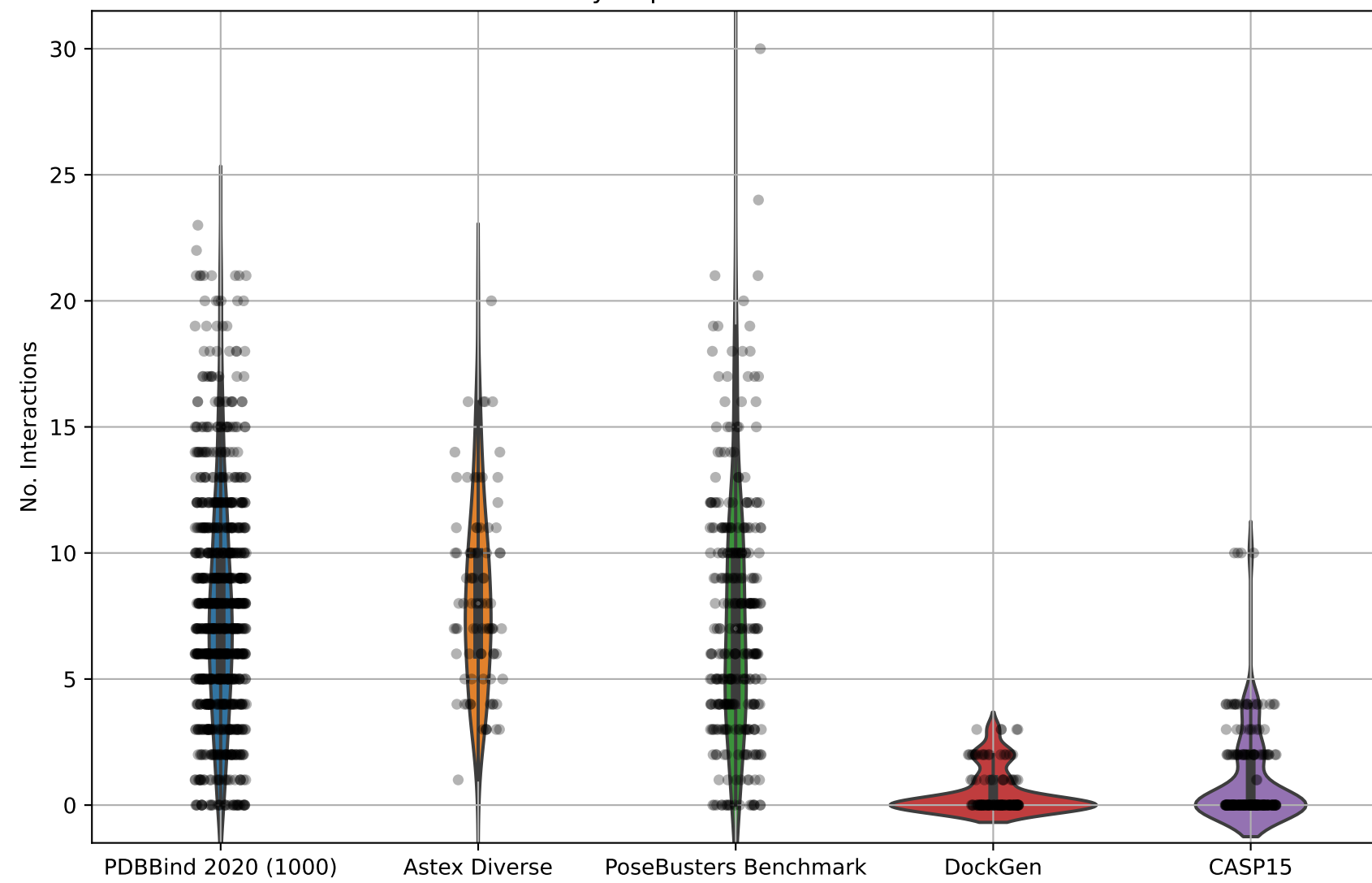
Hydrophobic Interactions
