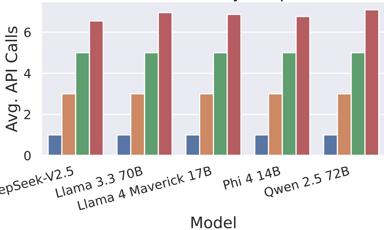
Dataset: dailylifeapis
