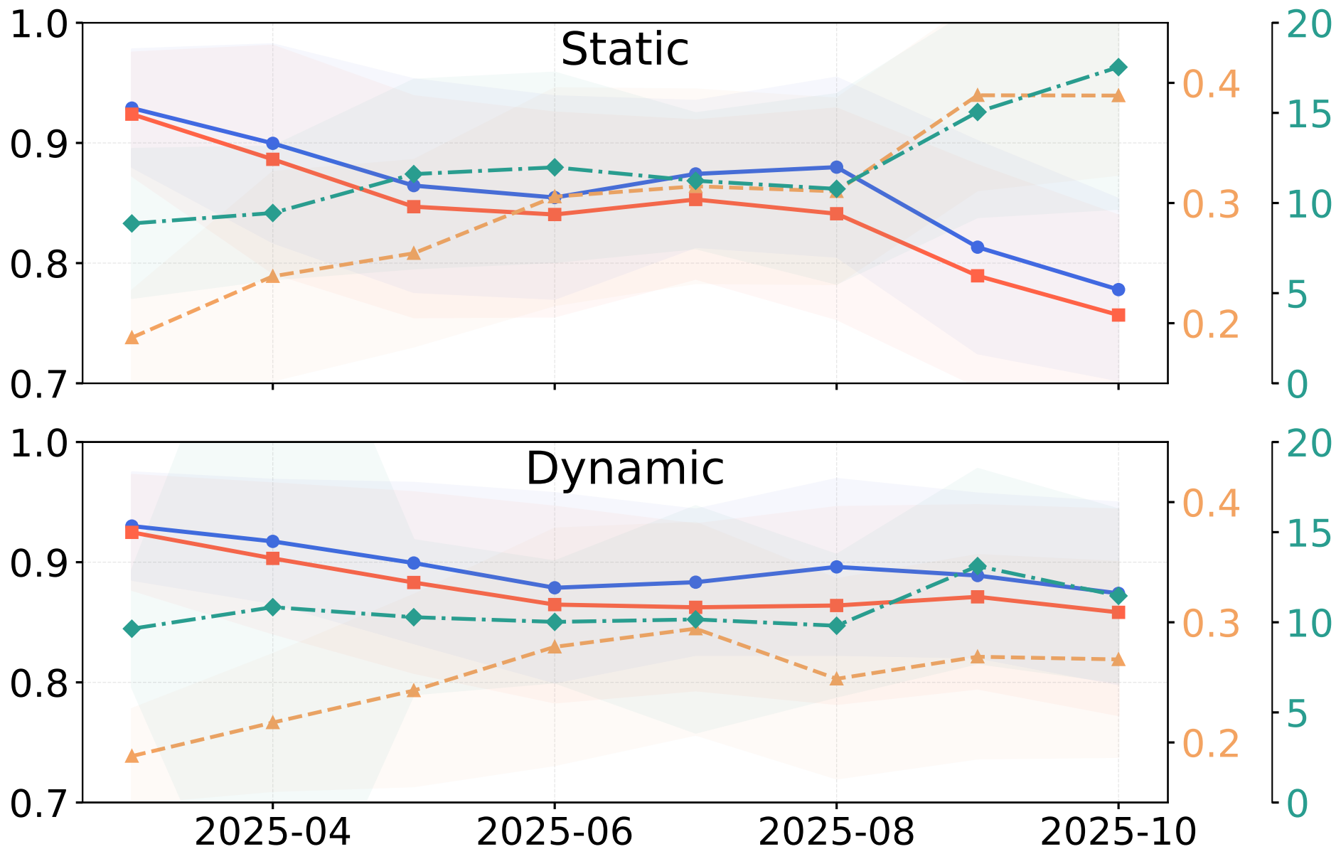
Model Performance
