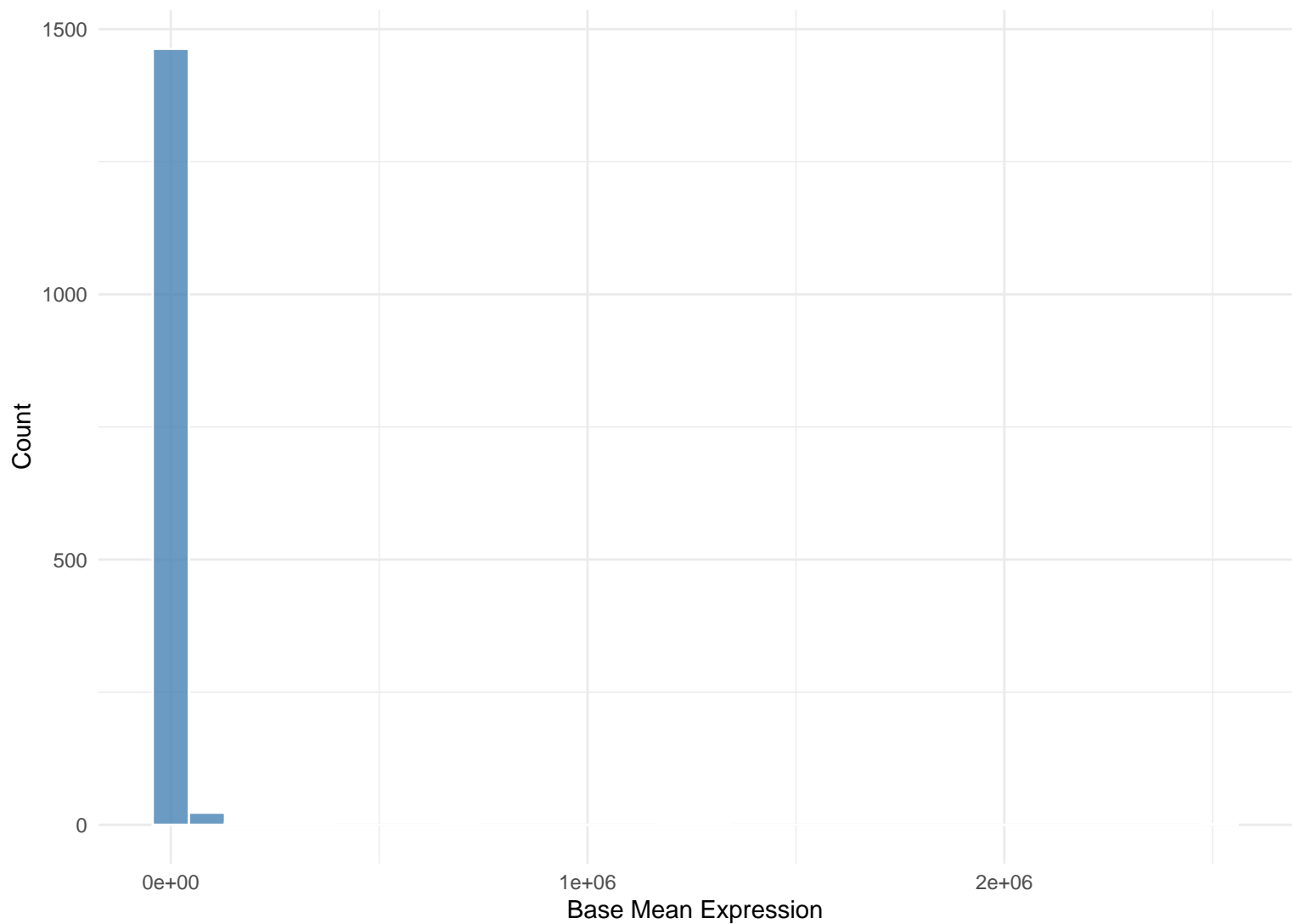
Distribution of Base Mean Expression
