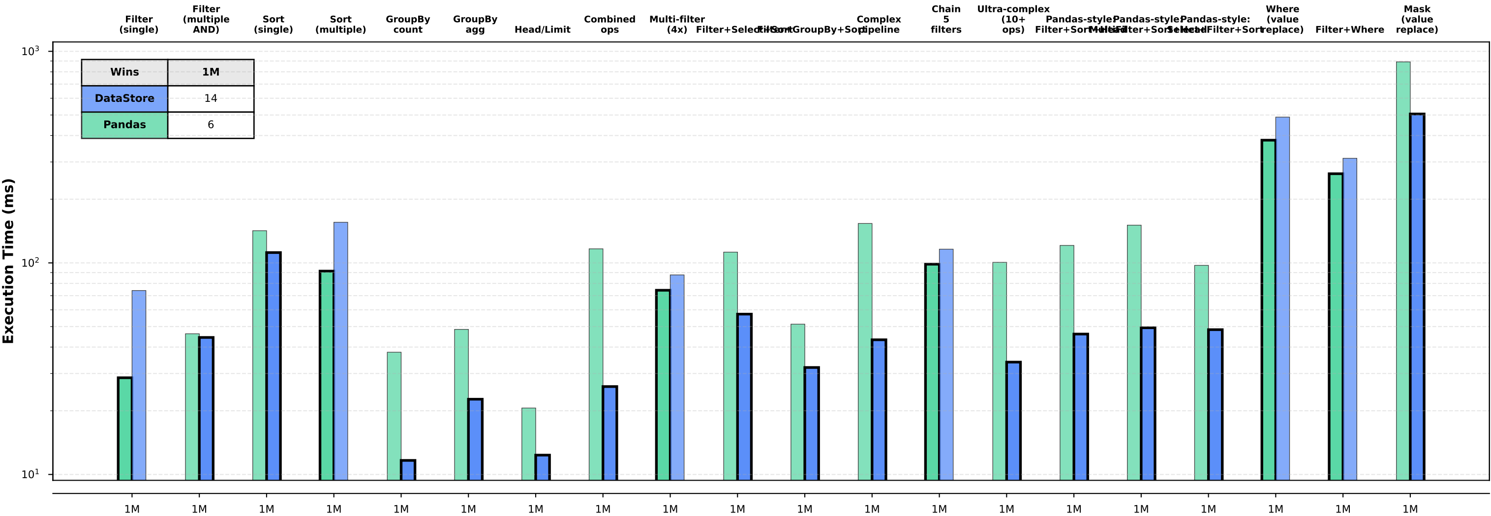
DataFrame Performance Benchmark: Pandas vs DataStore (chDB lazy mode)
