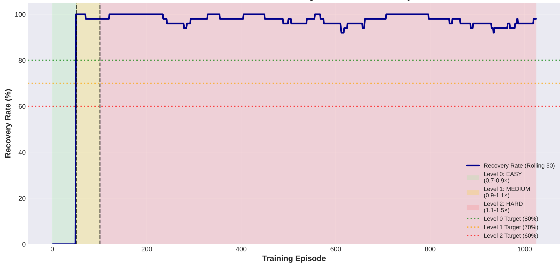
Performance-Gated Curriculum Progression with Recovery Rate
