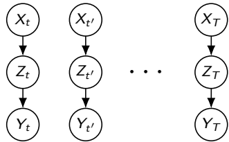
Stationary environment
