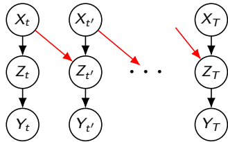
Non-stationary environment
