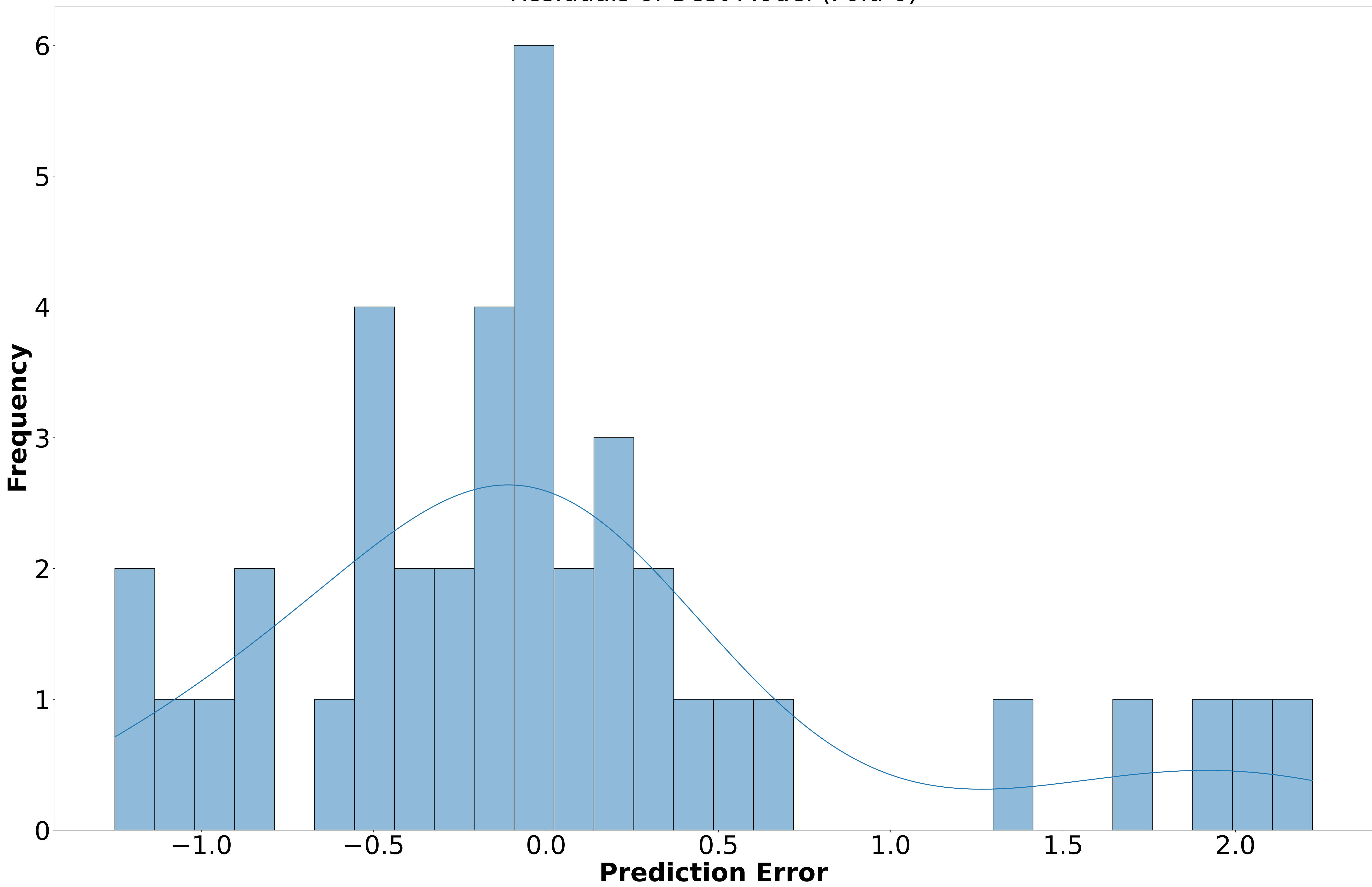
Residuals of Best Model (Fold 6)
