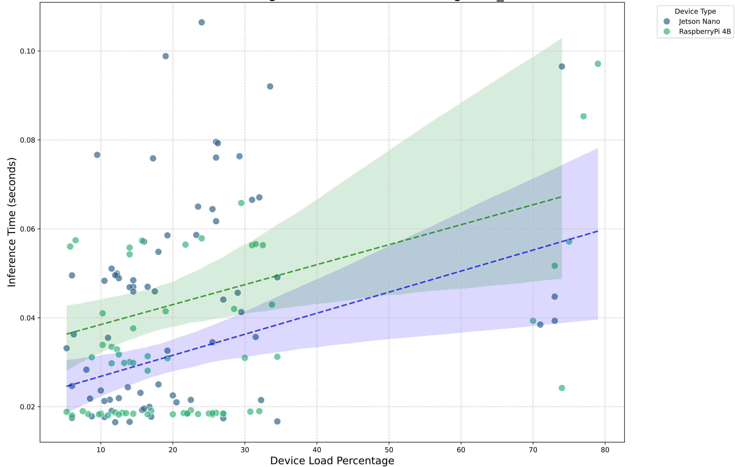
Device Load Percentage vs. Inference Time (Googlenet_Part3)
