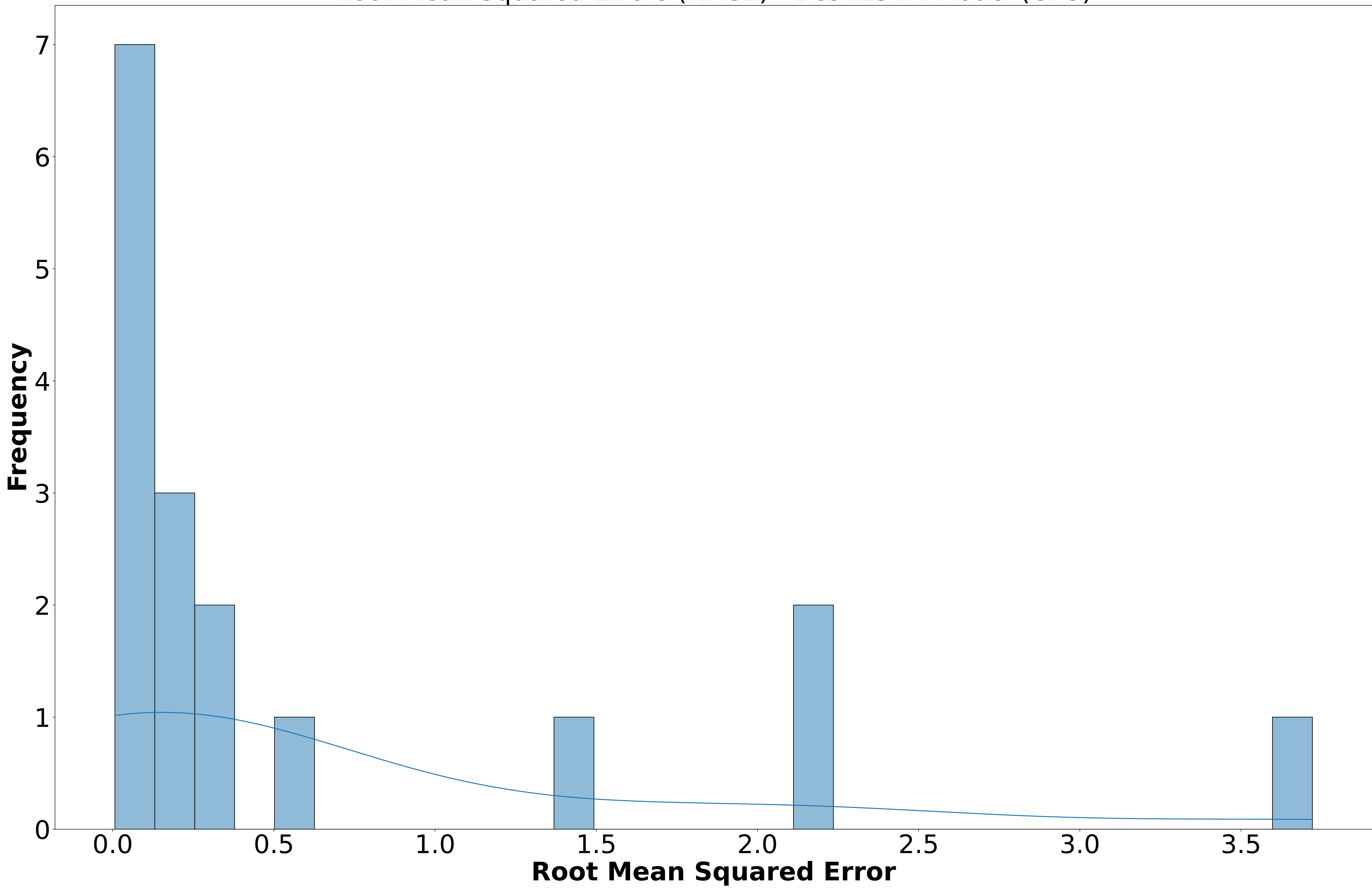
Root Mean Squared Errors (RMSE) - Best LSTM Model (CPU)
