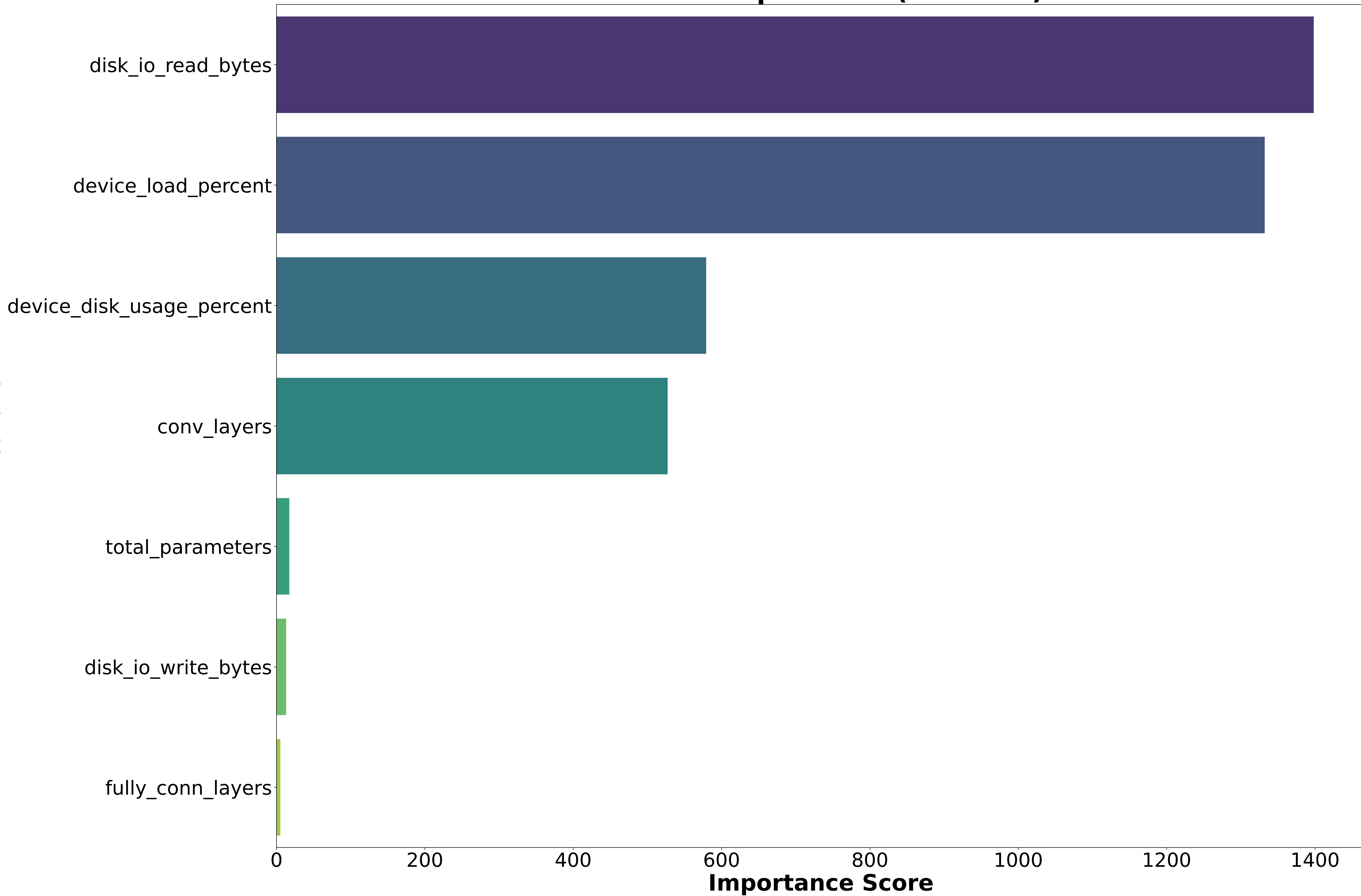
Feature Importance (XGBoost)
