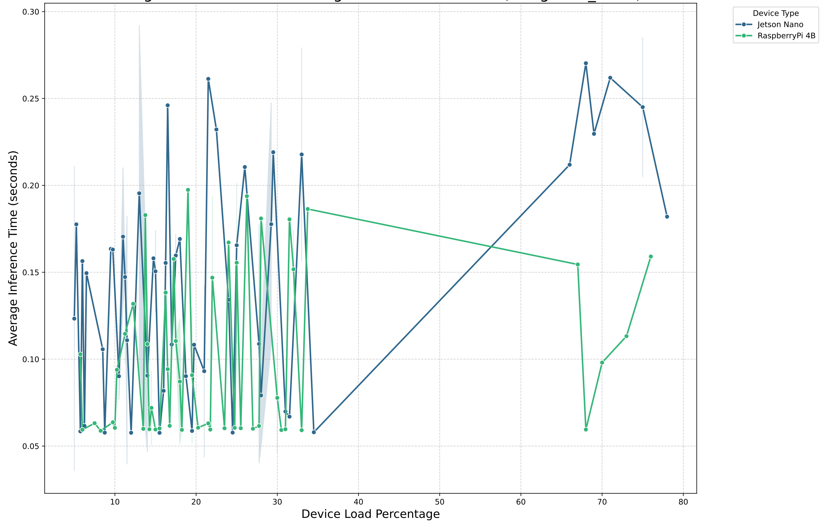
Average Device Load Percentage vs. Inference Time (Googlenet_Part2)
