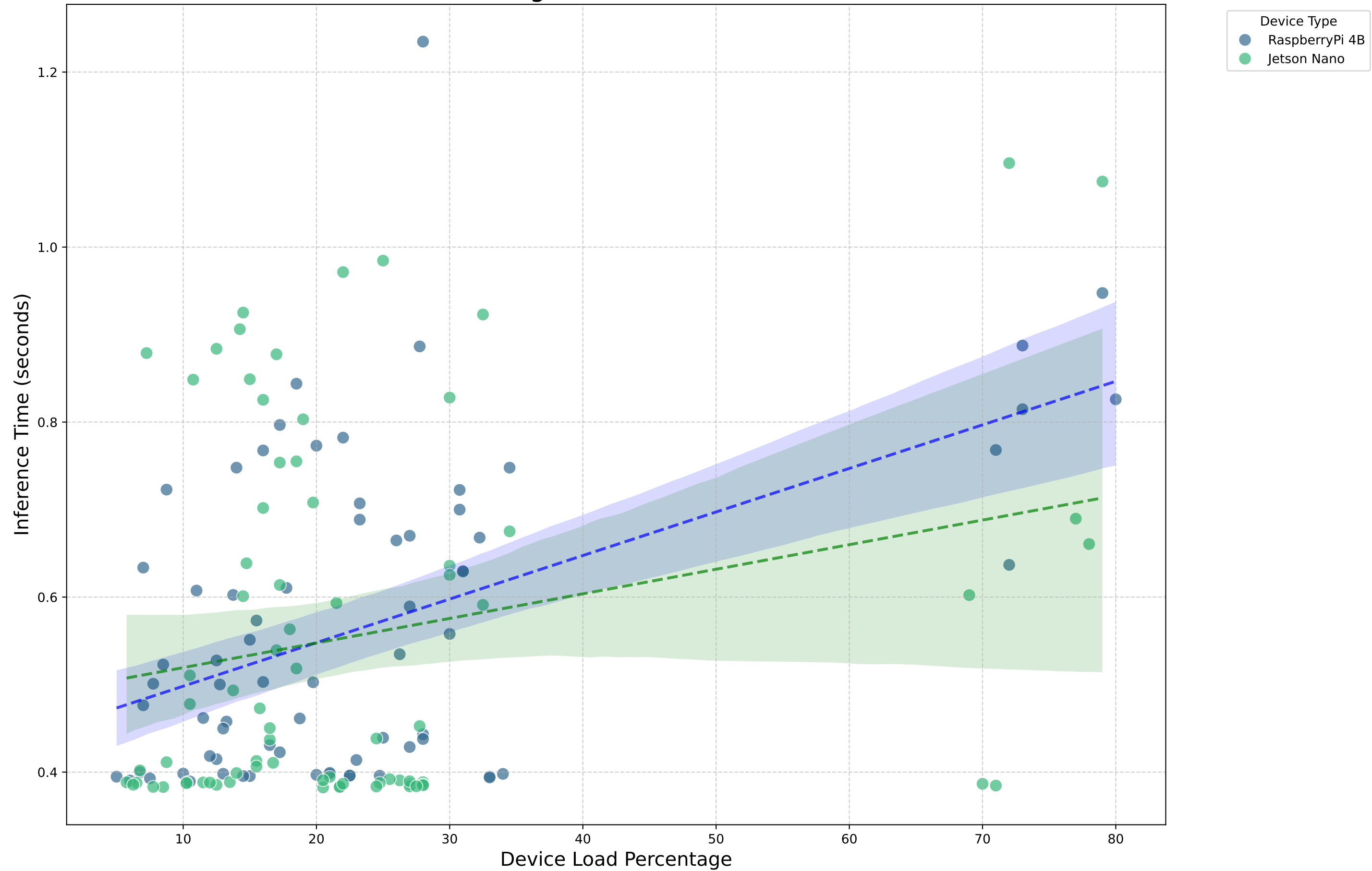
Device Load Percentage vs. Inference Time (Efficientnet)
