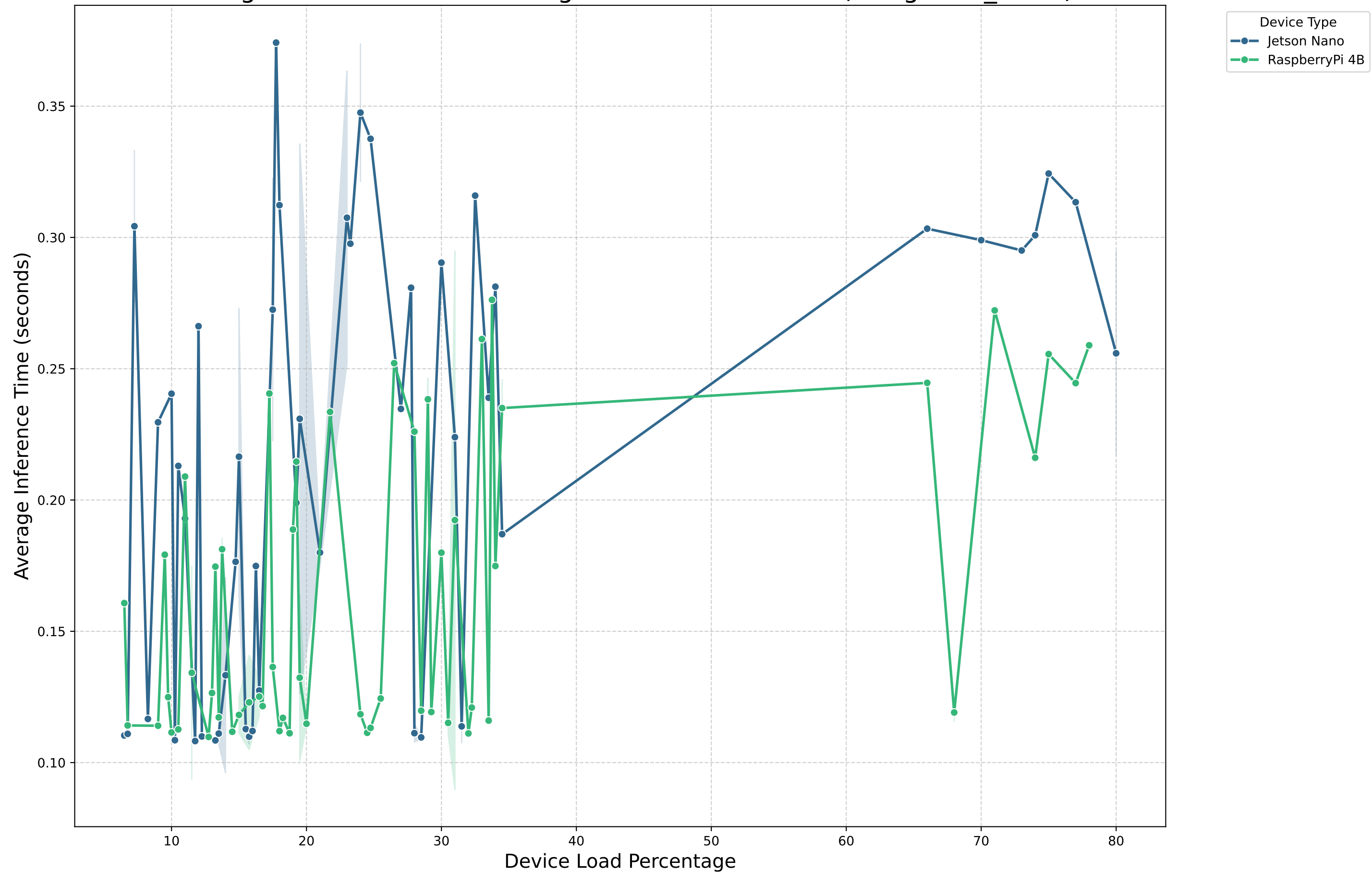
Average Device Load Percentage vs. Inference Time (Googlenet_Part1)
