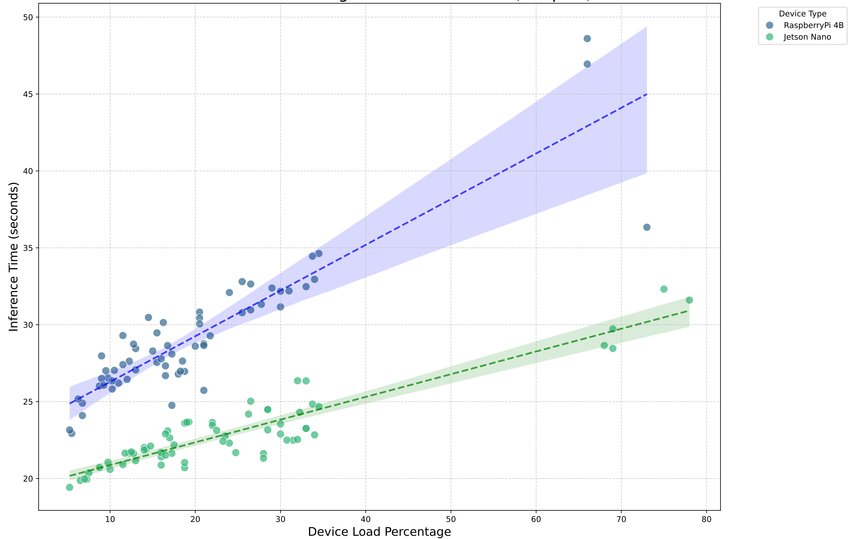
Device Load Percentage vs. Inference Time (Deeplab)
