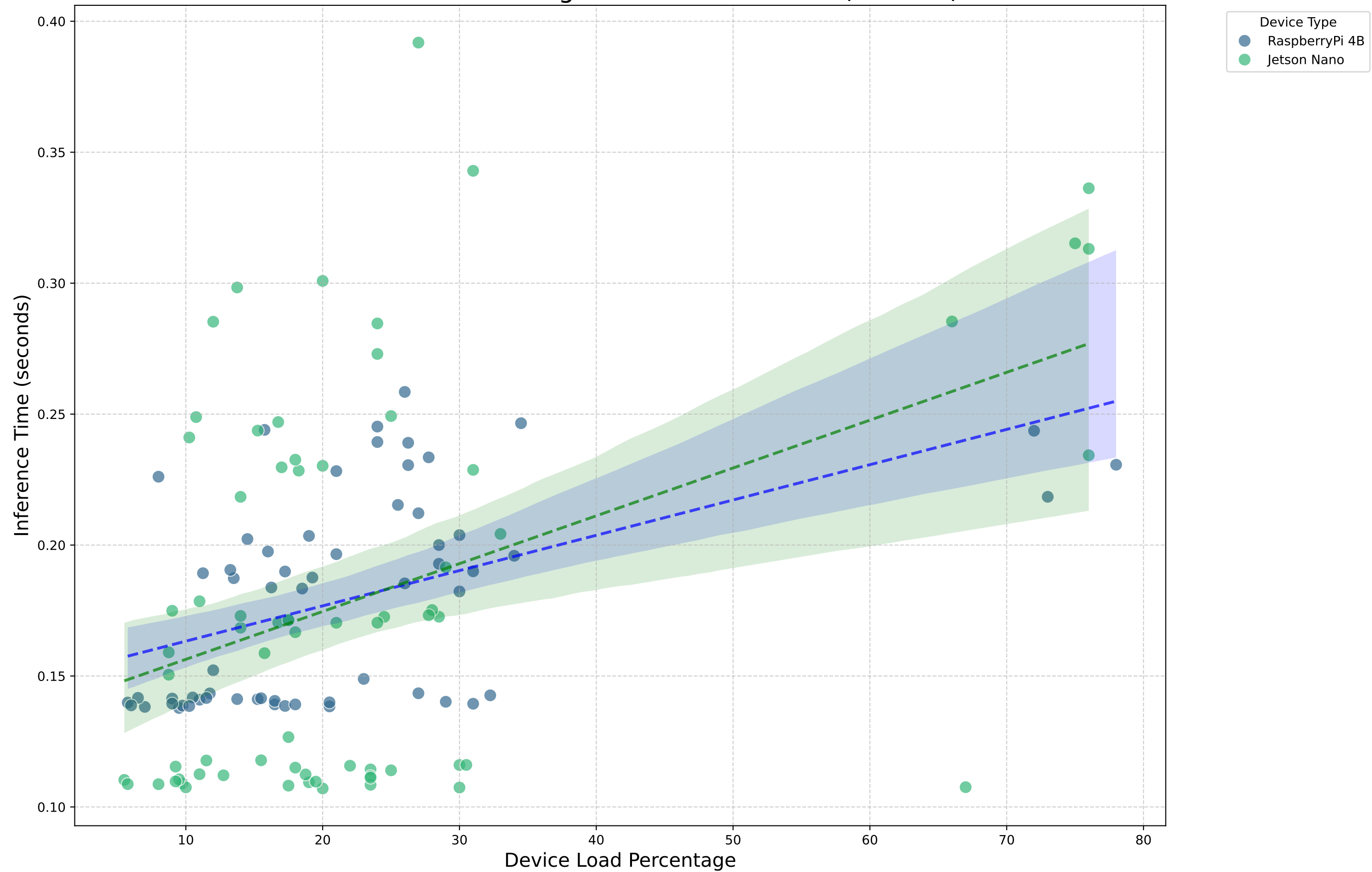
Device Load Percentage vs. Inference Time (Alexnet)
