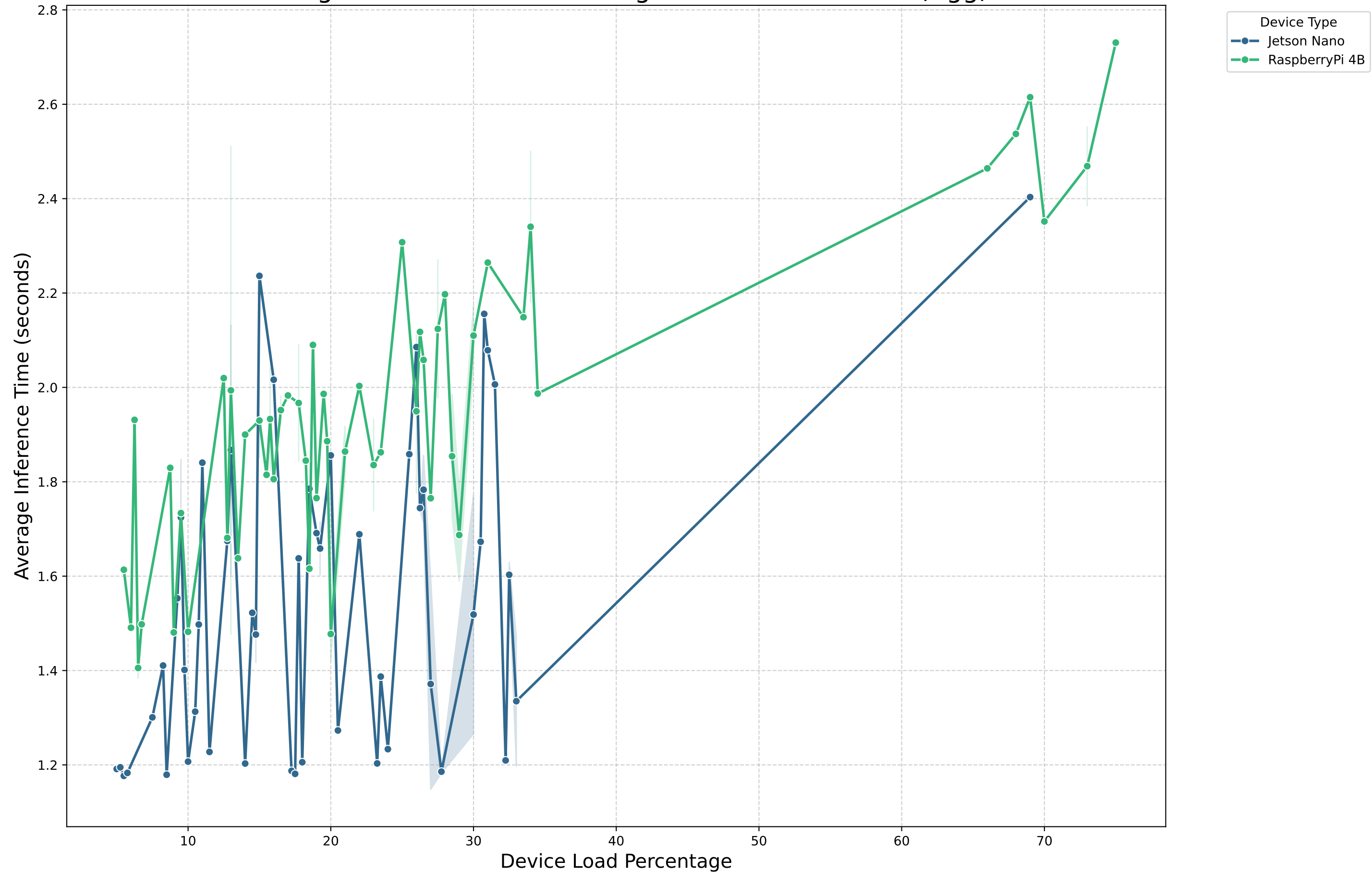
Average Device Load Percentage vs. Inference Time (Vgg)
