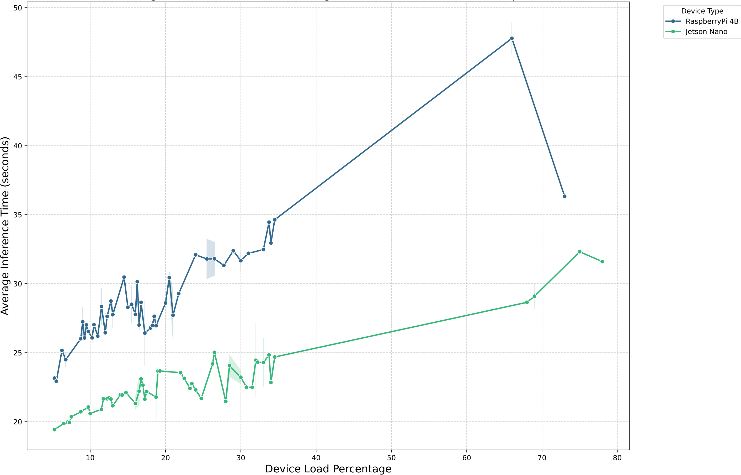
Average Device Load Percentage vs. Inference Time (Deeplab)
