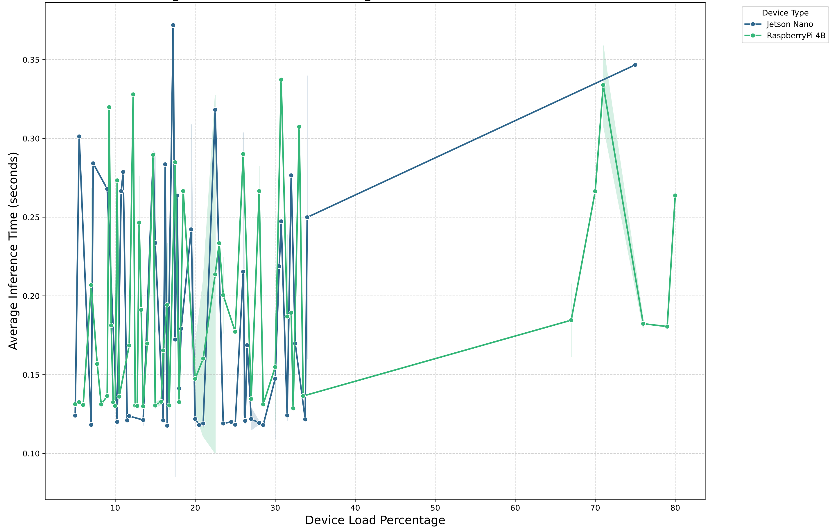
Average Device Load Percentage vs. Inference Time (Mobilenet)
