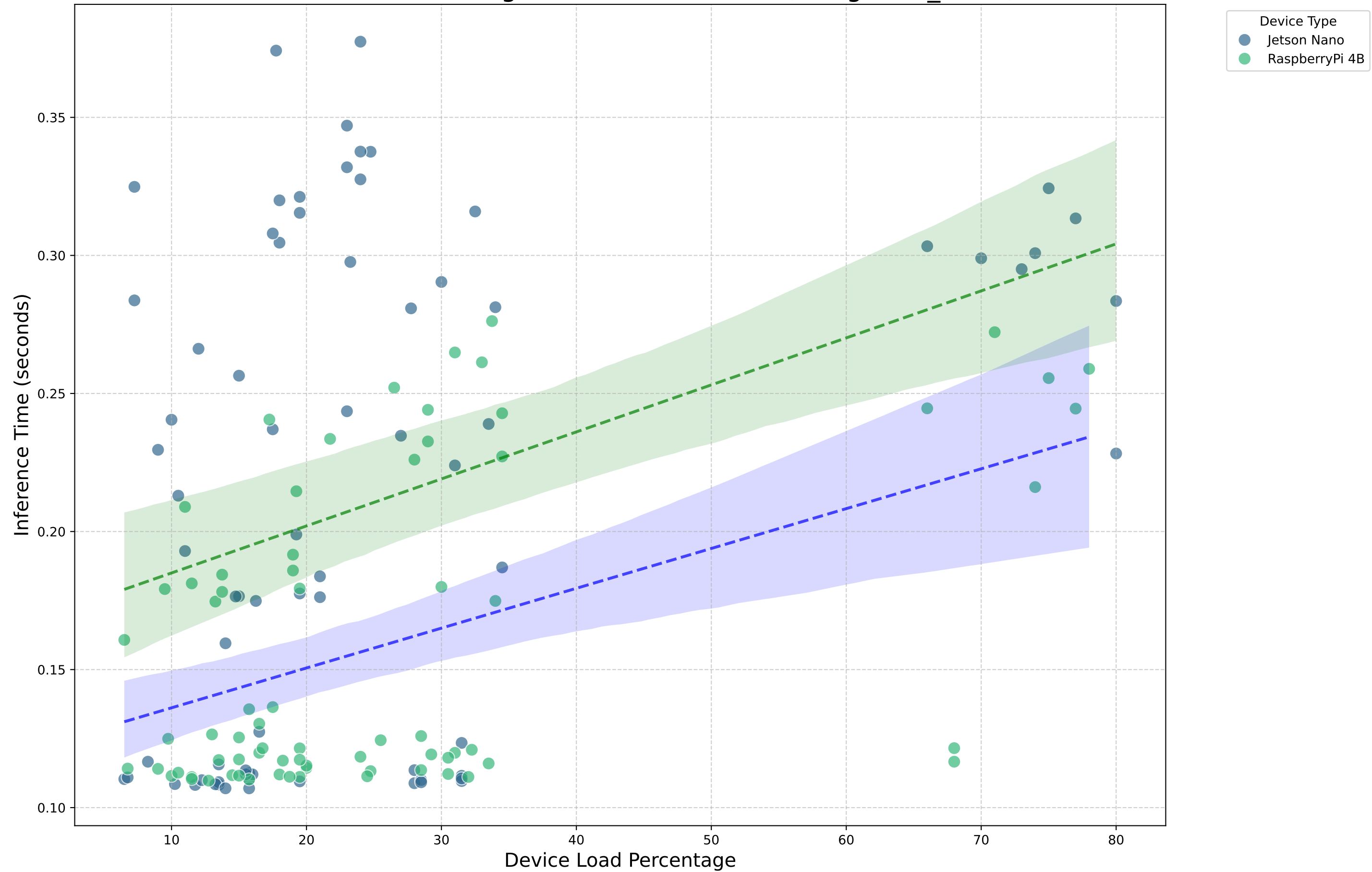
Device Load Percentage vs. Inference Time (Googlenet_Part1)
