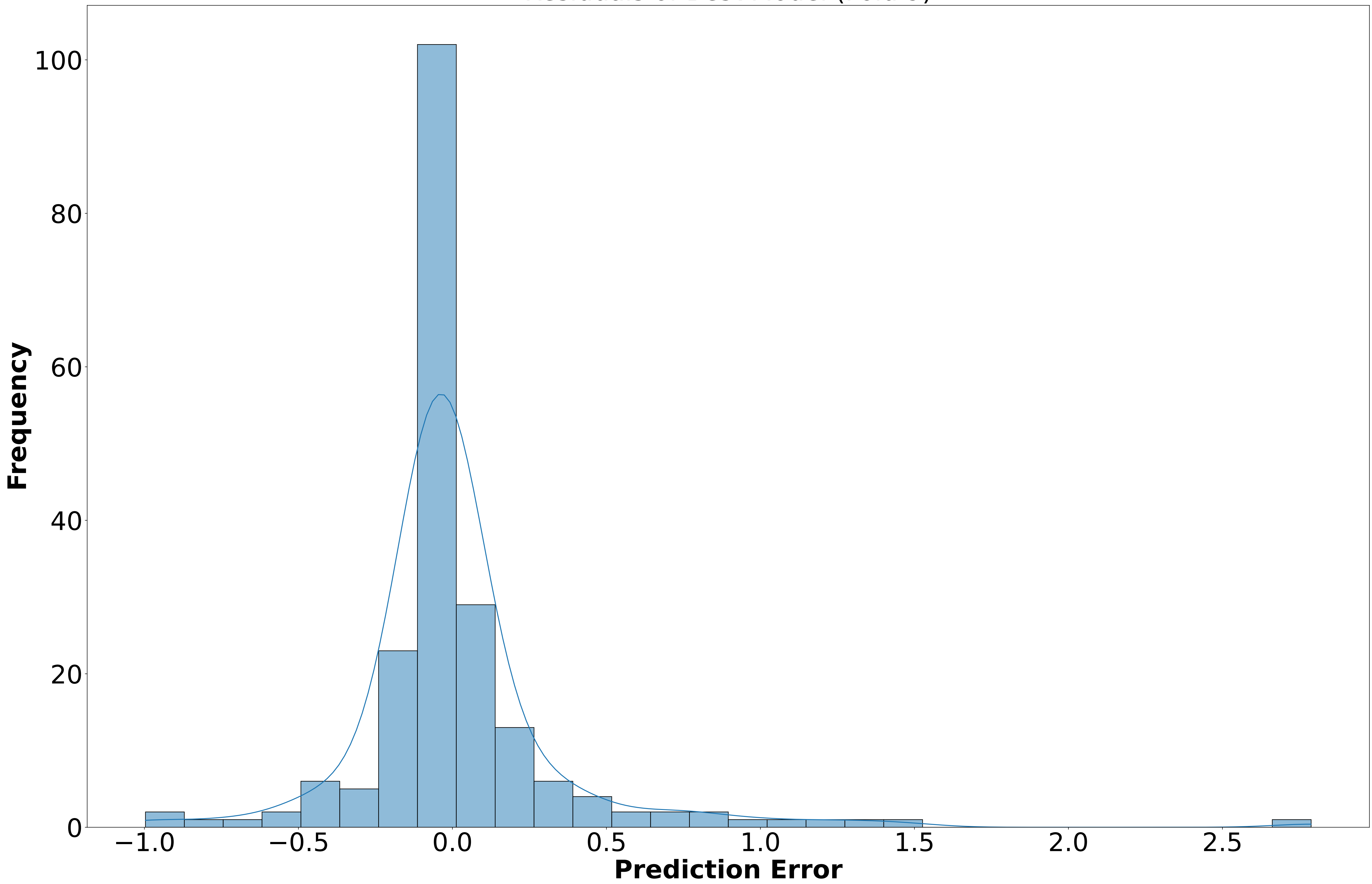
Residuals of Best Model (Fold 9)
