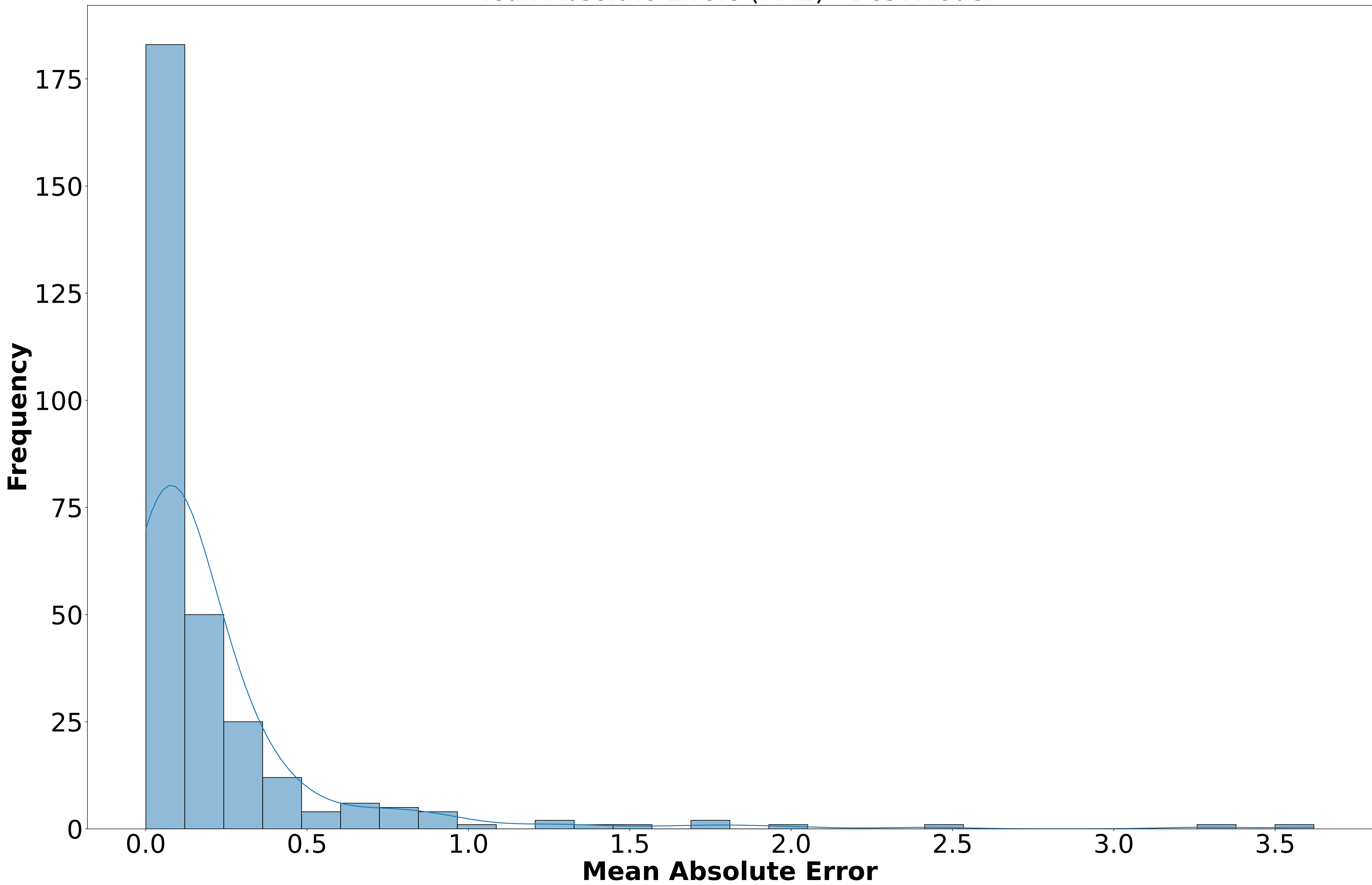
Mean Absolute Errors (MAE) - Best Model
