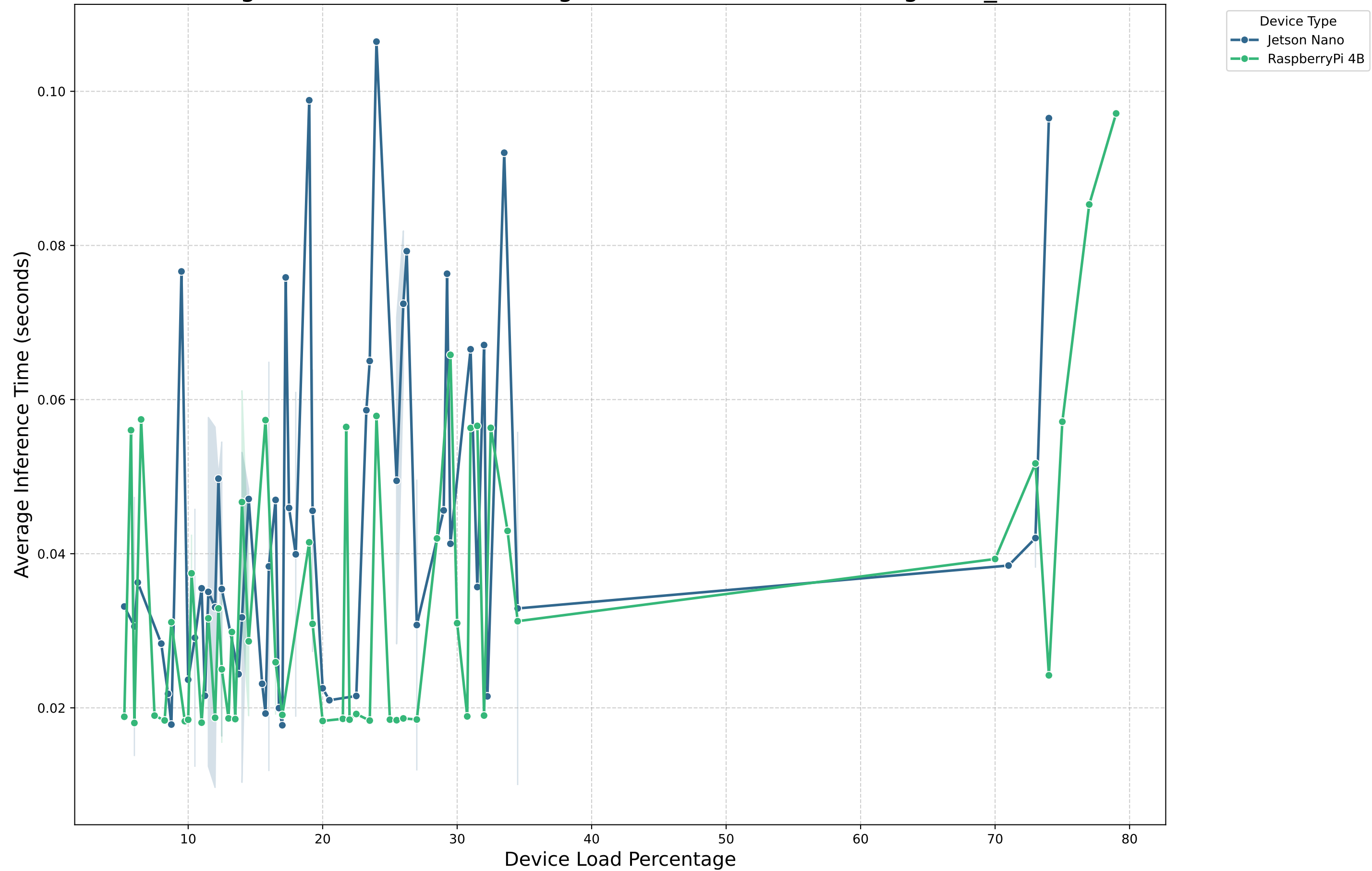
Average Device Load Percentage vs. Inference Time (Googlenet_Part3)
