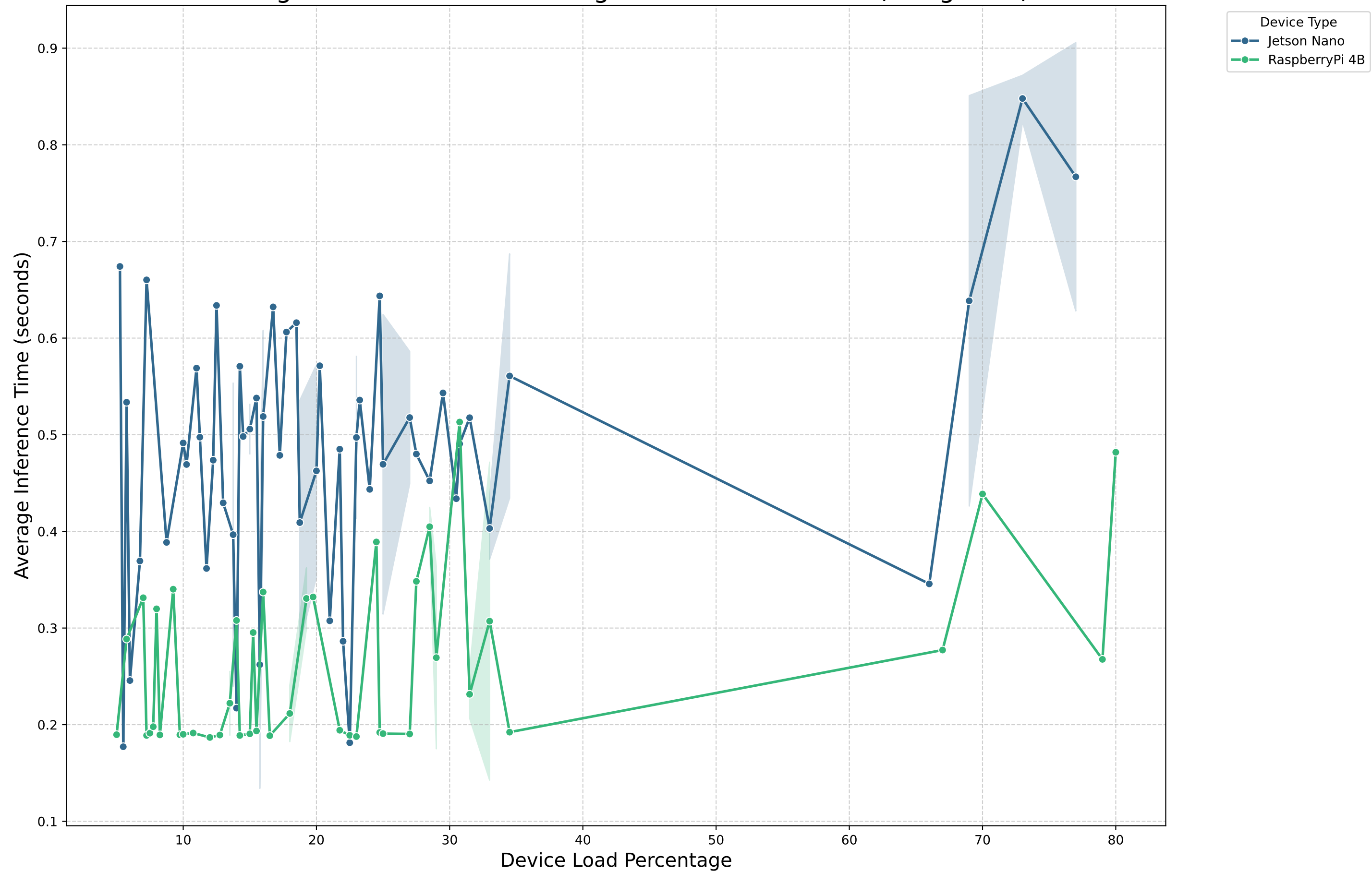
Average Device Load Percentage vs. Inference Time (Googlenet)
