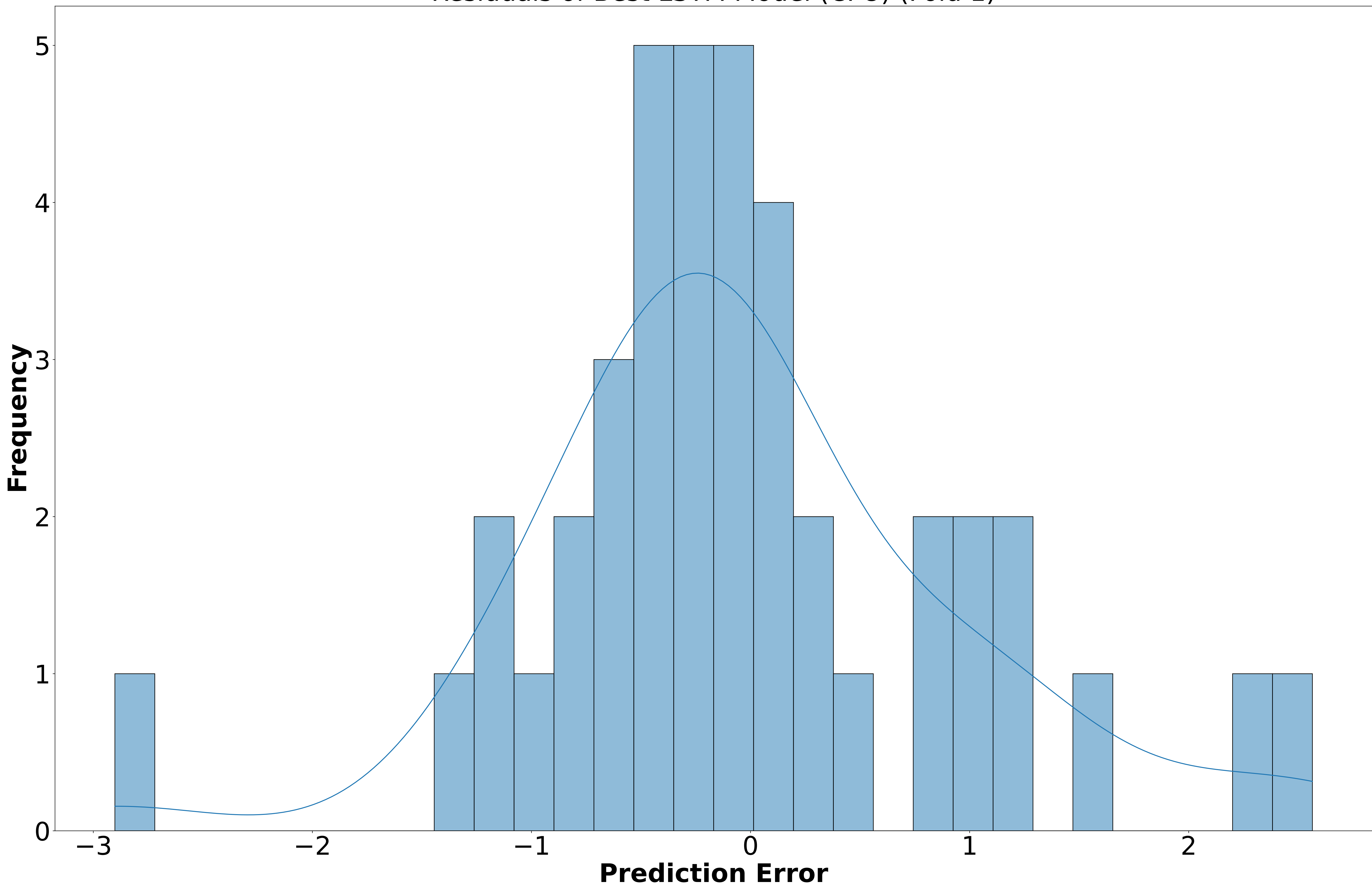
Residuals of Best LSTM Model (CPU) (Fold 1)
