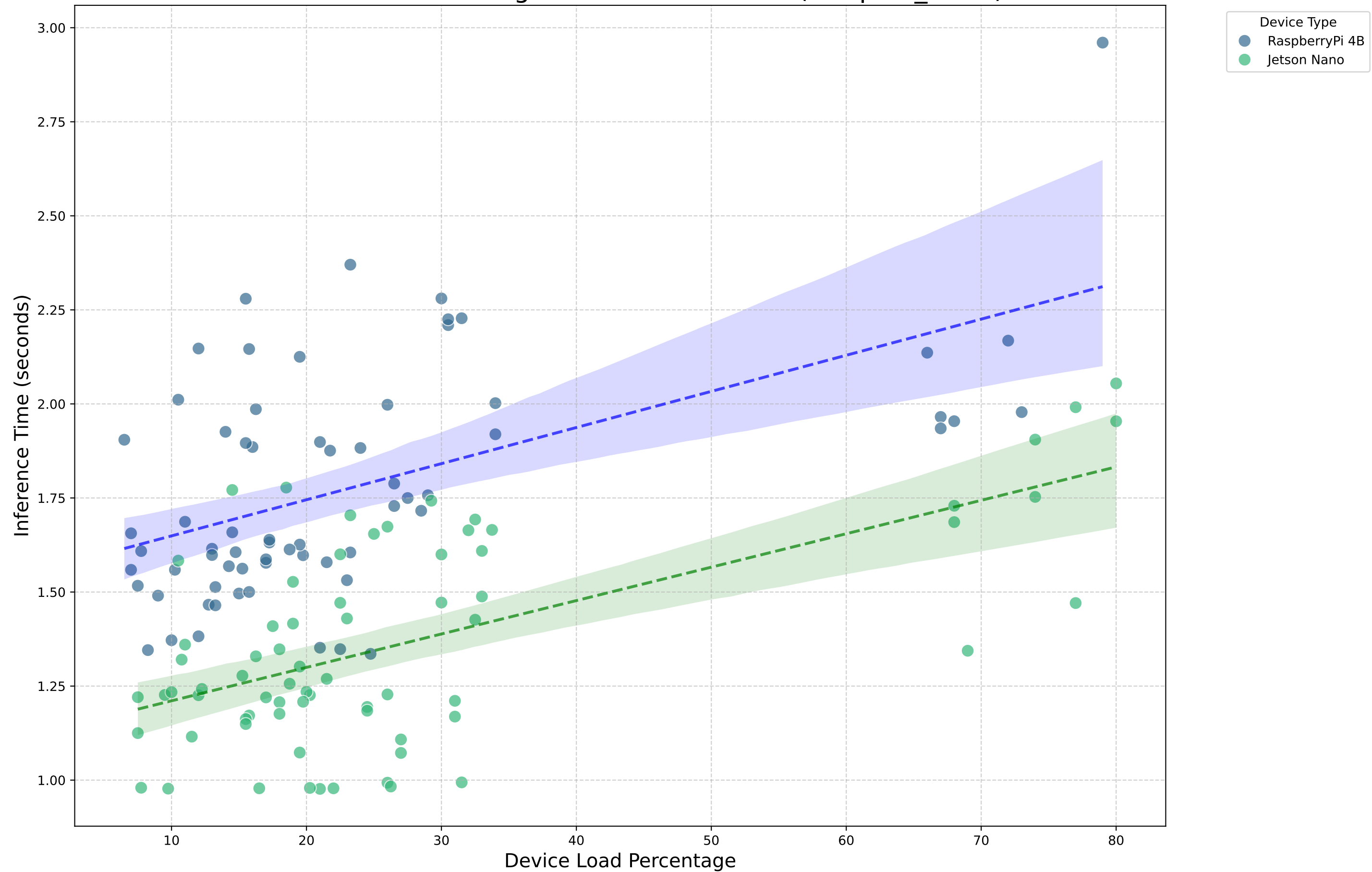
Device Load Percentage vs. Inference Time (Deeplab_Part2)
