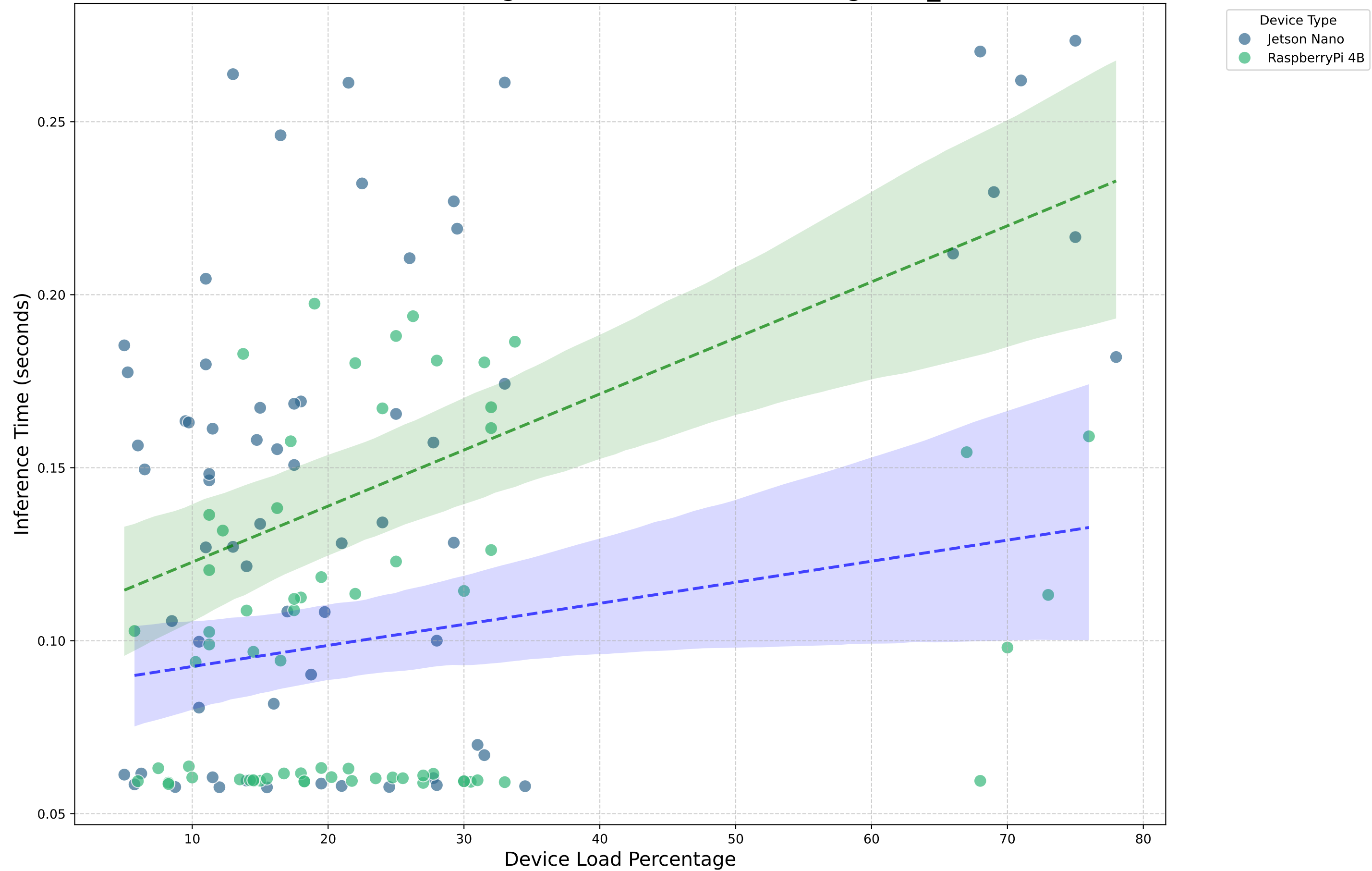
Device Load Percentage vs. Inference Time (Googlenet_Part2)
