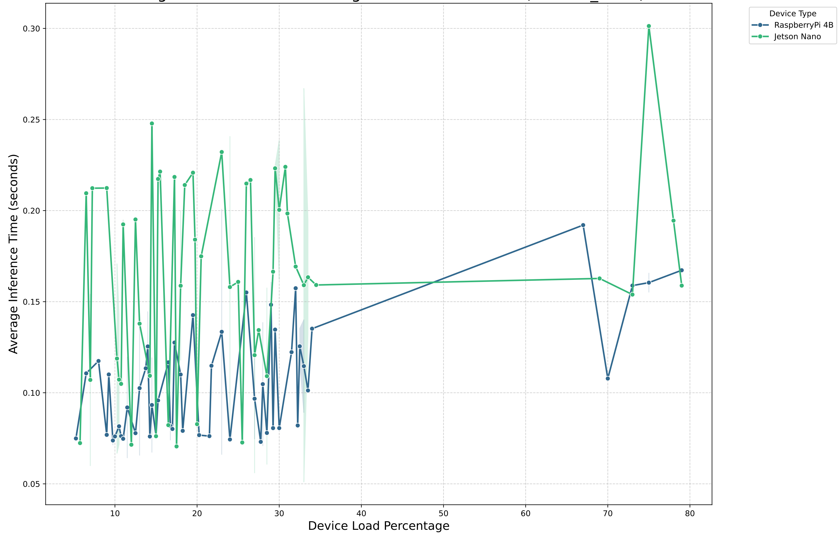
Average Device Load Percentage vs. Inference Time (Alexnet_Part1)
