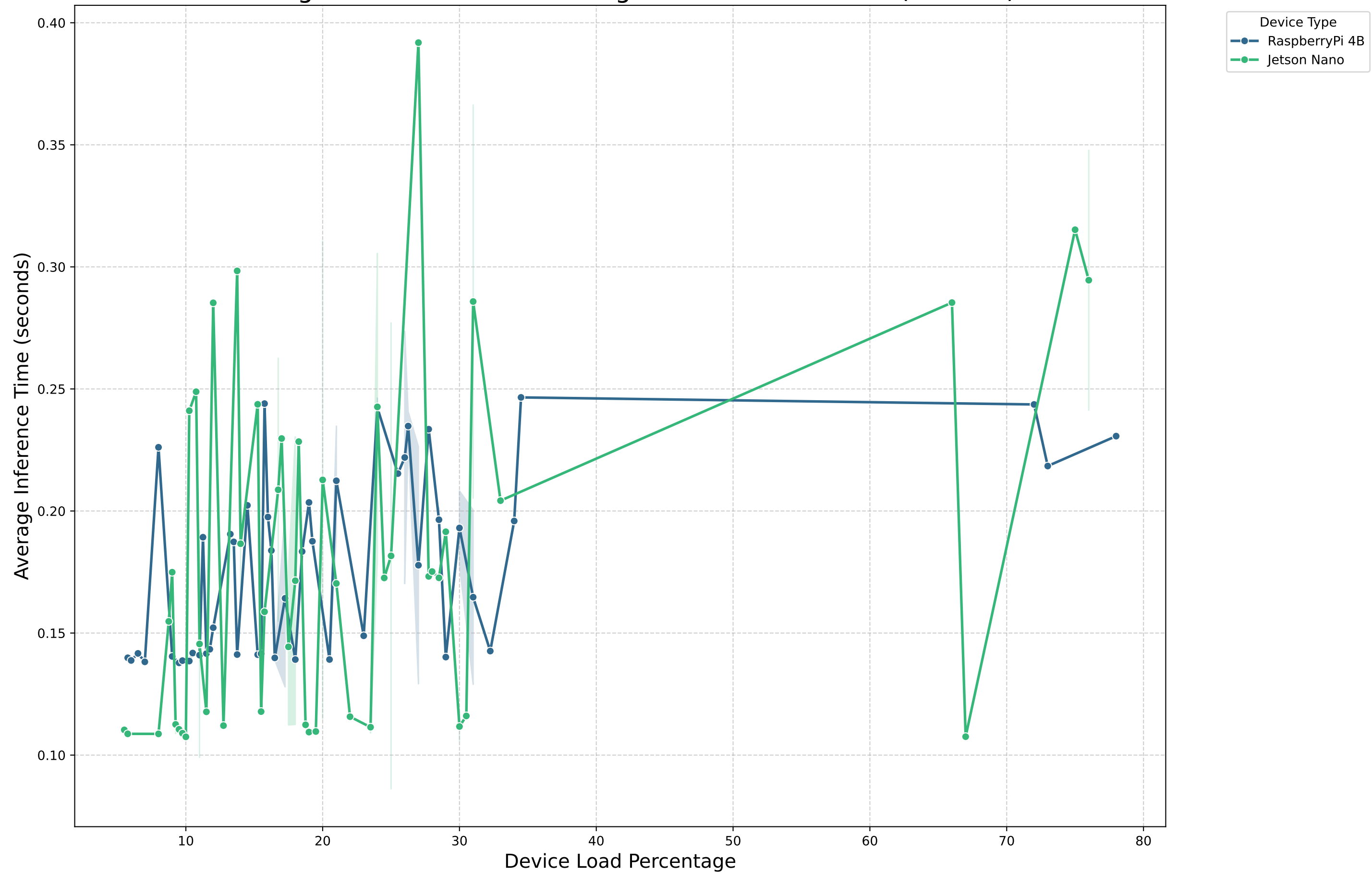
Average Device Load Percentage vs. Inference Time (Alexnet)
