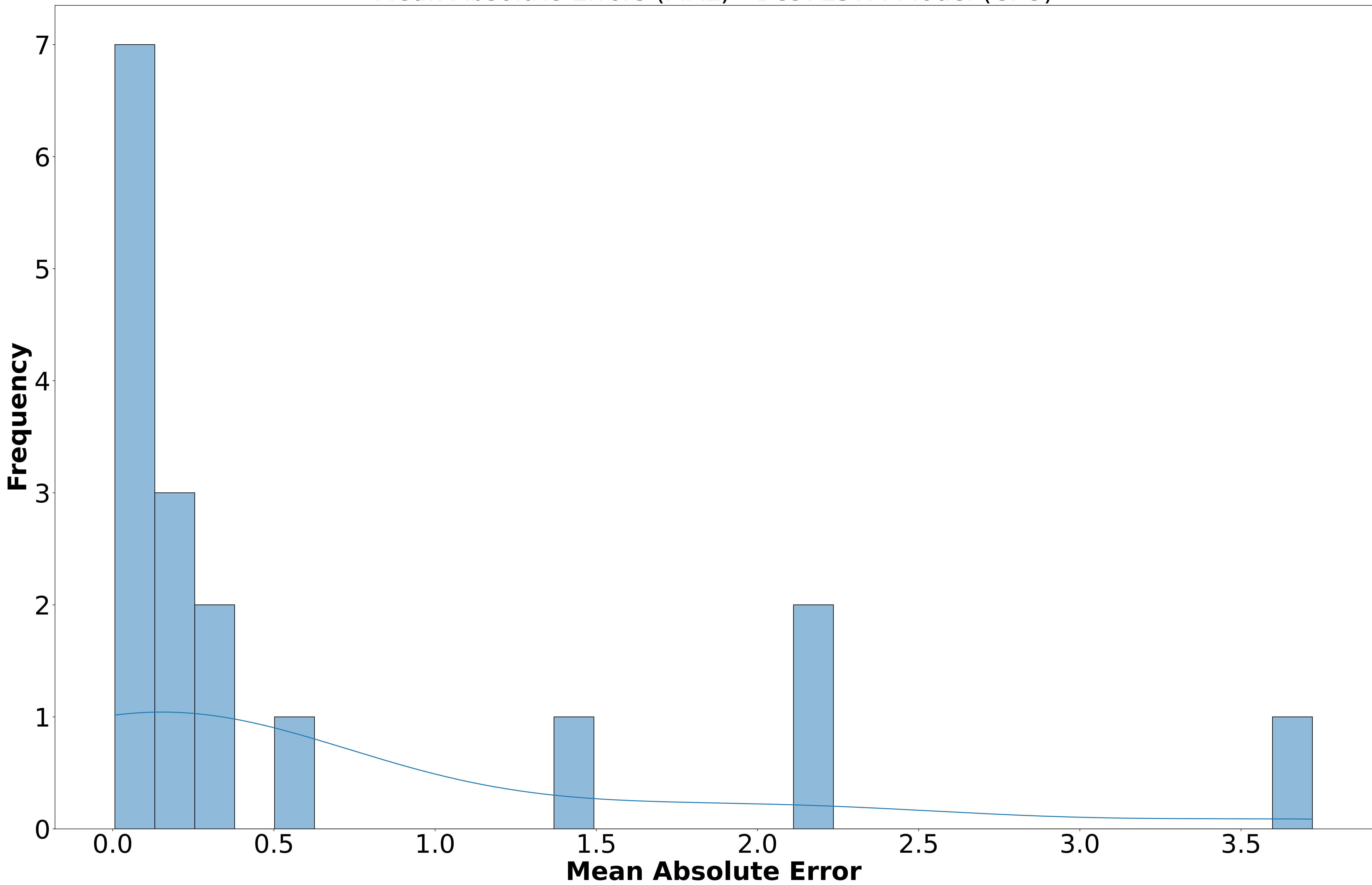
Mean Absolute Errors (MAE) - Best LSTM Model (CPU)
