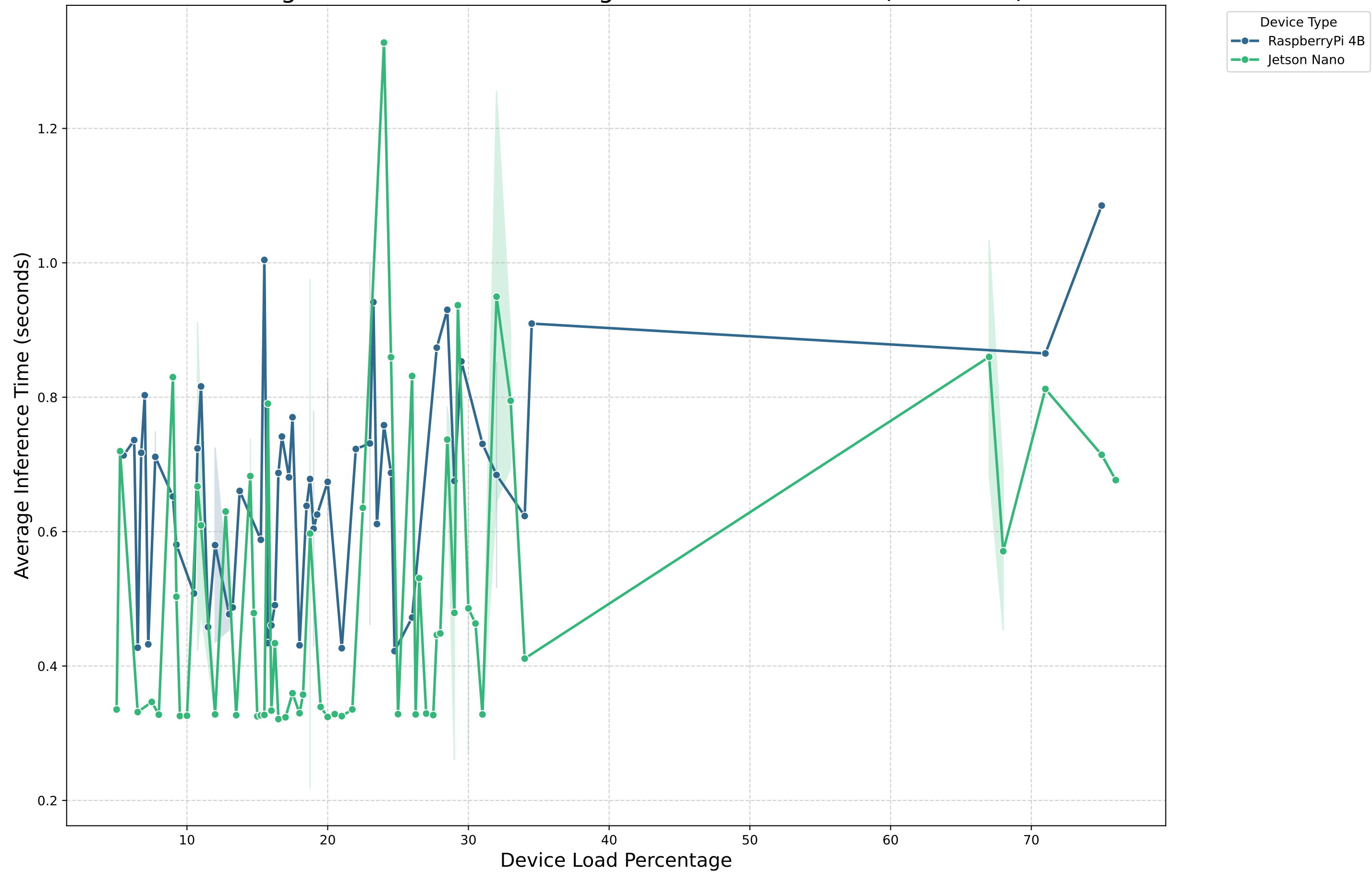
Average Device Load Percentage vs. Inference Time (Densenet)
