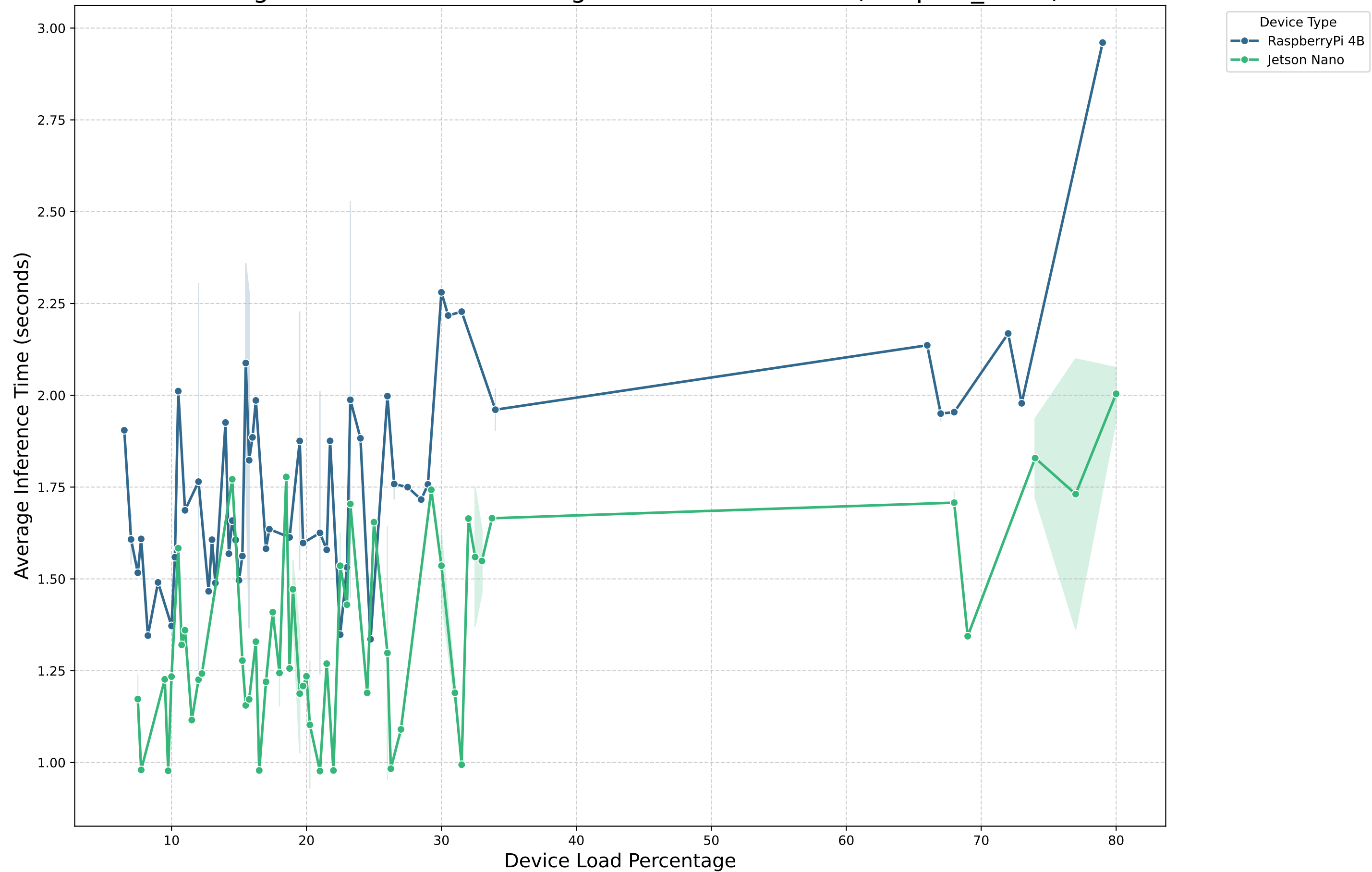
Average Device Load Percentage vs. Inference Time (Deeplab_Part2)
