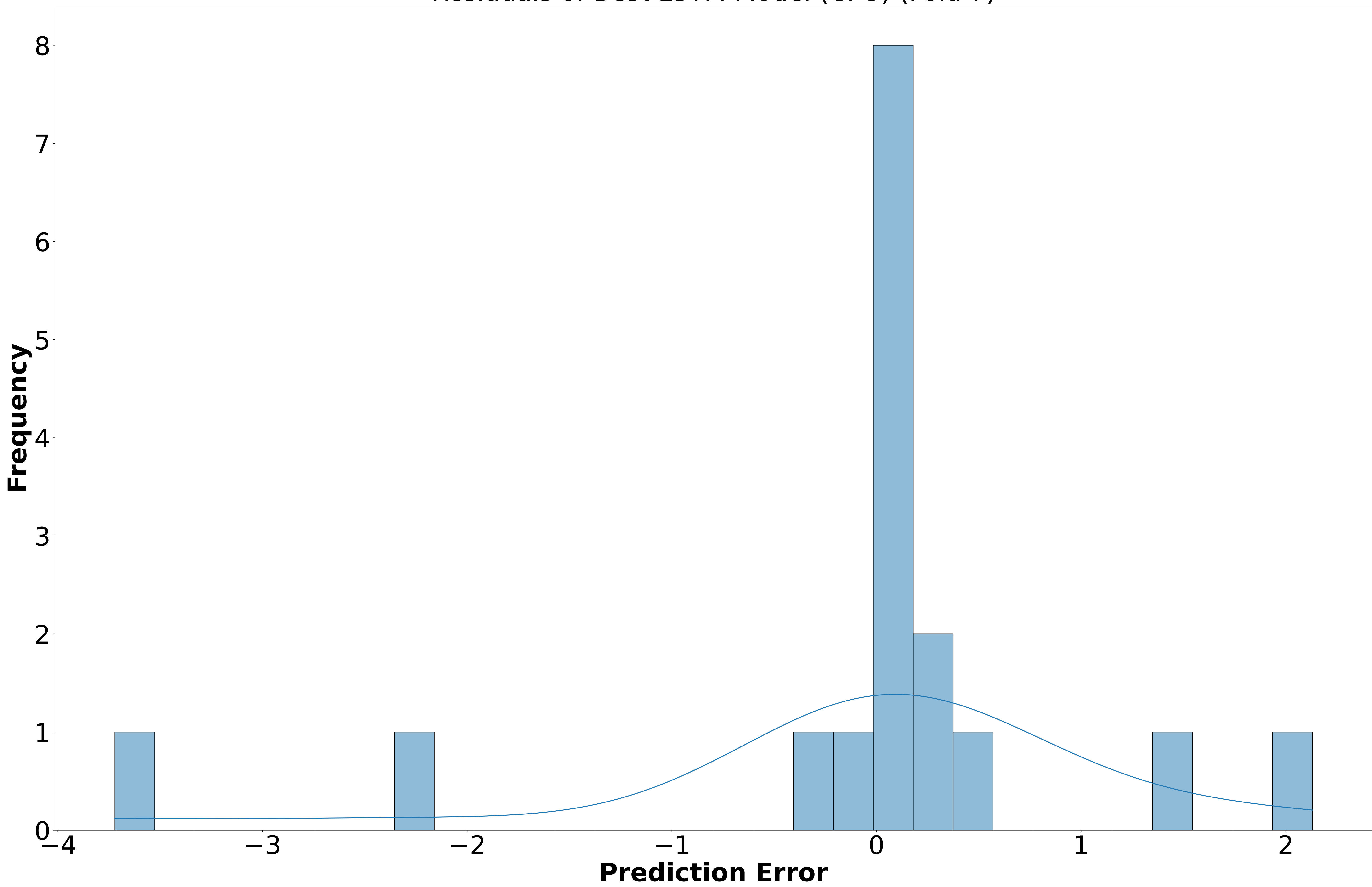
Residuals of Best LSTM Model (CPU) (Fold 7)
