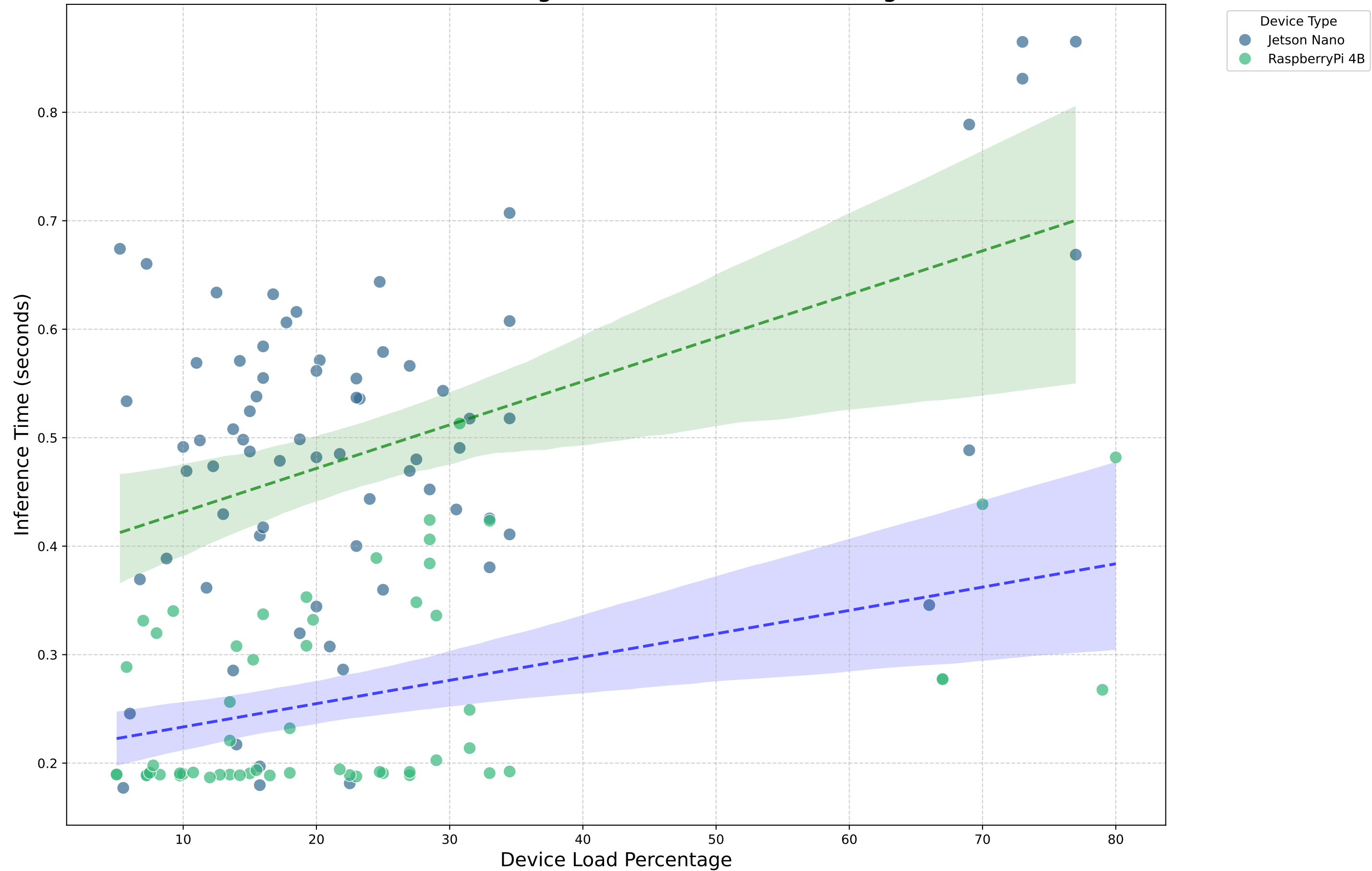
Device Load Percentage vs. Inference Time (Googlenet)
