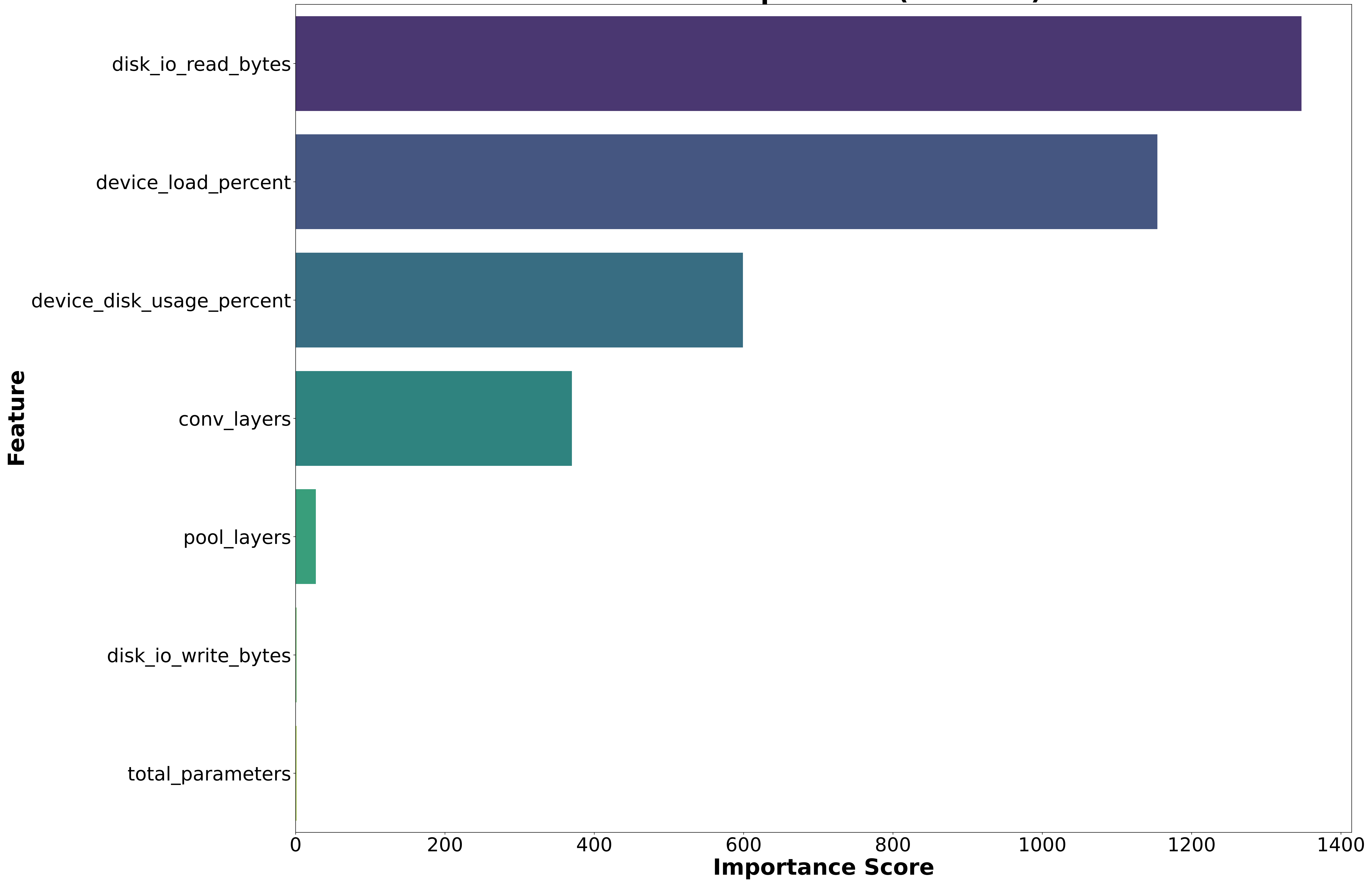
Feature Importance (XGBoost)
