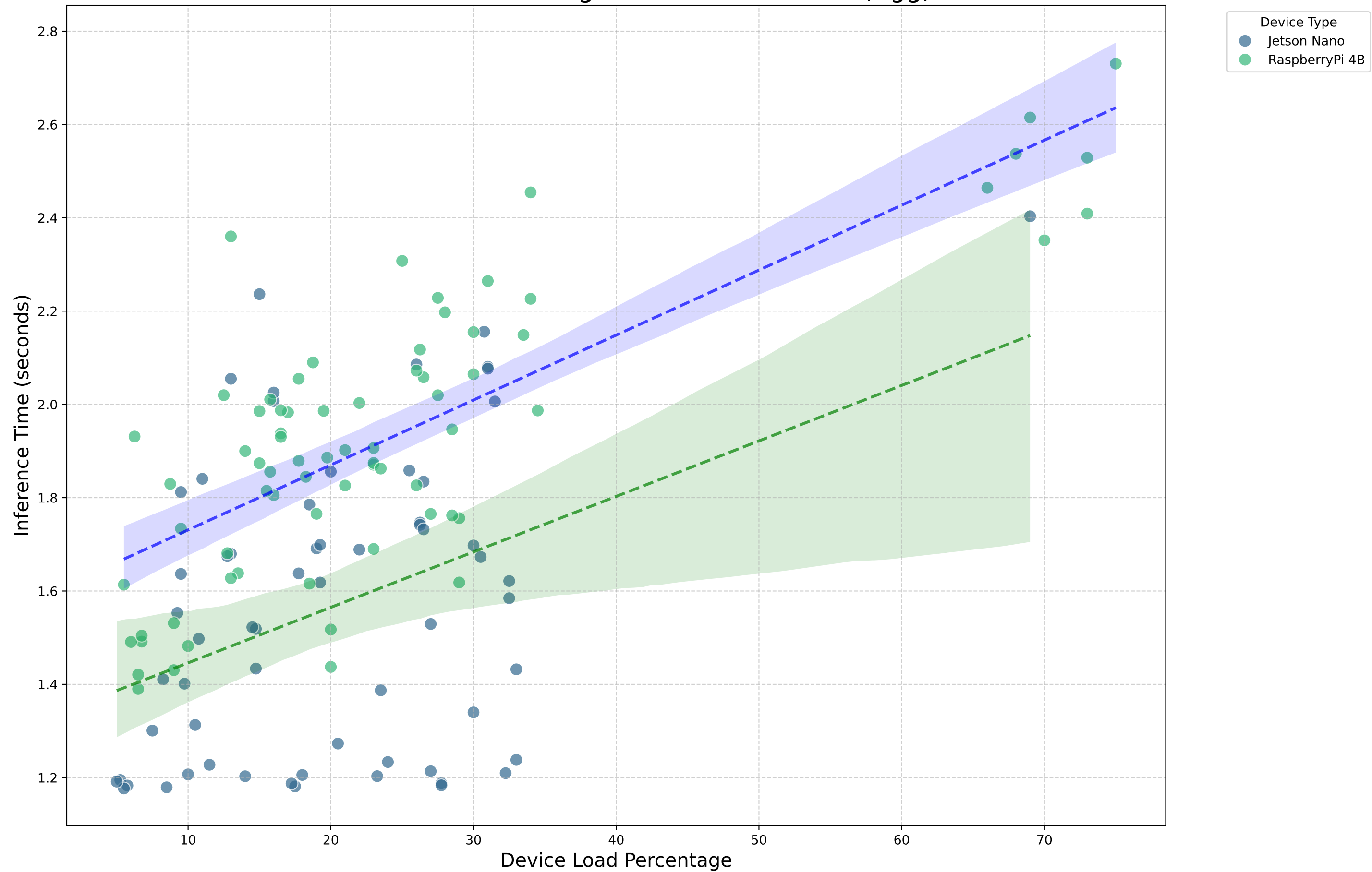
Device Load Percentage vs. Inference Time (Vgg)
