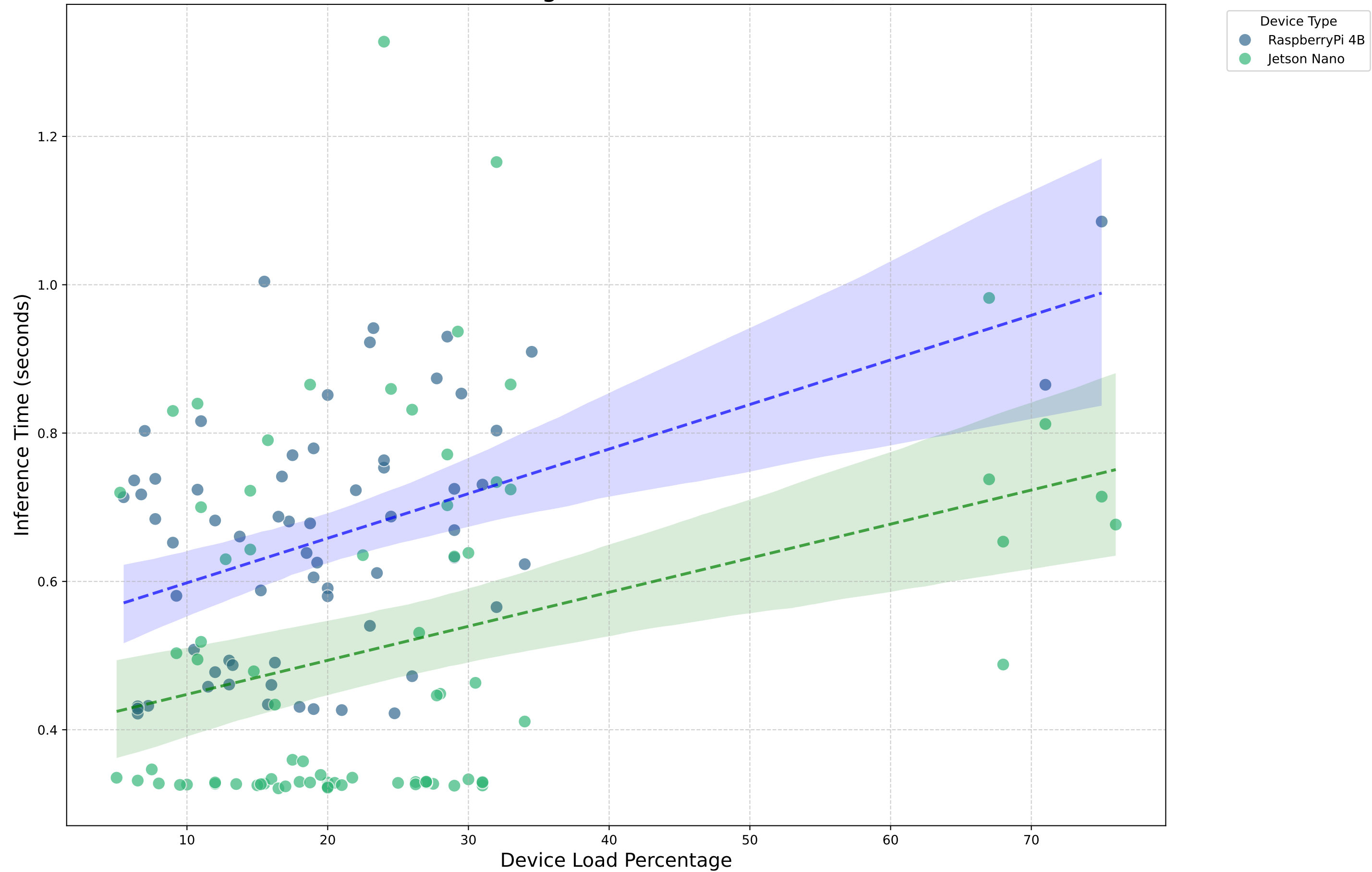
Device Load Percentage vs. Inference Time (Densenet)
