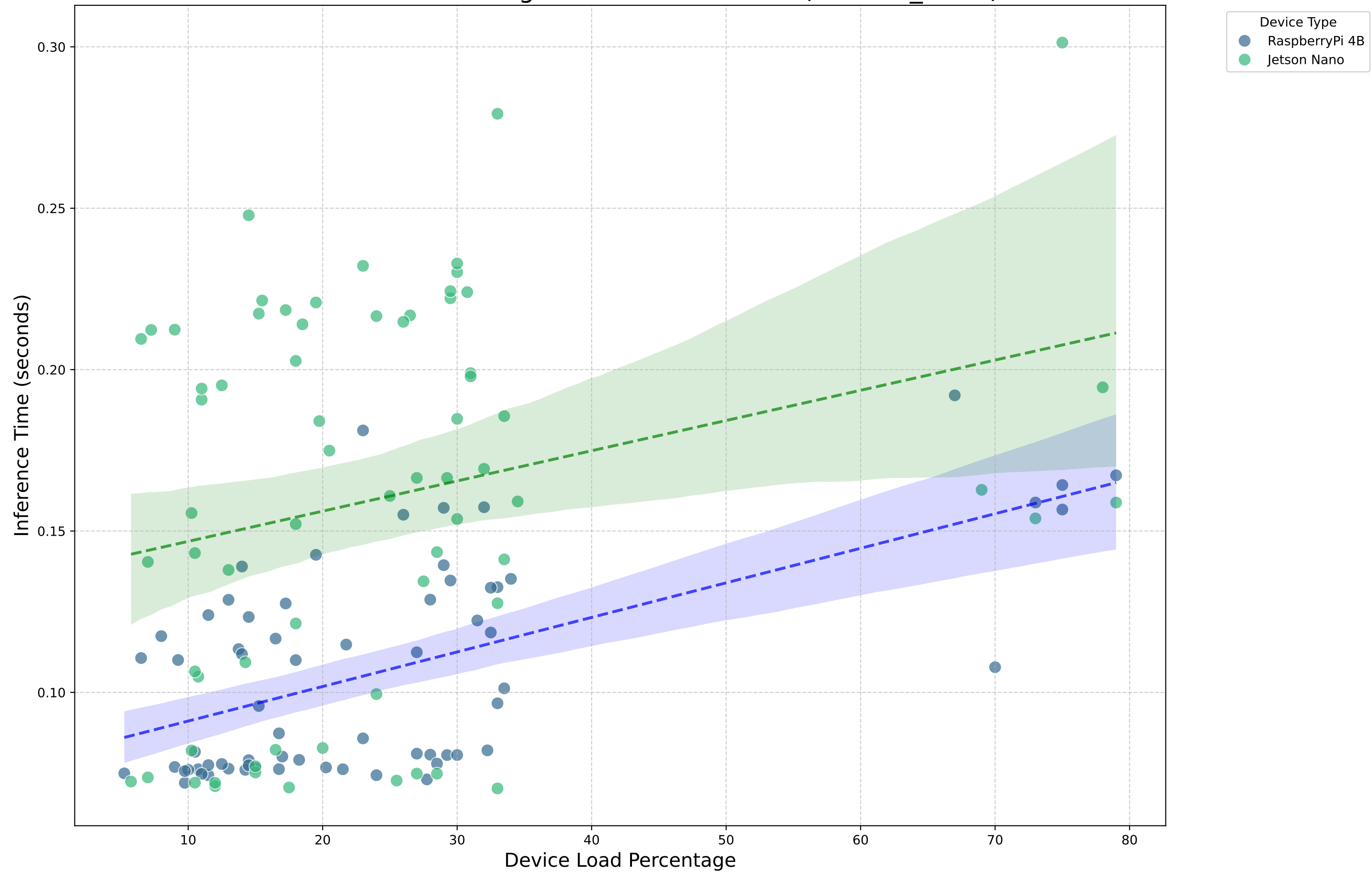
Device Load Percentage vs. Inference Time (Alexnet_Part1)
