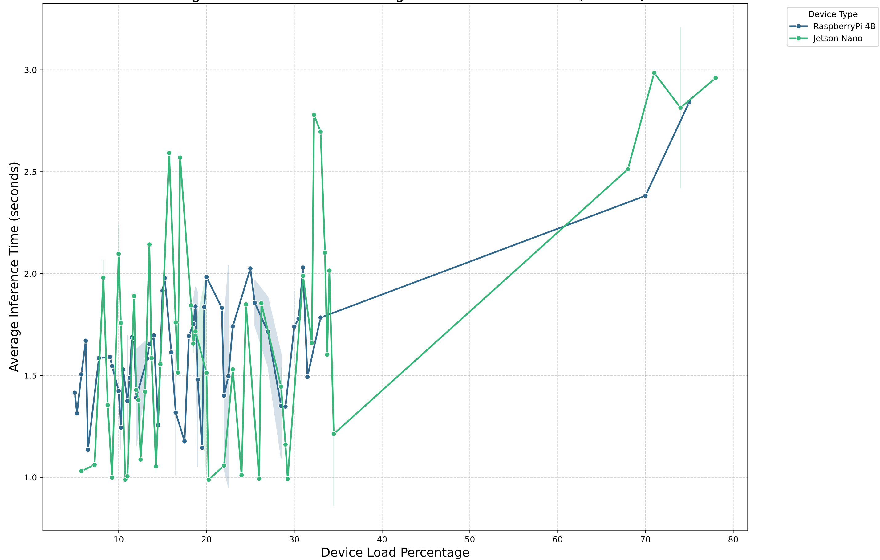
Average Device Load Percentage vs. Inference Time (Resnet)
