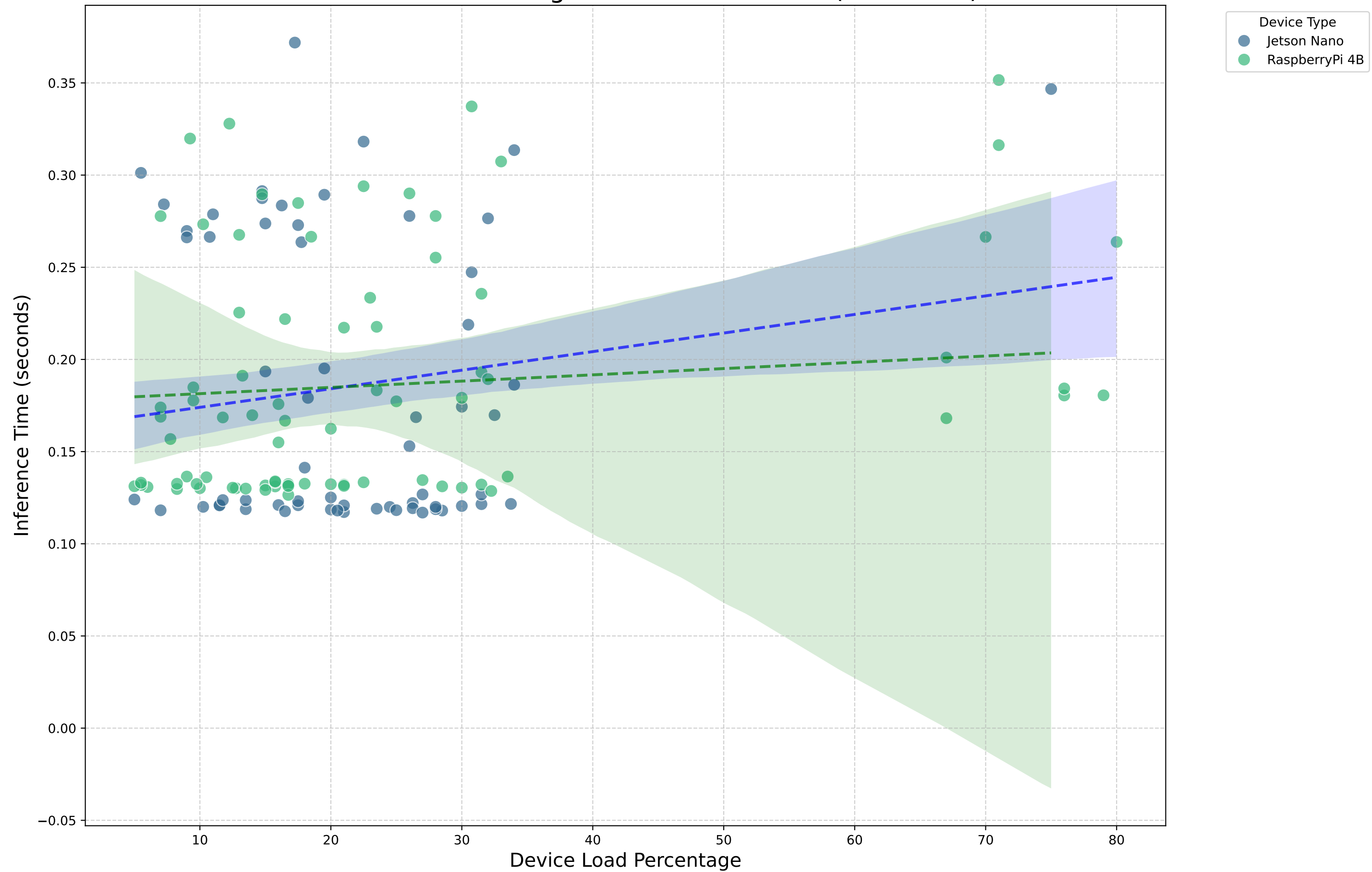
Device Load Percentage vs. Inference Time (Mobilenet)
