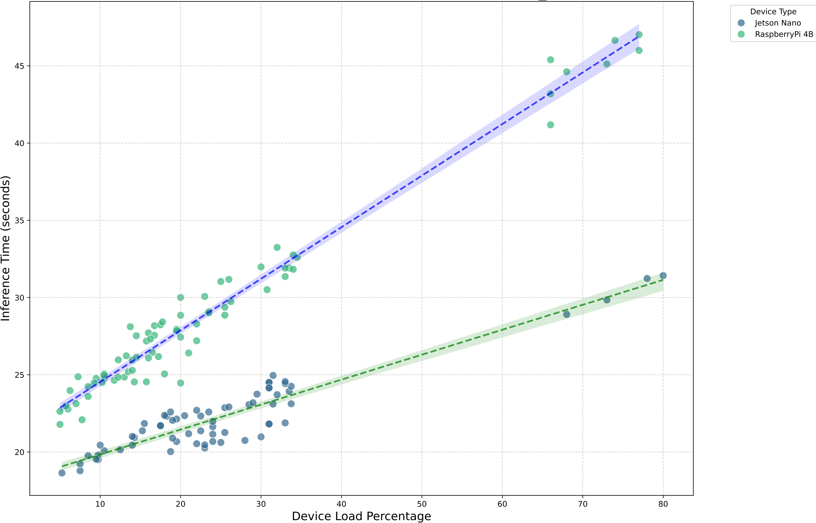
Device Load Percentage vs. Inference Time (Deeplab_Part1)
