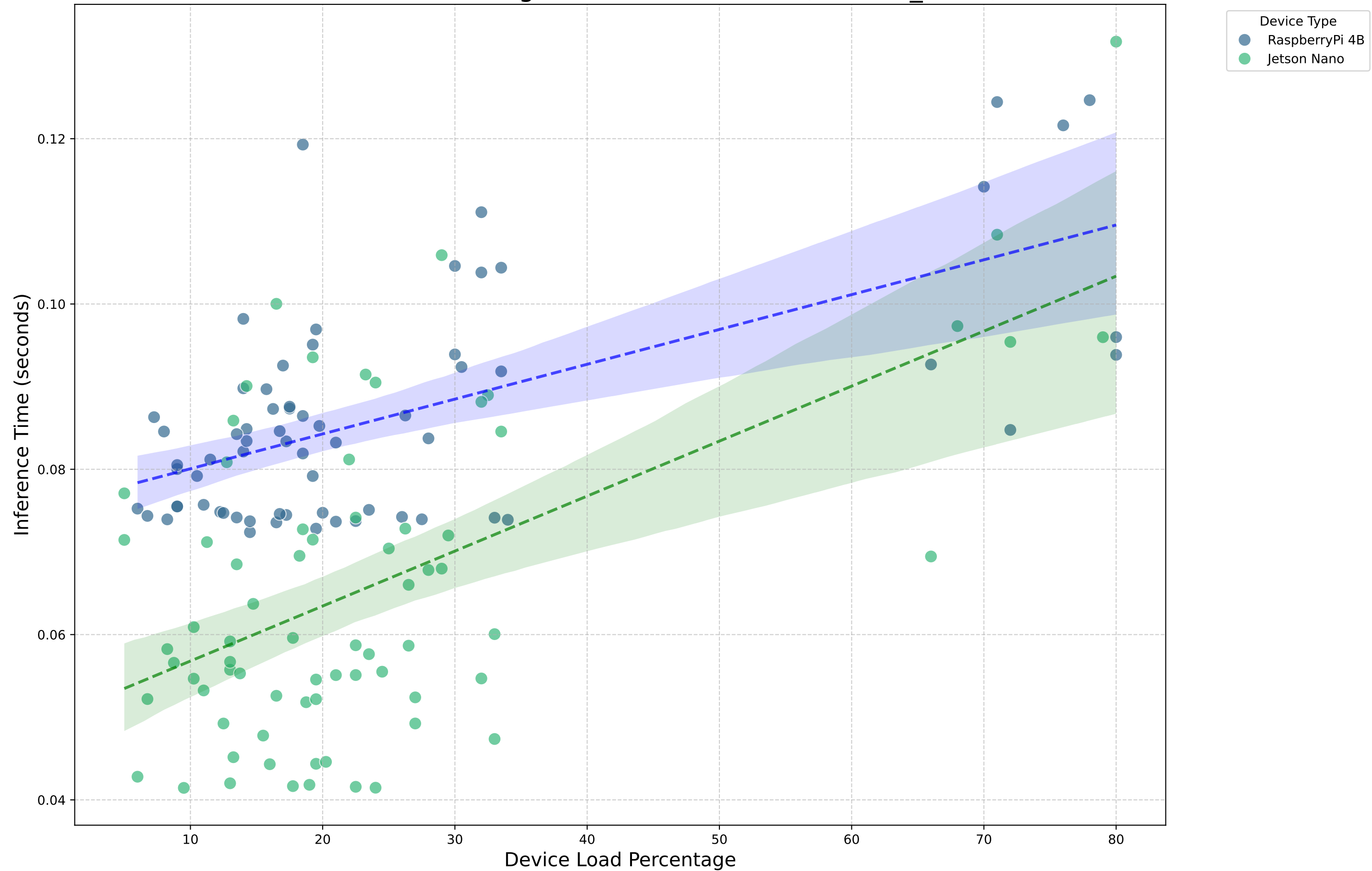
Device Load Percentage vs. Inference Time (Alexnet_Part2)
