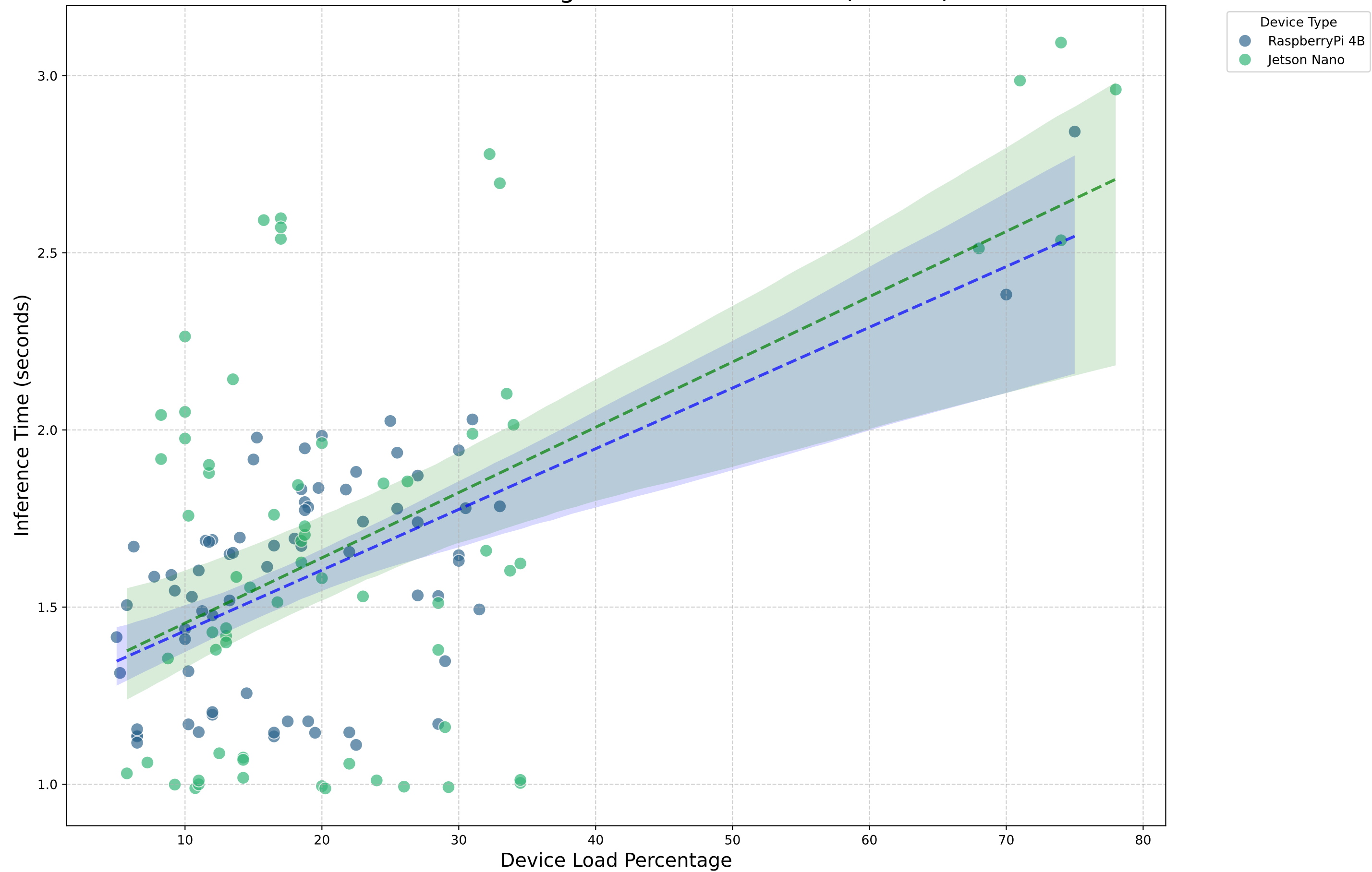
Device Load Percentage vs. Inference Time (Resnet)
