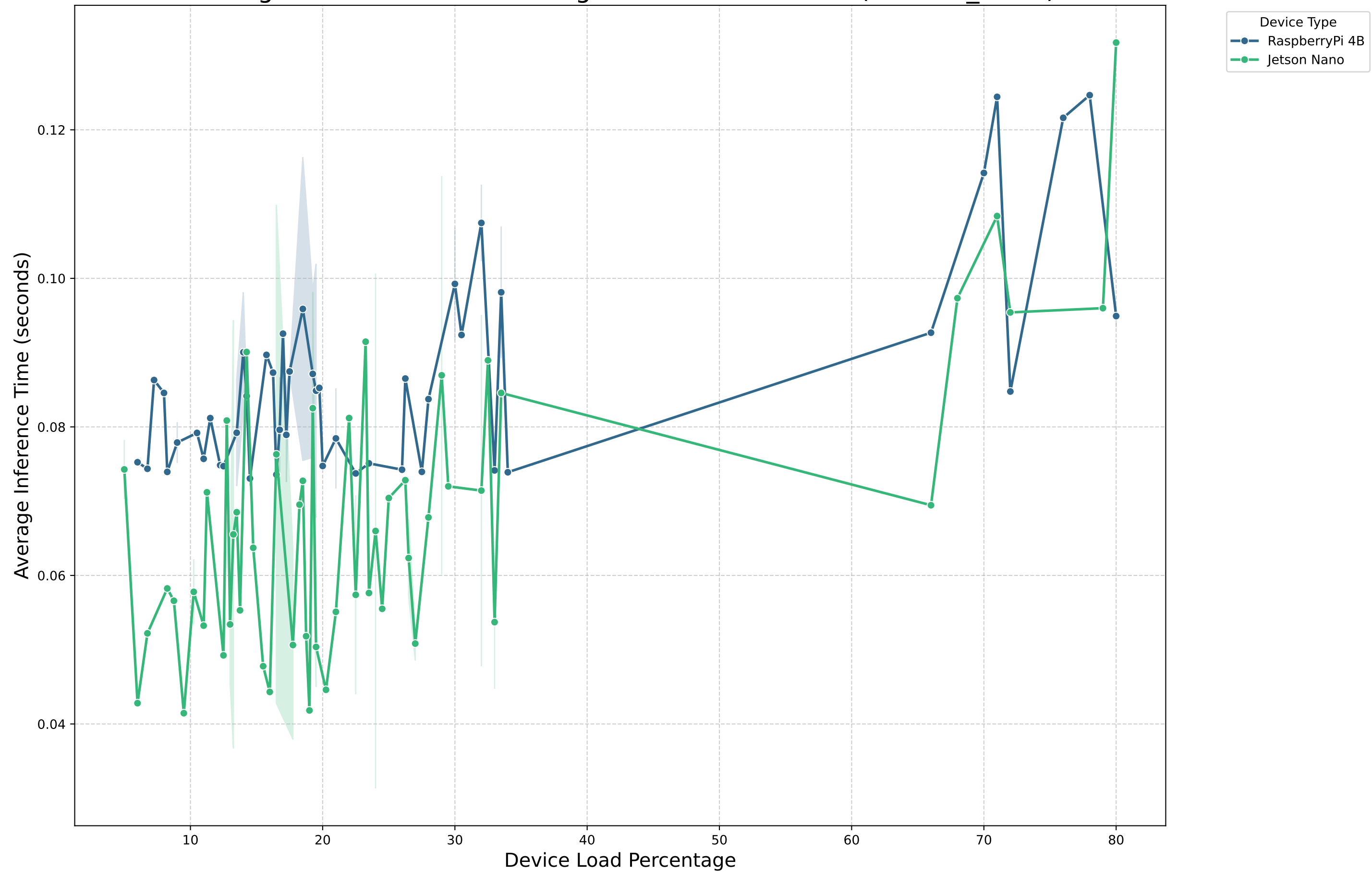
Average Device Load Percentage vs. Inference Time (Alexnet_Part2)
