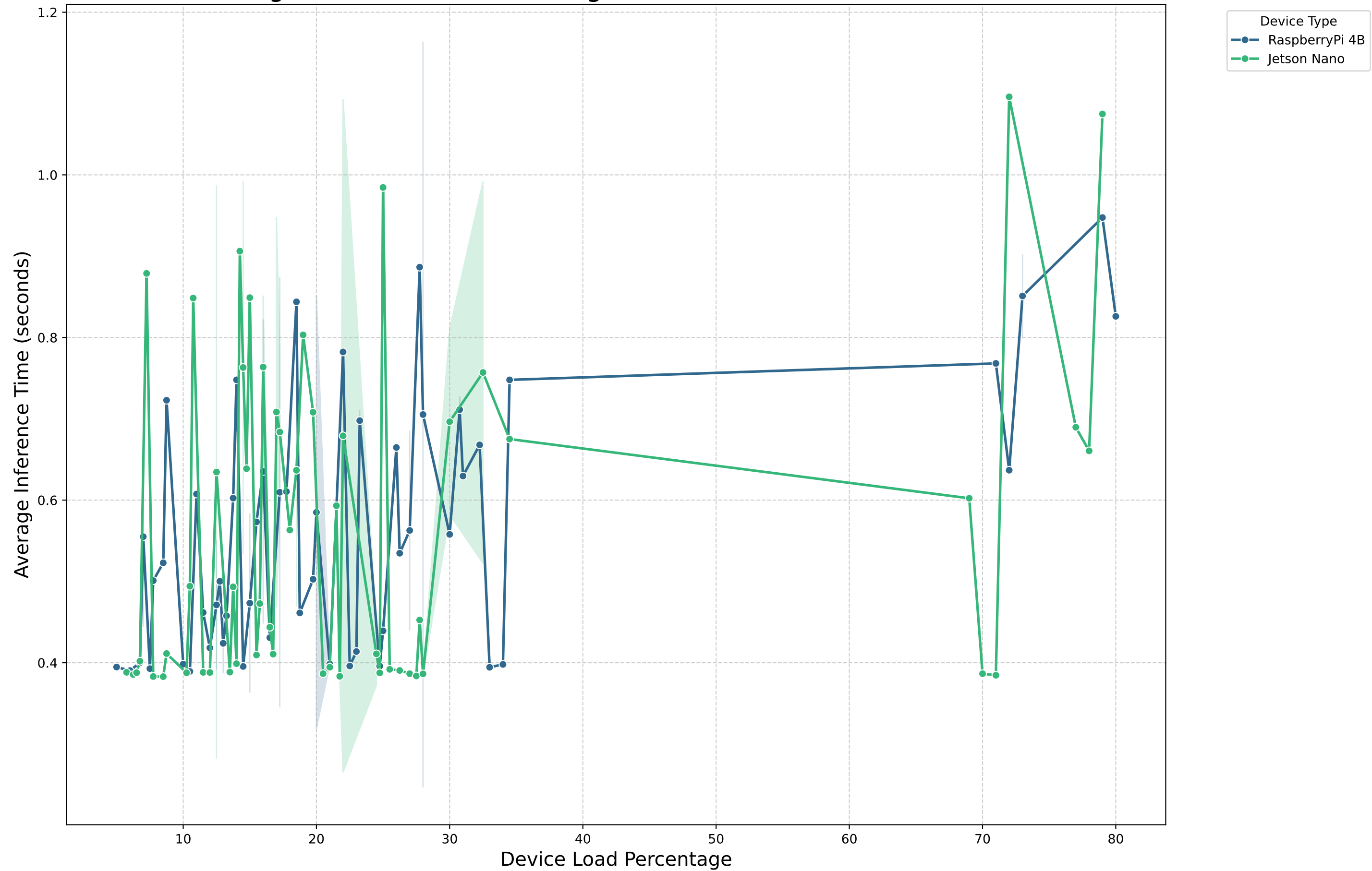
Average Device Load Percentage vs. Inference Time (Efficientnet)
