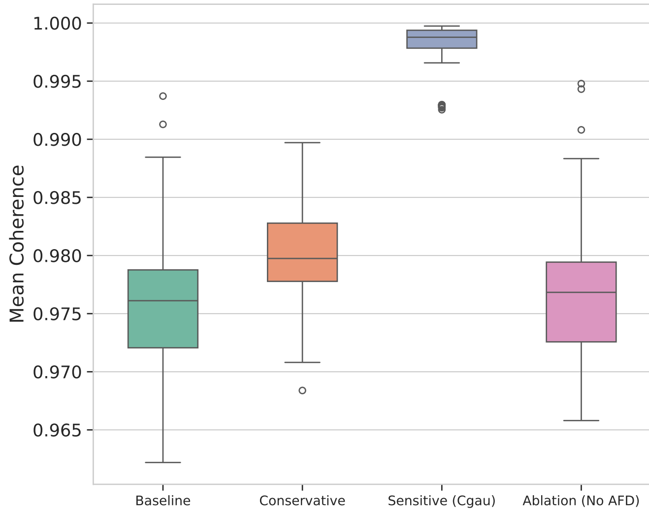
Distribution of Mean Coherence
