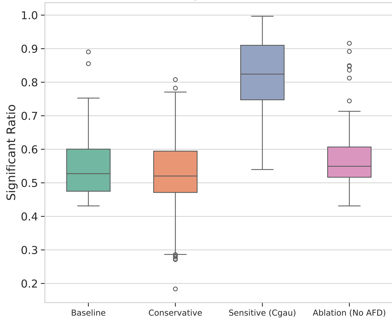
Distribution of Significant Coherence Ratio
