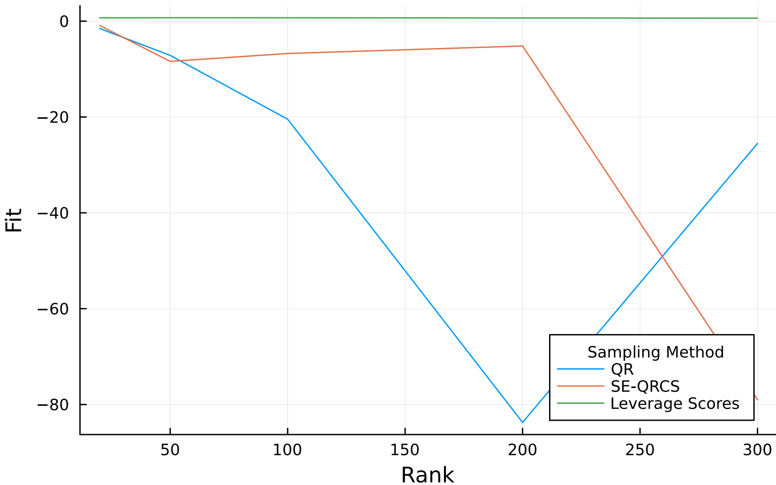
20 Image COIL data, 1000 Samples
