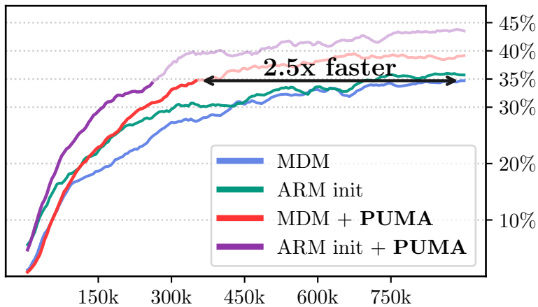
Training Iteration vs. GSM8K Accuracy
